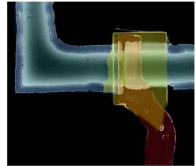
Figure 17. Gatemon qubit. Left: gatemon array. Right: closeup of the gatemon junction with an electrode to tune the static potential and change the tunnel barrier electrically. Reproduced with permission from [176].
