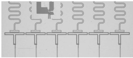
Figure 17. Gatemon qubit. Left: gatemon array. Right: closeup of the gatemon junction with an electrode to tune the static potential and change the tunnel barrier electrically. Reproduced with permission from [176].
