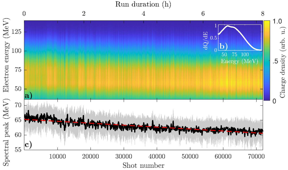
Figure 4.28: Electron energy as function of shot number and time. (a) waterfall plot, (b) average energy spectrum and (c) position of the peaks of Gaussian fits averaged over 100 shots at each position with their standard deviations shown as grey band
