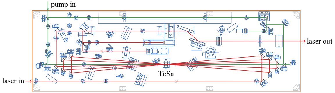
Figure 3.7: Layout of the second multi-pass amplifier stage. A pump laser (green) pumps the Ti:Sa crystal. The incoming laser (red) passes the pumped crystal five times. As no cavity mirrors are used, the intensity inside the crystal is the same intensity the pulse reaches after its final amplification. In addition, several diagnostics for pump and main laser as well as lenses are inside the amplifier.
