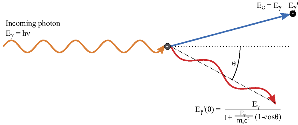
Figure 5.8: Illustration of Compton scattering. An incoming photon with an energy of E_\gamma = h\nu scatters on a quasi free electron from the absorber material, whereby the electron gains part of the energy of the incoming photon.
