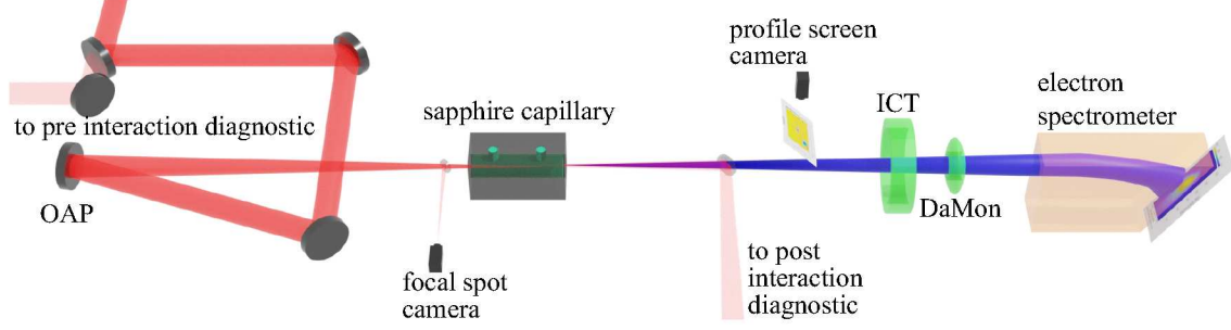
Figure 4.1: Schematic drawing of the setup for first self-injection experiments. The beam enters the main vacuum chamber and the leakage of the first mirror is sent to the pre-interaction diagnostics for alignment. The reflected part is sent to an f/14 off-axis parabola (OAP), which focussed the beam onto a sapphire capillary with a length of 15 mm and a diameter of 200 \mu\text{m} . To check the focus quality, a wedge could be driven into the focussed laser beam in front of the capillary, sending it into a focal-spot camera. The focal-spot quality was then optimised in vacuum using pico motors. Before the parabola, a pickoff mirror could be flipped into the beam to send the pulse to the pre-interaction diagnostics for pulse-duration measurements. The additional dispersion of the window was compensated using the Dazzler. After the capillary, the laser could be collected using a second wedge, was refocussed and sent to the post-interaction diagnostics for laser alignment, capillary alignment and spectral analysis of the laser beam. To characterise the electron beams, a profile screen and an electron spectrometer are available. Within the first few weeks after electron acceleration, the ICT and the DaMon, were added, which offered a non-invasive measurement of the bunch charge.
