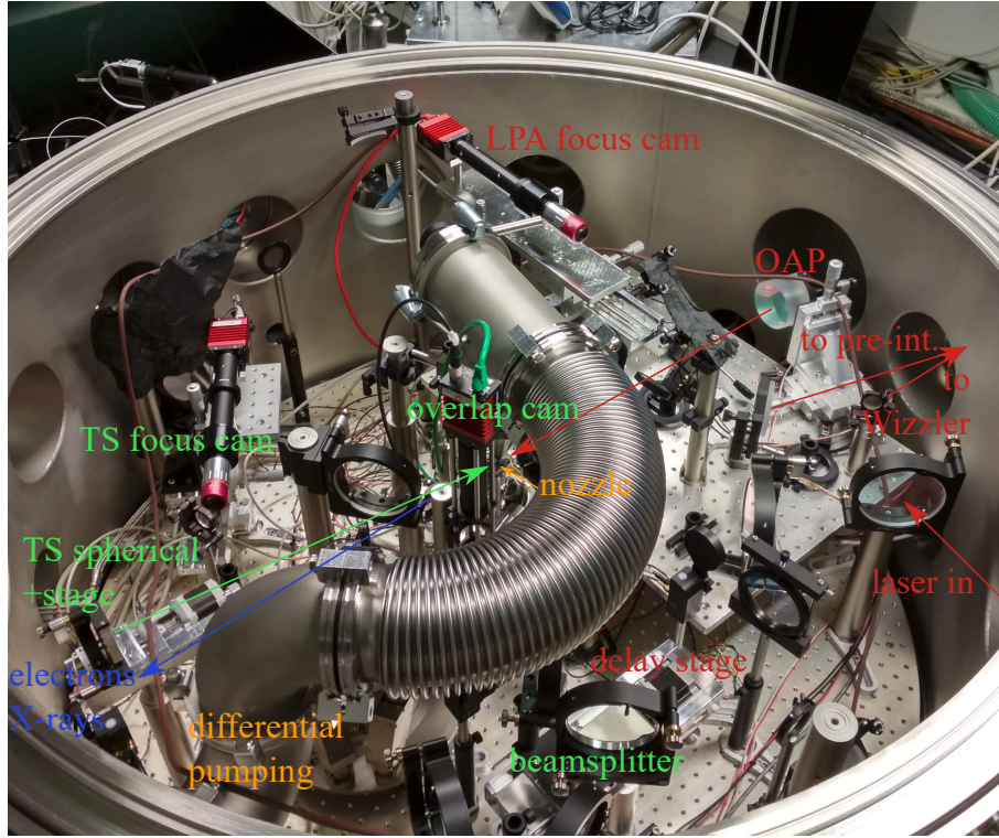
Figure 5.6: Image of the setup in the wakefield chamber for the Thomson experiments.
