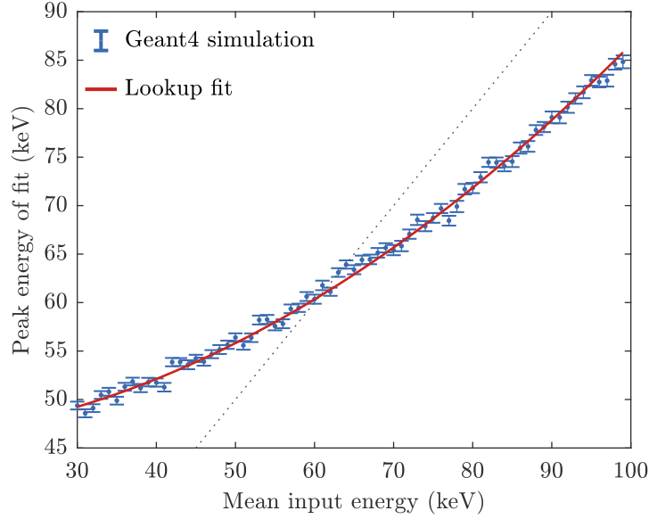
Figure 5.15: Peak position of the mean Gaussian fit as a function of the mean input energy from a Geant4 simulations with central beam energies of 30 keV to 100 keV [186]. In addition, a quadratic fit is shown that is used for the calculation of the peak energy from measured input spectra. The grey dotted line corresponds to a ratio of 1.
