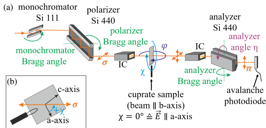
Fig. 1. (a) Sample was mounted on a Eulerian cradle with the b axis parallel to the linearly polarized beam ( \sigma -polarization in the horizontal plane). An avalanche photodiode behind the x-ray analyzer in crossed position to the polarizer detected the \sigma \rightarrow \pi scattered photons. Simultaneously, ionization chambers (IC) measured the transmitted intensity through the sample. (b) Enlarged view of the sample as seen from the direction of the incoming beam.
