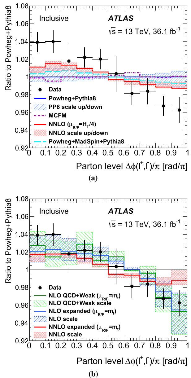
Fig. 14 Comparison of the unfolded \Delta\phi distribution with theoretical predictions for the inclusive selection: ratio as compared with POWHEG + PYTHIA 8 for a NLO generators and NNLO fixed-order predictions, b NLO and NNLO theoretical predictions expanded in the normalised cross-section ratio. Each prediction is discussed in the text
