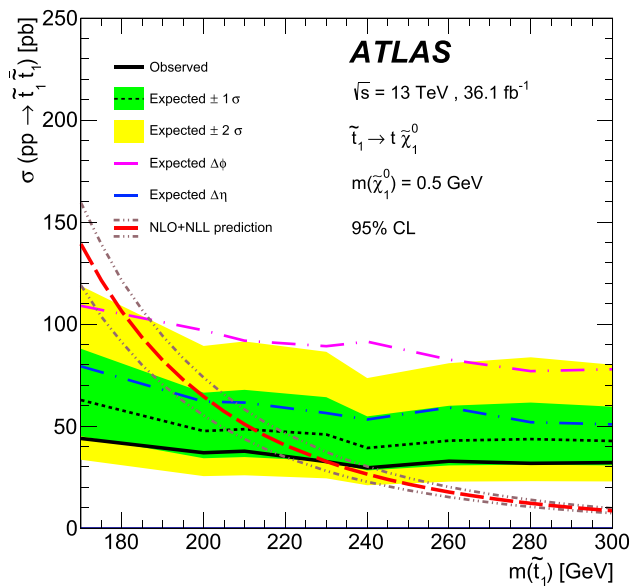
Fig. 16 Expected and observed limits at 95% CL on the top squark pair production cross-section as a function of m_{\tilde{t}_1} assuming a 100% branching ratio for \tilde{t}_1 \rightarrow t \tilde{\chi}_1^0 decays with m_{\tilde{\chi}_1^0} = 0.5 GeV. The dashed line shows the expected limit with \pm 1 and \pm 2 standard deviation bands. The dashed line shows the theoretical cross-section with uncertainties. The solid line gives the observed limit. Also shown are the expected limits using the \Delta\phi and \Delta\eta distributions separately
