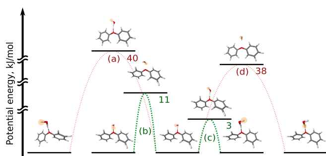
Figure 8: Scheme for motions in the OH-O DPE-(H 2 O) isomer that interconnect equivalent minima on the PES. This scheme contains a set of five equivalent minima and the transition states that lead from the central minimum to others. The letters in parentheses denote the motion (see text for details), numbers denote the transition state energies in kJ/mol computed at the DLPNO-CCSD(T)/def2-TZVPP//B97-3c level of theory. The yellow highlighting and its absence indicate the positions of the unique protons.
