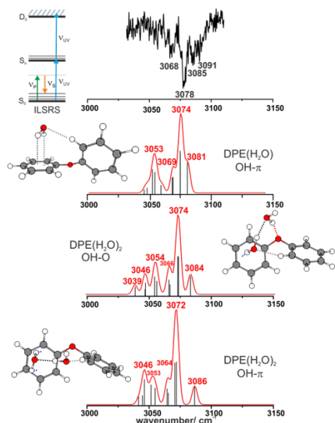
Figure 4: ILSR spectrum of the CH stretching region (top trace) of DPE/water aggregates recorded on the mass channel of DPE-(H 2 O) (carrier gas helium). Quantum-chemical calculations (DFT/B3LYP-D3(BJ)/def2-TZVP level) refer to DPE-(H 2 O) (OH- \pi arrangement), DPE-(H 2 O) 2 (OH-O arrangement), and also the DPE-(H 2 O) 2 cluster (OH- \pi arrangement), which can fragment on the DPE-(H 2 O) mass channel (scaling factor 0.96).
