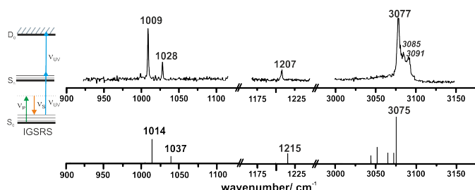
Figure 3: The top trace shows the experimental IGSR spectrum of DPE in helium. The bottom trace results from a quantum-chemical calculation (DFT/B3LYP-D3(BJ)/def2-TZVP). With respect to this functional and basis set, the typical scaling factors for the CH bending / C-O stretching region (0.99) and the CH stretching region (0.96) are chosen.
