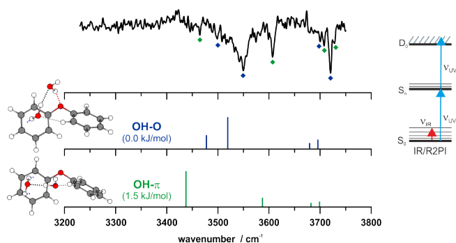
Figure 5: IR/R2PI spectrum of DPE-(H 2 O) 2 via the UV excitation energy of 35907 cm -1 using the carrier gas neon, compared to calculated vibrational frequencies for the two most stable clusters calculated at the B3LYP-D3(BJ)/def2-TZVP level. Scaling factor 0.96 (see also Figure S9).
