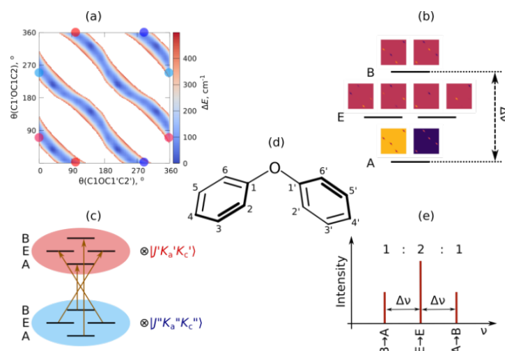
Figure 1: Theoretical analysis of the internal dynamics of the DPE monomer (see text for more details). (a) PES interpolated from a DLPNO(TightPNO)-CCSD(T)/def2-TZVPP//B3LYP-D3(BJ)/def2-TZVPP rigid scan for the two dihedral angles. The white areas correspond to energies above 400\text{ cm}^{-1} . (b) Splitting scheme with respect to the C_4 molecular symmetry group and the wavefunctions corresponding to the energy levels. The estimated splittings \Delta v are 3 kHz when using the B3LYP-D3 PES and 50 kHz for the DLPNO-CCSD(T) PES. (c) Rotational transition scheme caused by the \mu_b dipole-moment component that corresponds to the irreducible representation B of C_4 , (d) scheme of the molecular structure of DPE including labelling of the carbon atoms, and (e) sketch of the predicted theoretical splitting of a particular rotational transition in the rotational spectrum.
