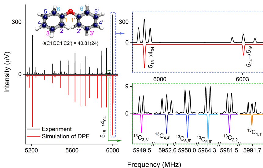
Figure 2: Parts of the rotational spectrum of the DPE monomer, where the zoom-ins highlight the characteristic triplet splitting pattern of DPE in both R and Q branches due to internal motions of the two phenyl groups (upper right blue box), and the triplet (C1,1' and C4,4') and doublet (C2,2', C3,3', C5,5' and C6,6') splitting patterns observed in the singly substituted ^{13}\text{C} isotopologues in natural abundance due to the same motions, presented here for the J'_{\text{Ka}',\text{Kc}} \leftarrow J_{\text{KaKc}} = 5_{15} \leftarrow 4_{04} rotational transition of DPE (lower right green box). In all spectra, the top, black trace shows the experimental spectrum, and the bottom traces give the simulated spectra based on the assigned rotational constants of DPE (red) and its ^{13}\text{C} isotopologues (multi-color). The experimental structure of the DPE monomer ( r_m^{(1)} fit, blue spheres) is also shown (top left, see also Figure S4), in comparison to the underlying grey structure computed at the B3LYP-D3(BJ)/def2-TZVP level of theory.
