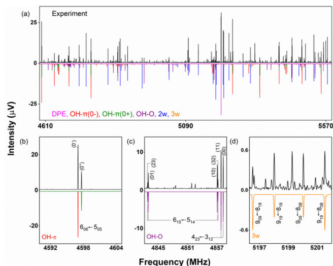
Figure 6: (a) A section of the 2–8 GHz rotational spectrum of DPE–H 2 O (5 million acquisitions). The upper experimental trace in black is compared with simulations based on fitted parameters for DPE and its complexes with one water (OH- \pi and OH-O isomers), two water (2w) and three water (3w) molecules. (b) Parts of the spectrum showing the tunneling splittings for the OH- \pi isomer indicated with 0 - (red) and 0 + (green), (c) the tunneling fine structure in the OH-O complex (see text), and (d) rotational transitions for the 3w complex. The other, low-intensity transitions do not correspond to any species we could identify so far.
