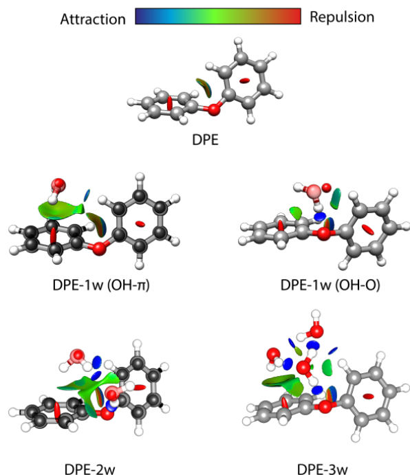
Figure 7: Non-covalent interaction (NCI) analysis for DPE and its experimentally observed complexes with one water (OH- \pi and OH-O isomers), two water (2w, OH-O structure, compare Figure 4), and three water (3w) molecules. The structures of DPE-1w and DPE-2w are made transparent to show the experimental atom positions of carbon and oxygen determined from the r_0 fit (for DPE-1w OH- \pi ) and the r_s structure (for DPE-1w OH-O and DPE-2w). Blue and green colors identify the presence of hydrogen bonding (strong attraction, blue) and van der Waals interactions (weak attraction, green). Red indicates repulsive interactions.
