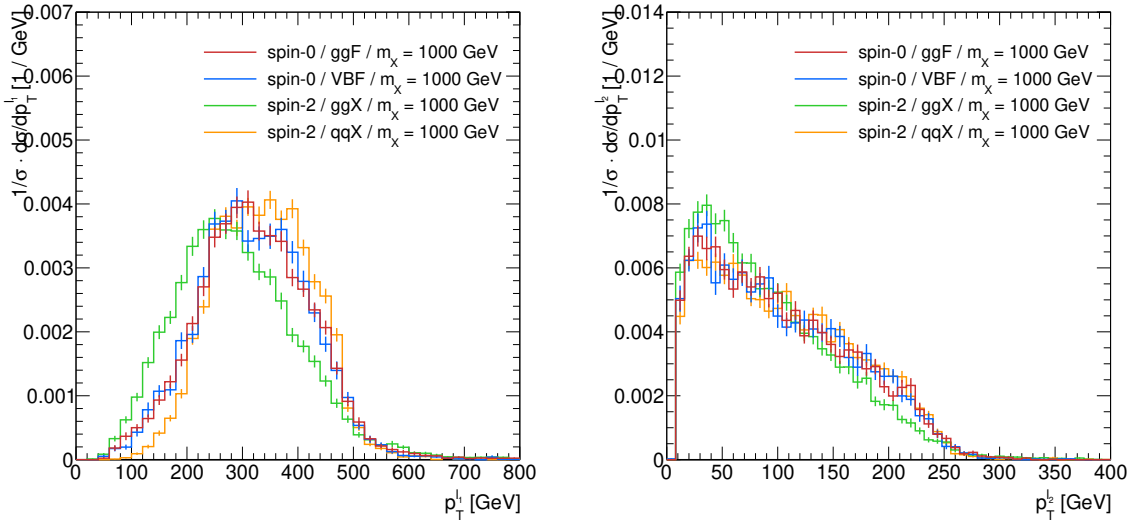
Figure B.4.: Normalised p_T distributions of the leading and sub-leading leptons for the ggF and VBF production of a spin-0 resonance and the gluon-induced and quark-induced production modes of a spin-2 resonance with a mass of m_X = 1 TeV as derived from Monte Carlo simulations after the common preselection stage.
