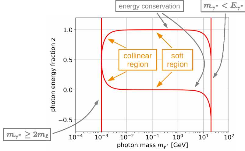
Figure 14.6.: Kinematic boundaries and regimes for electrons from the decay of a virtual photon with E_{\gamma^*} = 20 GeV.
