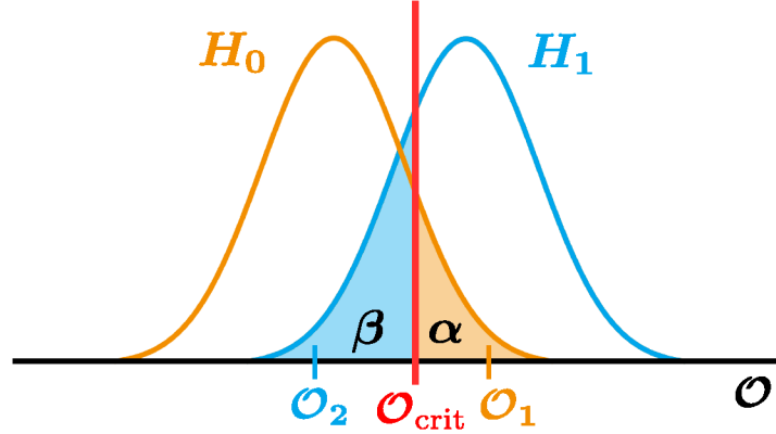
Figure 6.1.: Sketch of the type-1 and type-2 errors of hypothesis testing. The type-1 error describes the probability of falsely rejecting the true null hypothesis H_0 , while the type-2 error gives the probability of falsely accepting the false null hypothesis. In the frequentist approach, the decision to accept or reject the null hypothesis is made by comparing the observed value to a critical value \mathcal{O}_{\text{crit}} which is derived from the desired level of confidence 1 - \alpha .
