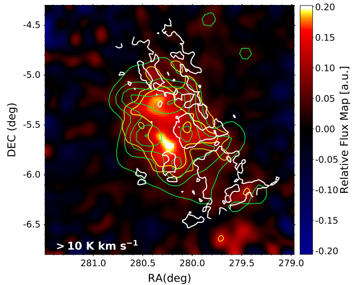
Figure 8. LE skymap, similar to Fig. 1. The source as seen by MAGIC is shown as yellow contours, while the Fermi -LAT source is plotted as green contours. The CO contours are shown with white solid lines when CO map is integrated over the range of -5 \text{ km/s} to 135 \text{ km/s} . The CO data is obtained from archival Galactic Ring Survey (GRS; Jackson et al. 2006).
