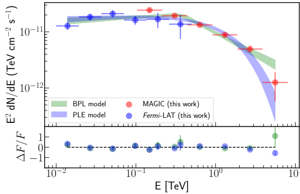
Figure 2. The spectral energy distribution (SED) of the extended source HESS J1841-055. The MAGIC energy fluxes are shown for energy above 100 GeV (red) whereas Fermi -LAT energy fluxes are obtained for energy above 10 GeV (blue). The combined fit of the Fermi -LAT and MAGIC SEDs is best described by either a BPL model (green shaded region) or a PLE (blue shaded region) model.
