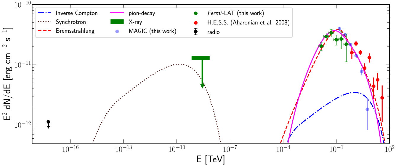
Figure 6. SED of HESS J1841-055 from radio to TeV energies. HE Fermi -LAT data (green points) and TeV MAGIC (blue points) and H.E.S.S. (red points) data are fitted both with hadronic (magenta solid line) and bremsstrahlung (red dashed line) models. Inverse Compton (blue dot-dashed line) can not account for the measured gamma-ray emission. The synchrotron spectrum (brown dotted line) is fitted according to the radio and X-ray ULs.
