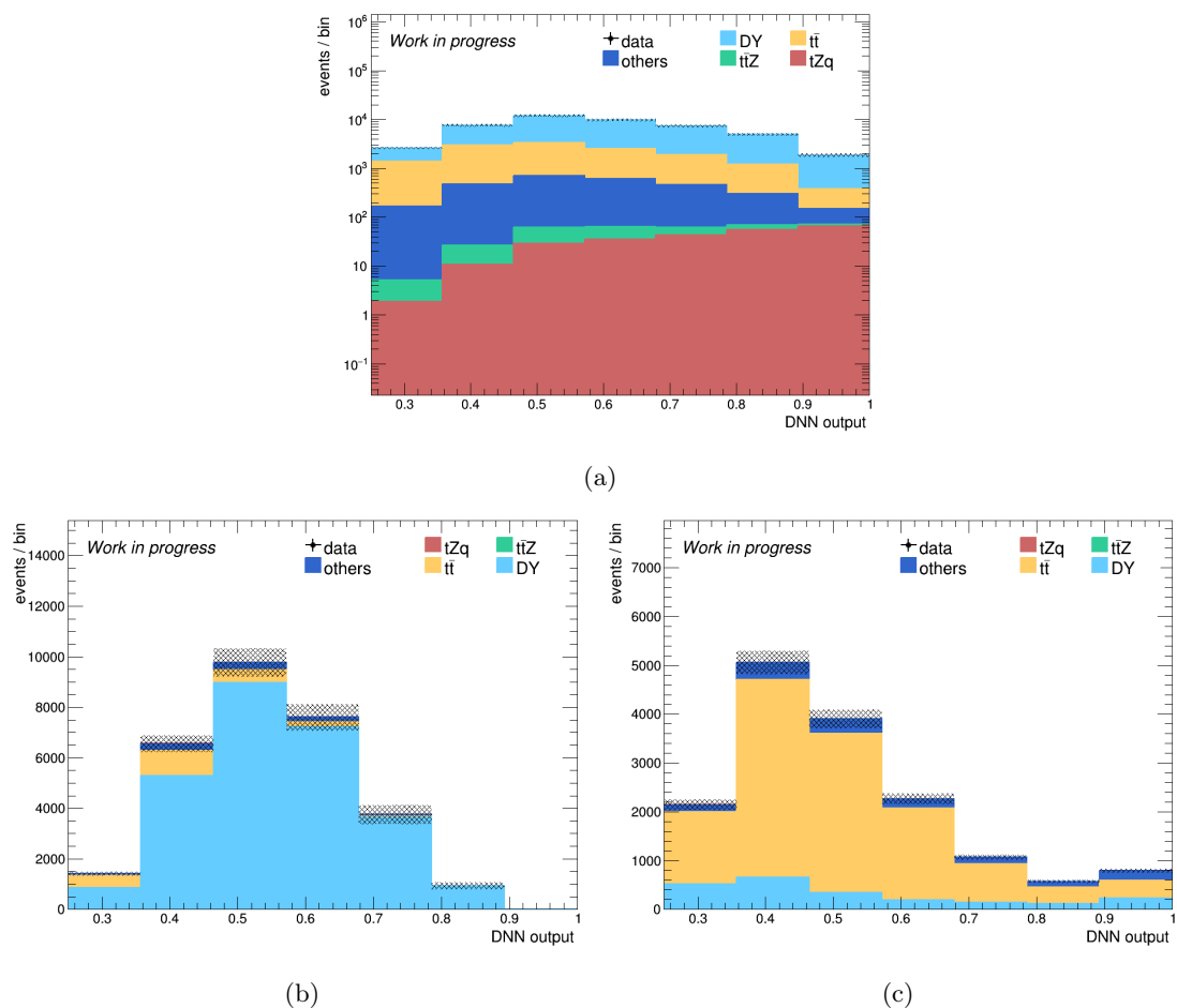
Figure 4.10: Pre-fit distributions for the three categories, corresponding to (a) tZq , (b) DY and (c) t\bar{t} output nodes. Statistical and systematic uncertainties are shown at the top of each histogram.
