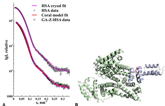
Fig 6. (a) HSA and GA-Z-HSA experimental data is shown as white circles and white squares, respectively. The corresponding fit to the HSA experimental data using CRYSOLOG and an X-ray crystallography model with PDB ID: 1TF0 is shown with a magenta line. For fitting to the GA-Z-HSA experimental we show both the CRYSOLOG fit (magenta line) using only HSA PDB ID: 1TF0 as well as that from the CORAL rigid body model (red line), for comparison. (b) The resulting rigid body model from CORAL is shown in a ribbon representation with HSA in green and GA-Z in blue, the linker between the GA and Z-domains is shown in magenta. GA-Z is bound to the HSA DII domain.
