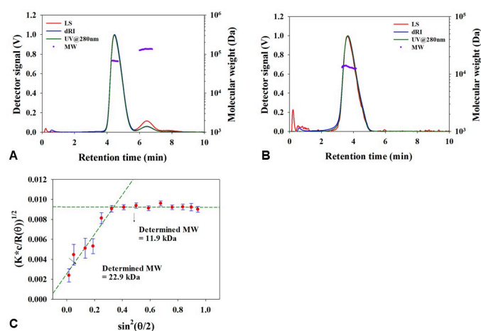
Fig 1. AF4 fractograms and molecular weight (MW) of (a) HSA, (b), GA-Z and (c) Berry plot of GA-Z in 25 mM phosphate buffer at pH 7.
