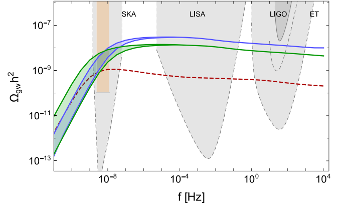
Fig. 2. Gravitational wave spectra from metastable cosmic strings explaining the NANOGrav excess (at 2\sigma CL). The colored blue (green) region accounts for successful inflation, leptogenesis and dark matter [22,24] for the maximal (minimal) allowed value of G\mu with \sqrt{\kappa} = 8.0 \dots 8.1 (8.1.8.3), corresponding to the \star ( \diamond ) markers in Fig. 1. For reference, the dashed red line shows the spectrum for stable cosmic strings for the best-fit value G\mu = 10^{-10} [15,16], this curve is degenerate with the corresponding curve with \sqrt{\kappa} = 9 . The (lighter) gray-shaded areas indicate the sensitivities of the (planned) experiments SKA [37], LISA [38], LIGO/Virgo [35] and ET [39]. The orange band indicates the frequency range of NANOGrav.
