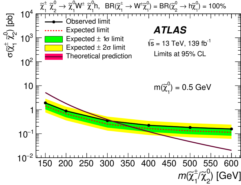
Figure 9. Expected and observed 95% CL exclusion upper limits on the production cross-section of \tilde{\chi}_1^\pm \tilde{\chi}_2^0 \rightarrow W^\pm \tilde{\chi}_1^0 h \tilde{\chi}_1^\pm as a function of m(\tilde{\chi}_1^\pm/\tilde{\chi}_2^0) .
