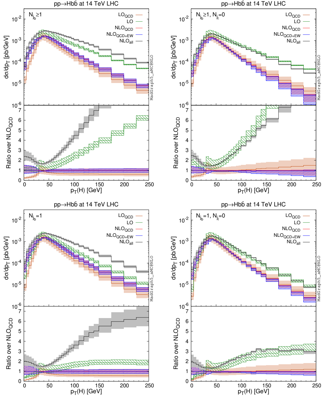
Figure 5. The p_T(H) distribution for N_b \geq 1 (up) and N_b = 1 (down). In the right plots the light-jet veto is applied.
