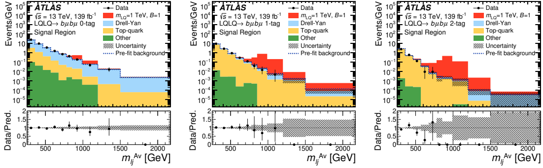
Figure 7. Post-fit distributions of m_{\ell j}^{Av} in the b\mu signal regions: 0-tag (left), 1-tag (middle), and 2-tag (right). The expected signals, shown for m_{LQ} = 1 TeV and \mathcal{B}(LQ \rightarrow b\mu) = 1 , are shown for illustrative purposes. The category ‘Top-quark’ refers to t\bar{t} and single-top-quark processes. The category ‘Other’ refers to diboson and W +jet production. The hatched band represents the total uncertainty in the background predictions.
