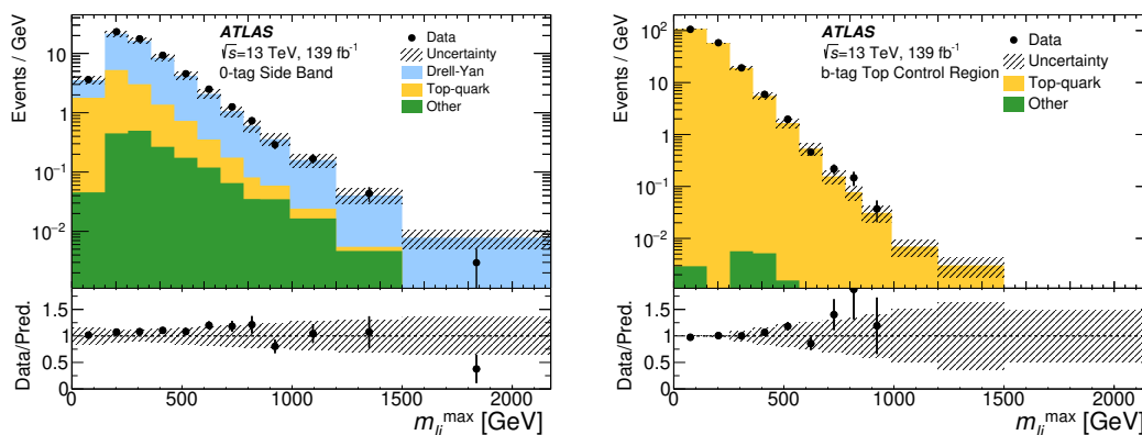
Figure 2. Distributions of m_{\ell j}^{\max} in the combined be and b\mu 0-tag SB for the b\ell channels (left) and the b -tag Top CR for the c\ell channels (right). The total modelling uncertainty combined with the MC statistical error is shown as the hatched band as explained in section 7. The category ‘Other’ represents the sum of all SM background contributions except those from top-quark processes ( t\bar{t} and single-top) and, for the 0-tag SB distribution, Drell-Yan processes.
