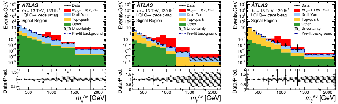
Figure 4. Post-fit distributions of m_{\ell j}^{Av} in the ce signal regions: untagged (left), c -tag (middle), and b -tag (right). The expected signals, shown for m_{LQ} = 1 TeV and \mathcal{B}(LQ \rightarrow ce) = 1 , are shown for illustrative purposes. The category ‘Top-quark’ refers to t\bar{t} and single-top-quark processes. The category ‘Other’ refers to diboson and W +jet production. The hatched band represents the total uncertainty in the background predictions.
