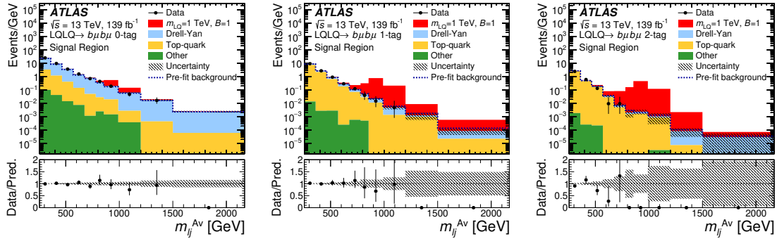
Figure 7. Post-fit distributions of m_{l_j}^{Av} in the b\mu signal regions: 0-tag (left), 1-tag (middle), and 2-tag (right). The expected signals, shown for m_{LQ} = 1 TeV and \mathcal{B}(LQ \rightarrow b\mu) = 1 , are shown for illustrative purposes. The category ‘Top-quark’ refers to t\bar{t} and single-top-quark processes. The category ‘Other’ refers to diboson and W +jet production. The hatched band represents the total uncertainty in the background predictions.
