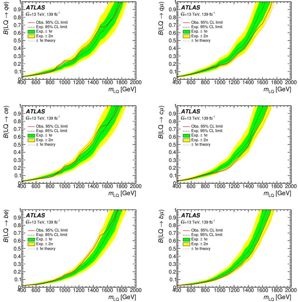
Figure 9. The observed (solid line) and expected (dashed line) limits on the leptoquark branching ratio \mathcal{B} into a quark and an electron or a muon at 95% CL, shown as a function of m_{\text{LQ}} for the different leptoquark channels. The green and yellow bands show the \pm 1\sigma and \pm 2\sigma ranges of the expected limit. The error band on the observed curve (dotted lines) represents the uncertainty in the theoretical cross-section from PDFs, renormalisation and factorisation scales, and the strong coupling constant \alpha_s .
