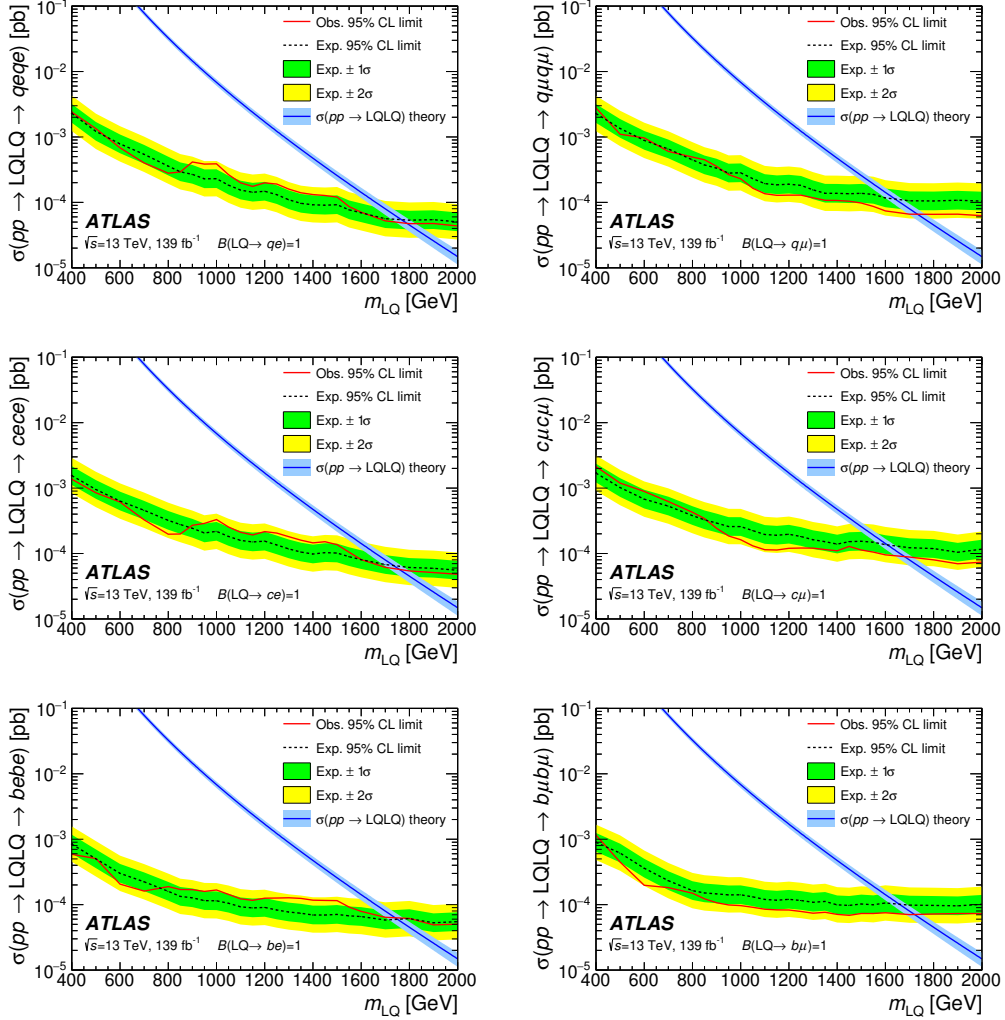
Figure 8. The observed (solid line) and expected (dashed line) limits on the leptoquark pair production cross-section at 95% CL for \mathcal{B} = 1 into electrons or muons, shown as a function of m_{LQ} for the different leptoquark channels. The green and yellow bands show the \pm 1\sigma and \pm 2\sigma ranges of the expected limit. Also included on the plots is the expected theoretical cross-section. The thickness of the theory curve represents the theoretical uncertainty from PDFs, renormalisation and factorisation scales, and the strong coupling constant \alpha_s .
