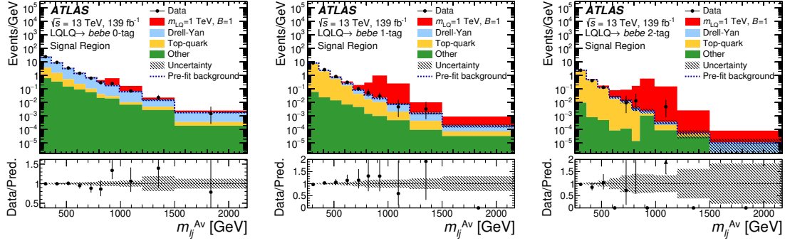
Figure 6. Post-fit distributions of m_{l_j}^{Av} in the be signal regions: 0-tag (left), 1-tag (middle), and 2-tag (right). The expected signals, shown for m_{LQ} = 1 TeV and \mathcal{B}(LQ \rightarrow be) = 1 , are shown for illustrative purposes. The category ‘Top-quark’ refers to t\bar{t} and single-top-quark processes. The category ‘Other’ refers to diboson and W +jet production. The hatched band represents the total uncertainty in the background predictions.
