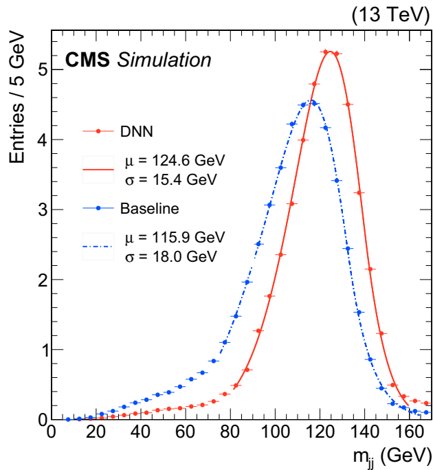
Fig. 5 Dijet invariant mass distributions for simulated samples of Z(\rightarrow \ell^+ \ell^-)H(\rightarrow b\bar{b}) events, where two jets and two leptons were selected. Distributions are shown before (dotted blue) and after (solid red) applying the b jet energy corrections. A Bukin function [44] was used to fit the distribution. The fitted mean and width of the core of each distribution are displayed in the figure
