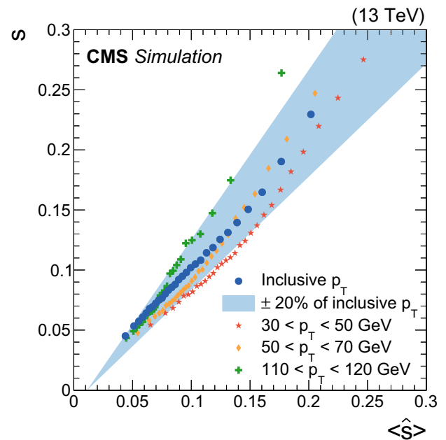
Fig. 4 Correlation between jet energy resolution s and the average jet energy resolution estimator \langle s \rangle for b jets from t\bar{t} MC events. The blue circles correspond to the inclusive p_T spectrum, while the blue band represents 20% up and down variations of the fitted \langle s \rangle trend for the inclusive p_T spectrum. The red stars correspond to jets with p_T \in [30, 50] GeV, orange diamonds to p_T \in [50, 70] GeV, and green crosses to p_T \in [110, 120] GeV
