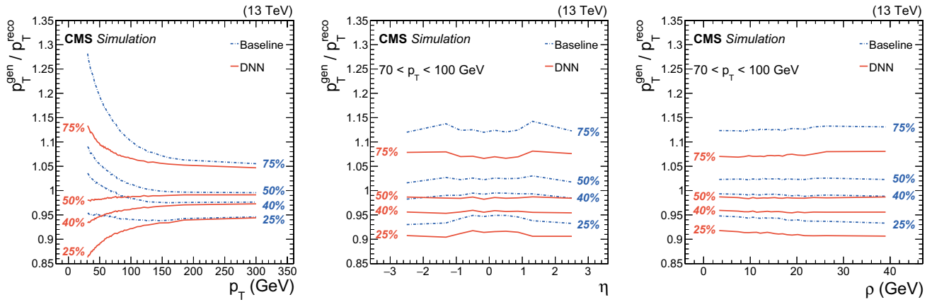
Fig. 2 The 25, 40, 50, and 75% quantiles are shown for the b jet energy scale p_T^{\text{gen}}/p_T^{\text{reco}} distribution before (blue dashdot) and after (red solid) applying the regression correction as a function of jet p_T
