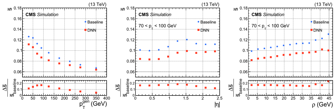
Fig. 3 Relative jet energy resolution, \bar{s} , as a function of generator-level jet p_T^{\text{gen}} (left), \eta (center), and \rho (right) for b jets from t\bar{t} MC events. The average p_T of these b jets is 80 GeV. The \eta and \rho distributions are shown for jets with p_T \in [70, 100] GeV. The blue stars and
