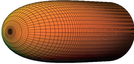
Figure 2: Visualization of the 2D manifold with metric (1.2).
