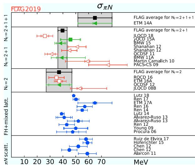
Fig. 44 Lattice results and FLAG averages for the nucleon sigma term, \sigma_{\pi N} , for the N_f = 2, 2 + 1 , and 2 + 1 + 1 flavour calculations. Determinations via the direct approach are indicated by squares and the Feynman-Hellmann method by triangles. Results from calculations which analyse more than one lattice data set within the Feynman-Hellmann approach [454, 455, 949, 954–960] are shown for comparison (pentagons) along with those from recent analyses of \pi - N scattering [940–942, 961] (circles)
