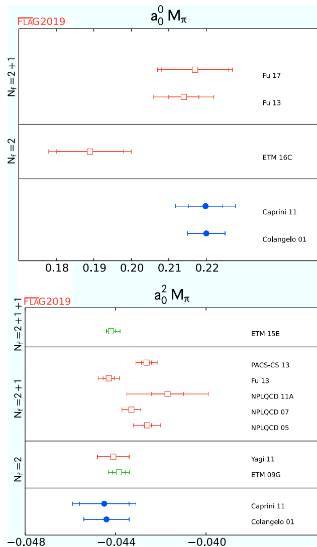
Fig. 16 Summary of the \pi\text{-}\pi scattering lengths a_0^0 M_\pi (top) and a_0^2 M_\pi (bottom)
