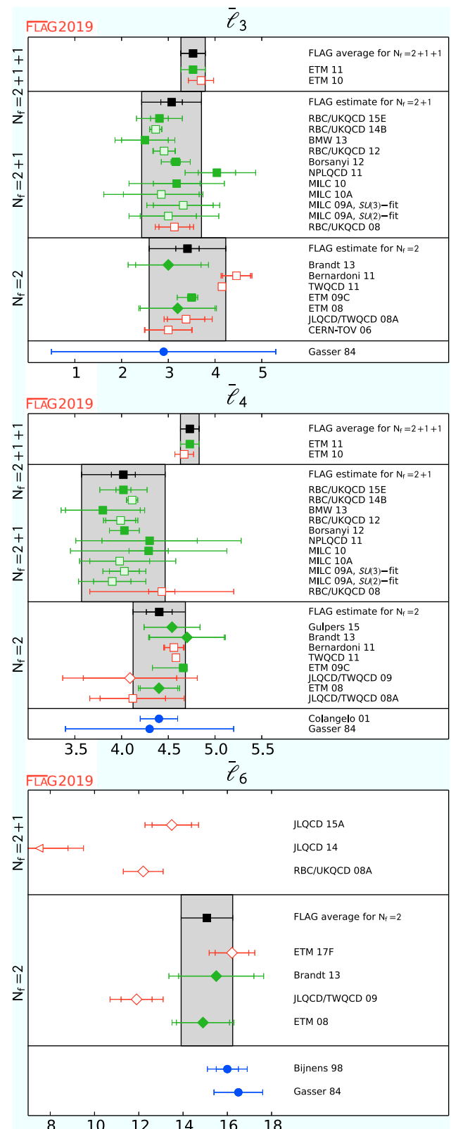
Fig. 14 Effective coupling constants \bar{l}_3 , \bar{l}_4 and \bar{l}_6 . Squares indicate determinations from correlators in the p -regime, diamonds refer to determinations from the pion form factor
