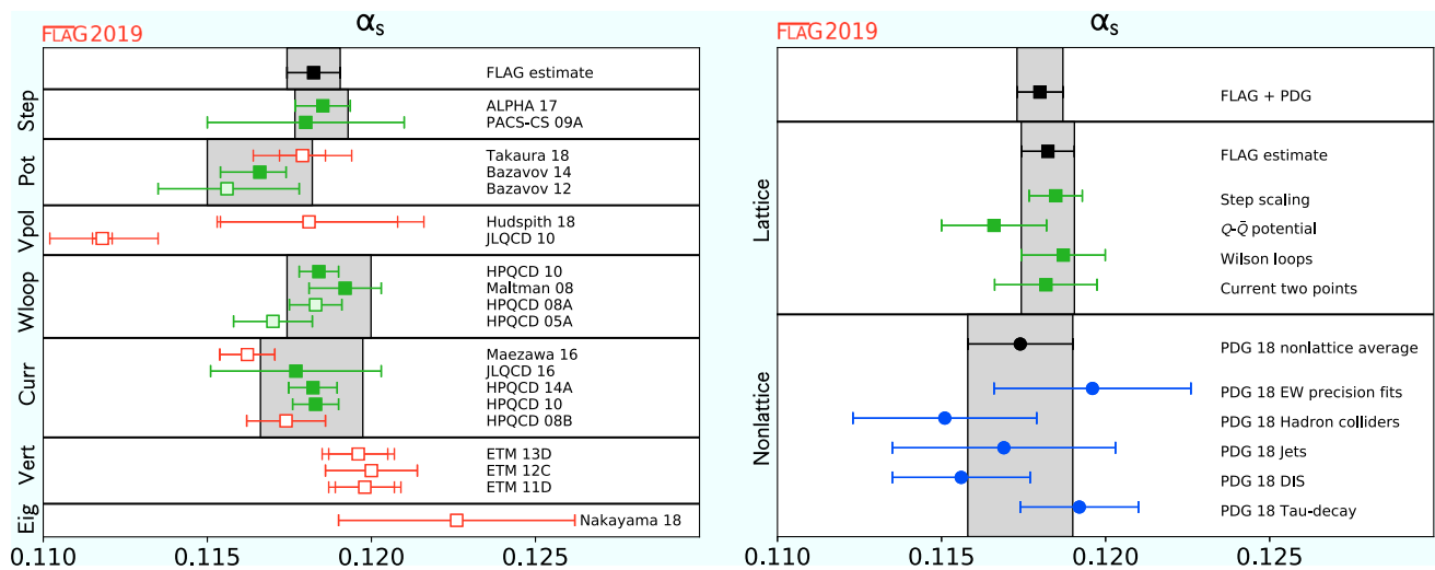
Fig. 38 \alpha_{\overline{\text{MS}}}^{(5)}(M_Z) , the coupling constant in the \overline{\text{MS}} scheme at the Z mass. Left: Lattice results, pre-ranges from different calculation methods, and final average. Right: Comparison of the lattice pre-ranges
