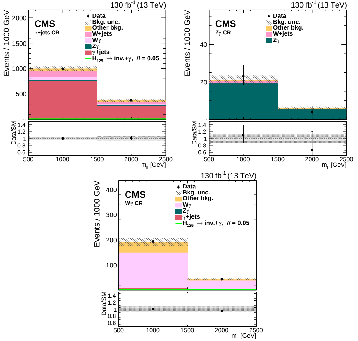
Figure 2: The m_{jj} distributions from the simultaneous fit in the \gamma + \text{jets} (upper left), Z(\ell\bar{\ell}) + \gamma (upper right), and W(\ell\nu) + \gamma (lower) CRs. The category other background includes contributions from Z + jets, nonprompt, top quark, VV, and VVV processes. Overflow events are included in the last bin. The shaded bands represent the combination of the statistical and systematic uncertainties in the predicted yields. The light green line, illustrating the possible contribution expected from inclusive SM Higgs boson production, assumes a branching fraction of 5% for H \rightarrow \text{inv.} + \gamma decays. The lower panel in the figures shows a per-bin ratio of the data yield and the background expectation. The shaded band corresponds to the combined systematic and statistical uncertainty in the background expectation.
