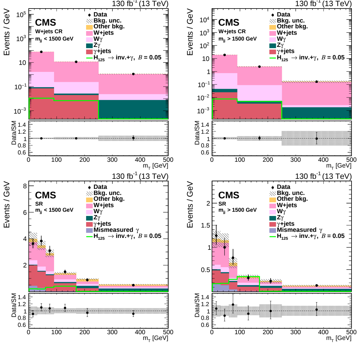
Figure 3: The m_T distributions from the simultaneous fit for events with m_{jj} < 1500 GeV in the W(\text{ev}) + \text{jets} CRs (upper left), for events with m_{jj} \geq 1500 GeV in the W(\text{ev}) + \text{jets} CRs (upper right), for events with m_{jj} < 1500 GeV in the SRs (lower left), and for events with m_{jj} \geq 1500 GeV in the SRs (lower right). The category other background includes contributions from Z + \text{jets} , nonprompt, top quark, VV , and VVV processes. Overflow events are included in the last bin. The shaded bands represent the combination of the statistical and systematic uncertainties in the predicted yields. The light green line, illustrating the possible contribution expected from inclusive SM Higgs boson production, assumes a branching fraction of 5% for H \rightarrow \text{inv.} + \gamma decays. The lower panel in the figures shows a per-bin ratio of the data yield and the background expectation. The shaded band corresponds to the combined systematic and statistical uncertainty in the background expectation.
