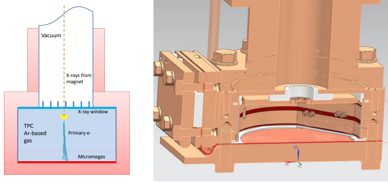
Figure 31. Left: Scheme of the detection principle of Micromegas detectors. Right: Design of the BabyIAXO detector prototype.
