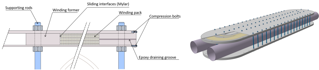
Figure 9. Left: layout of the cold mass mechanical design. Right: 3D artistic view of the cold mass (not showing all details).
