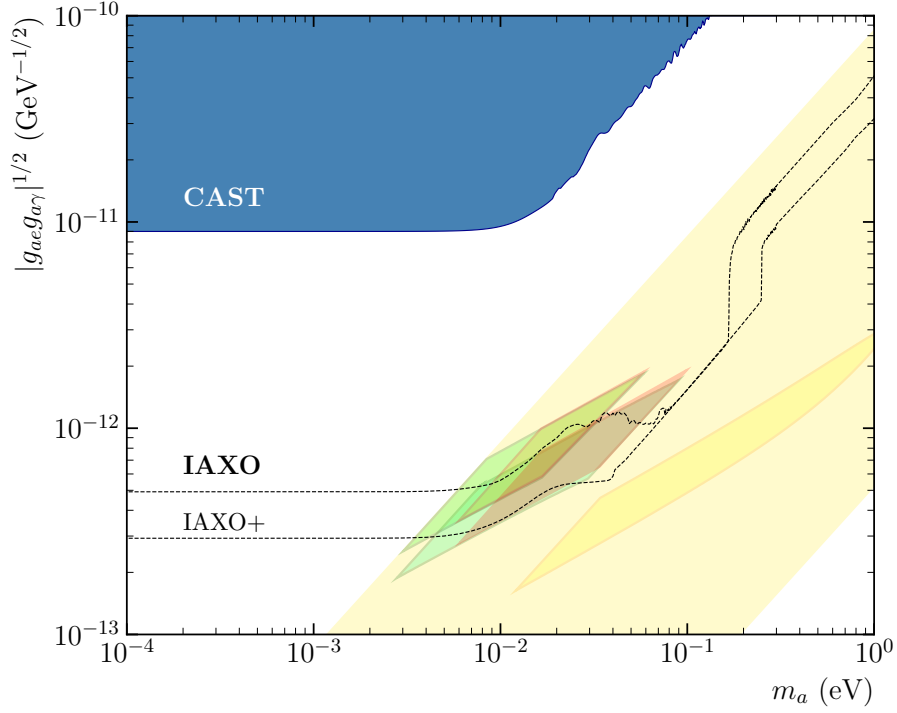
Figure 2. Sensitivity plot of IAXO to BCA ( g_{ae} -mediated) solar axions, in the (|g_{ae}g_{a\gamma}|^{1/2}-m_a) parameter space. The yellow band corresponds to the QCD axion models and the diamond-shaped color regions correspond to particular QCD axion models that are able to fit all the anomalous stellar cooling observations, following [23].
