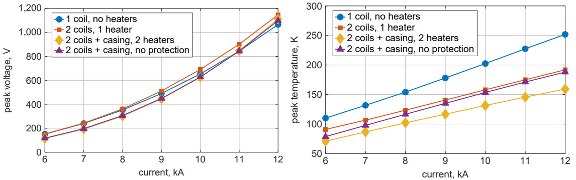
Figure 13. Peak voltage and peak temperature as a function of the operating current.
