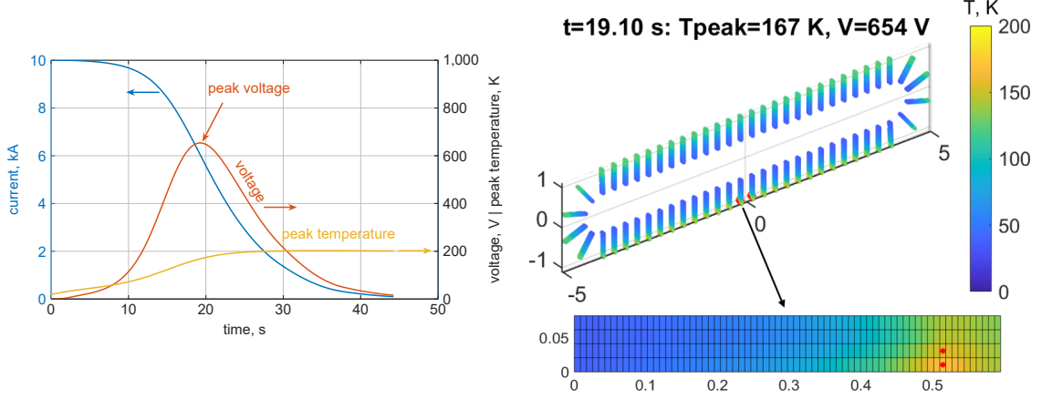
Figure 12. Left: time evolution of current, internal voltage and peak temperature of the magnet quenched at the operating current of 10 kA. Right: temperature distribution after a quench occurrence in a single coil at the moment of reaching the peak voltage.
