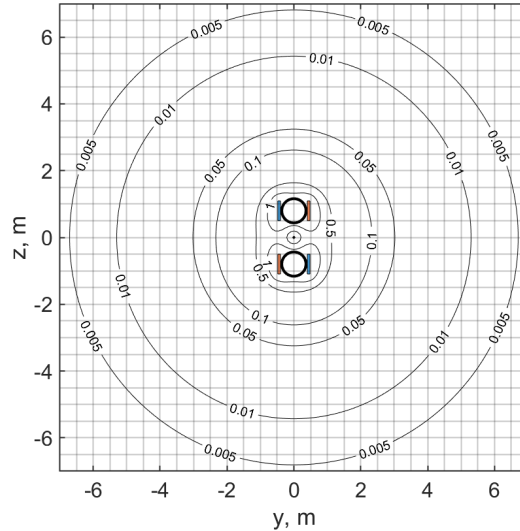
Figure 14. Map of stray magnetic field around the BabyIAXO magnet calculated in the magnet mid-plane for operation at 9.8 kA nominal current. The contour labels are in tesla.
