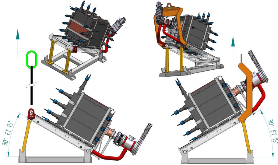
Figure 38. The setup to check the detector performance at different slope angles ( \pm 15^\circ degrees and \pm 30^\circ degrees).
