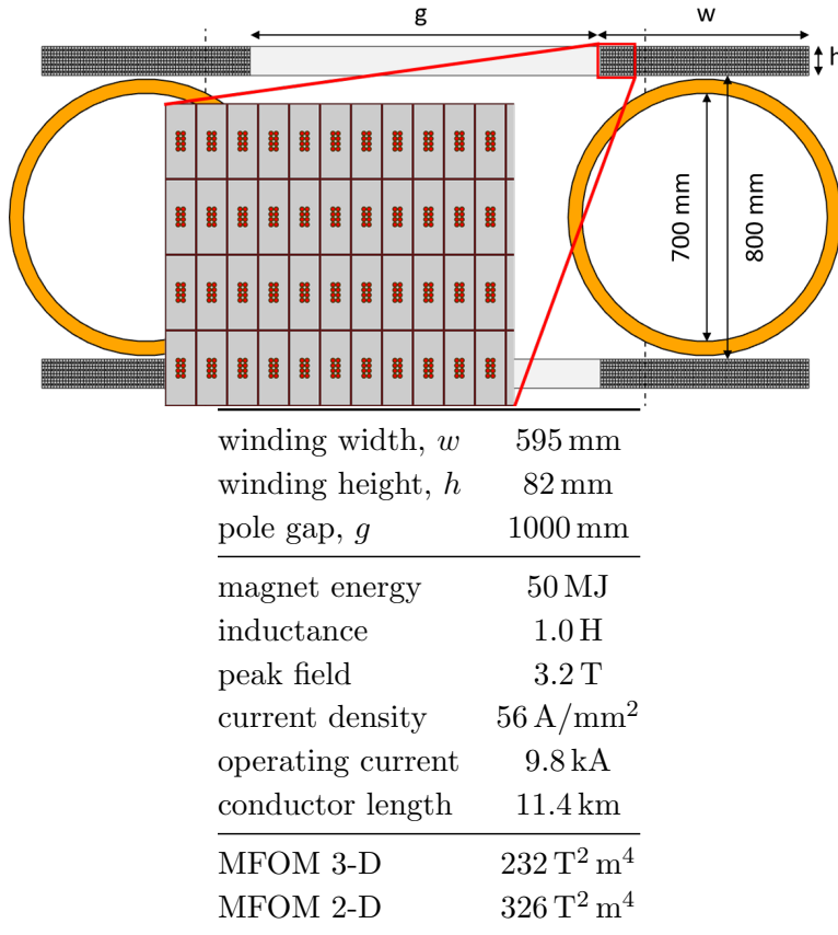
Figure 7. Design of the BabyIAXO coil windings with respect to the two used bores of 700 mm each. The insert shows a zoom of the four layer windings. The main magnet parameters are listed in the table.
