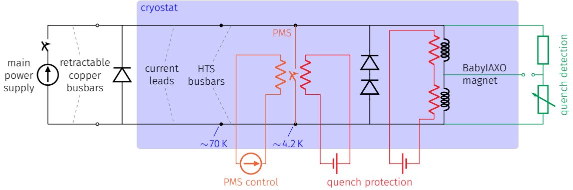
Figure 10. Electrical circuit (black) of the BabyIAXO magnet showing from left to right: the 10 kA power converter and its current breaker, bus bars, run-down resistor-diode unit, current leads, persistent mode switch PMS (orange) with its on-off heater and quench protection heaters, cold diodes across the magnet, the magnet itself equipped with quench protection heaters, and its quench detection unit (green). The various heaters are activated with low current power supplies. The in-cryostat parts are indicated in the violet area.
