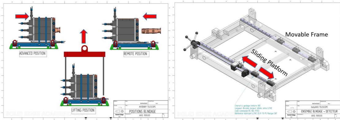
Figure 36. Left: Different movements of the Micromegas Detector shield assembly. Right: Perspective with a detailed view of the sliding platform and the movable frame components
