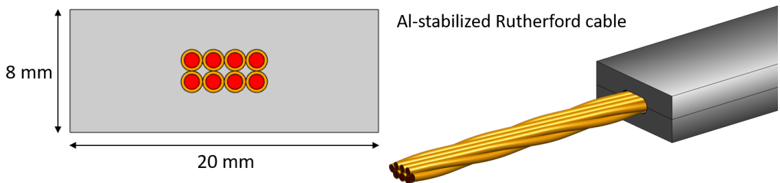
Figure 4. Cross-section (left) and artistic view (right) of the Al-stabilized 8 NbTi/Cu strands Rutherford cable.
