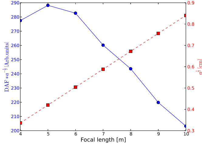
Figure 24. Value of the focal spot size \sqrt{a} (red squares and dashed line, right axis) and the figure of merit f_{\text{DO}} (blue circles and solid line, left axis) versus focal length f . The optimal figure of merit is found for f = 5 m.
