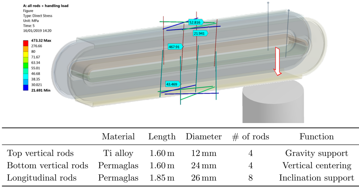
Figure 19. Design parameters and stress analysis of the multi-rods suspension system of the BabyIAXO cold mass. In total 16 rods are foreseen positioned in the center post. In addition a few extra rods, not yet dimensioned, will be added for transferring the Lorentz force load between cold mass and rotation tower.
