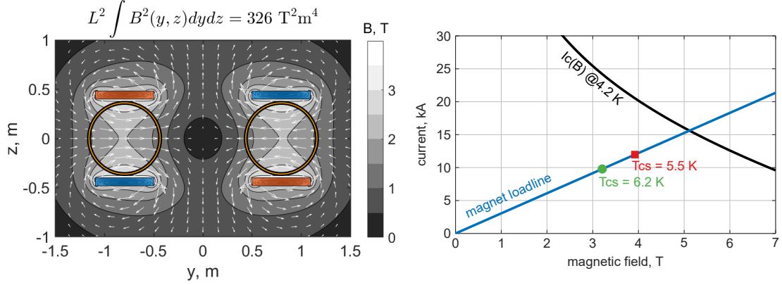
Figure 8. Left: distribution of the magnetic field in the magnet mid plane, with two bores and windings cross-section indicated (current directed outwards in red domains, inwards - in blue). Right: load line of the conductor in the coil windings with two operating points indicated for T_{cs} = 5.5 K and 6.2 K.
