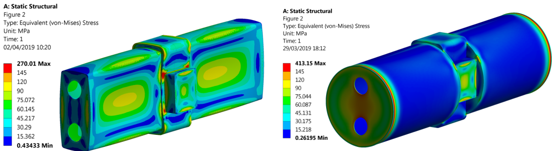
Figure 18. Von-Mises stress distribution in the rectangular (left) and circular (right) cryostats.
