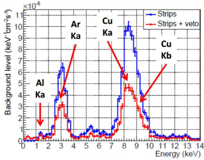
Figure 30. Background spectra obtained during the 2013-2015 data taking in the CAST experiment. Copper fluorescence peaks can be clearly seen as well as the escape peak of Ar at 3 keV. The difference between the two spectra is the effect of the muon veto.
