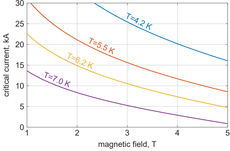
Figure 5. Dependence of the conductor critical current in kA on magnetic field in T at various temperatures between 4.2 K and 7.0 K.
