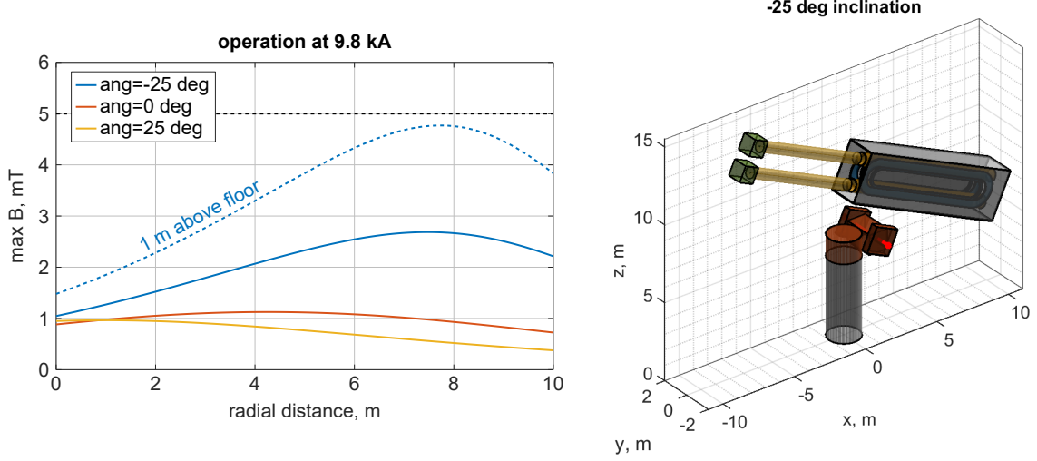
Figure 15. Stray magnetic field at z = 0 for minimum, zero and maximum inclination of the system operating at nominal current of 9.8 kA and at z = 1 m for the inclination at -25^\circ .
