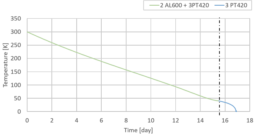
Figure 23. Cooling-down of the BabyIAXO cold mass by five cryocoolers within 17 days (not using the LN2 heat exchanger). At 45 K the cold mass is disconnected from the single stage AL600 machines and cool down continues using the three PT420 only.
