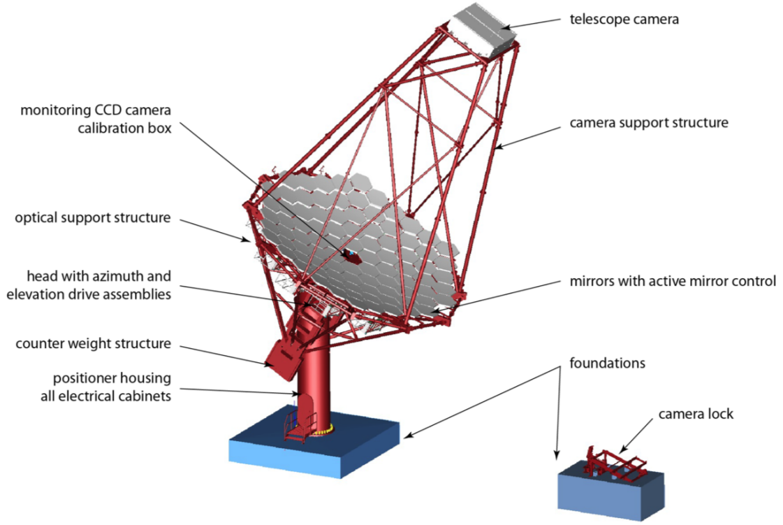
Figure 43. Overview of the complete MST assembly [128].
