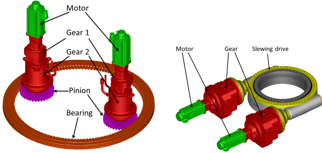
Figure 45. Left: azimuth drive sub-assembly [128]. Right: elevation drive sub-assembly [128].
