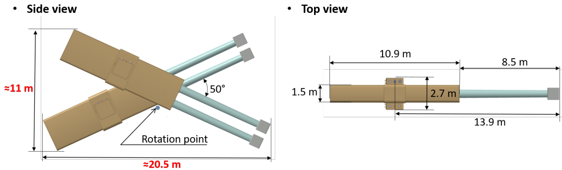
Figure 21. Main dimensions in side view and top view of the BabyIAXO cryostat with optics and detectors attached.
