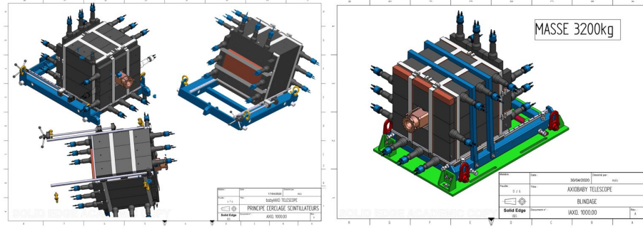
Figure 34. Left: Different views of the detector with the passive and active shield showing the 4\pi sr coverage. Right: Perspective of the whole assembly with the indicated weight.
