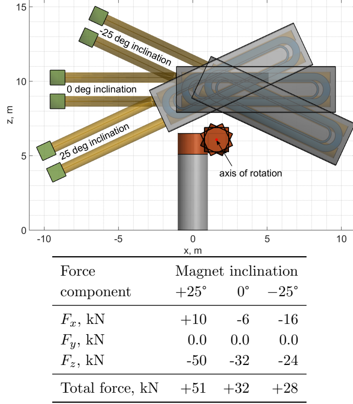
Figure 16. Left: schematic arrangement of the BabyIAXO components for the three angles of magnet inclination. Right: magnetic force on the magnet operated at 9.8 kA due to the magnetized drive system.
