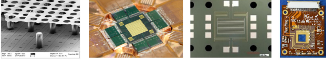
Figure 40. Active zone of a Gripix detector (left), MMC array (center-left), NbSi TES sensor (center-right) and SDD (right).
