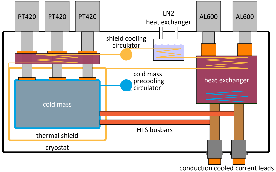
Figure 22. Layout of the innovative BabyIAXO “dry” cryogenic system based on using cryocoolers.
