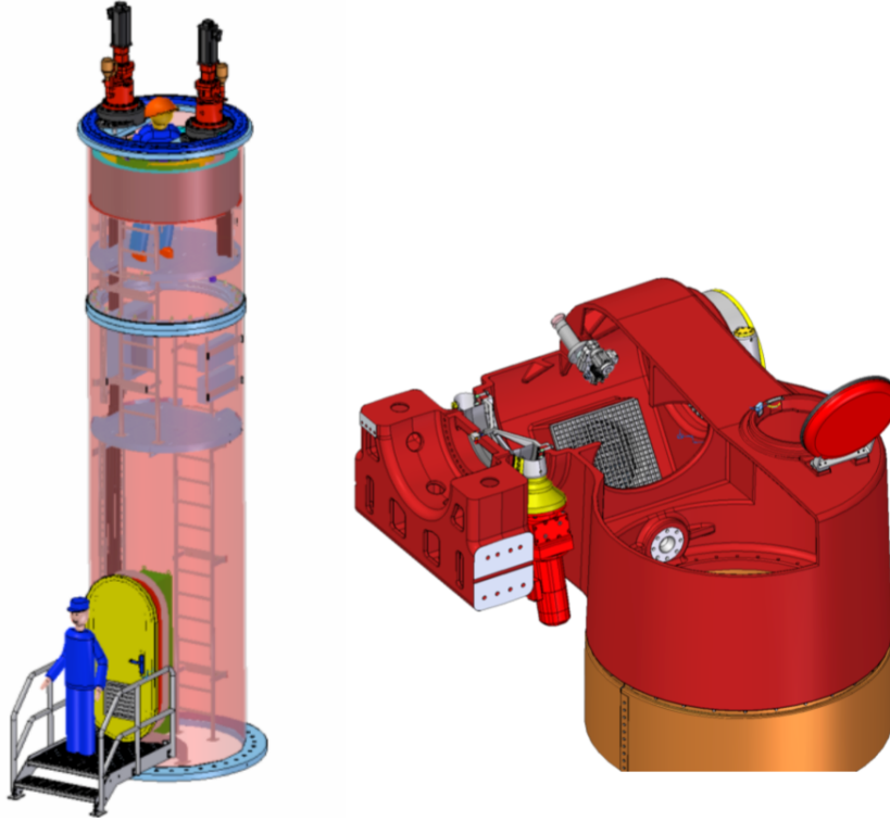
Figure 44. CAD view of the MST tower and head [128]. The scale of the two views is not the same.
