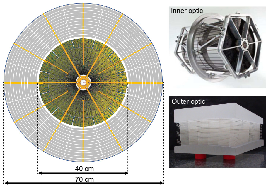
Figure 25. Left: Schematic view of the BabyIAXO optic, including the hexagonal “spider” structure that will be used to mount the optic to the magnet bores. The optic consists of an inner and outer part using two different glass-slumping and optics assembly technologies. The thousands of individual mirror segments are visible. Right: the top image shows the NuSTAR optic which forms the base of the inner part of the BabyIAXO optic, while the bottom image displays the cold-slumped glass technology that is going to be used to build the outer part of the axion telescope.
