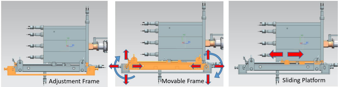
Figure 35. The components of the frame assembly with their movement degrees of freedom.
