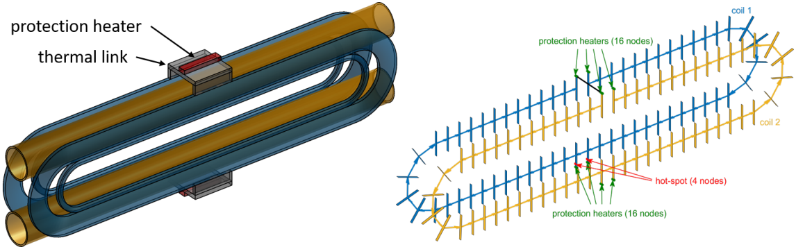
Figure 11. Left: sketch of the protection heaters installed on the cold mass, 2 units creating 4 normal zones in the two coils. Right: geometry of the quench propagation simulation model.
