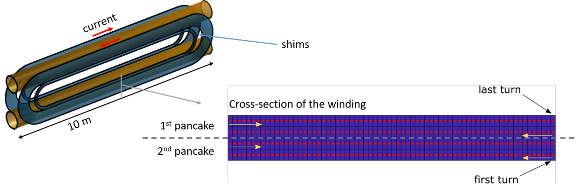
Figure 6. Schematic of the common-coil layout enclosing two user bores. In the coil heads shims or dummy turns of conductor are included in the 2 double-pancake winding for reducing the local peak magnetic field.
