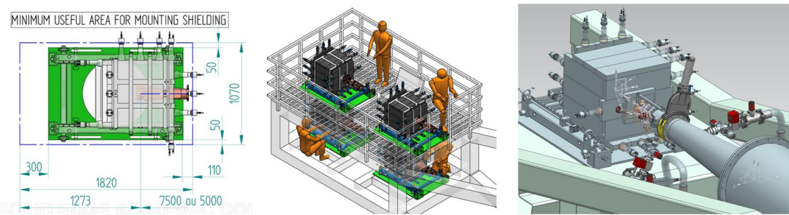
Figure 37. Left: Dimensions of the Micromegas detector assembly on the BabyIAXO platform. Middle: Preliminary detector layout onto the BabyIXO platform with two different focal lengths: 7.5 m and 5 m. Right: Tentative representation with the detector and the beamline components.
