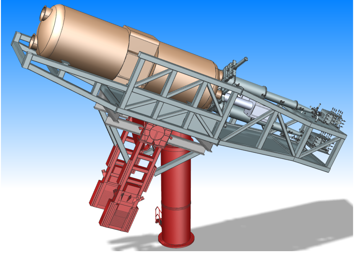
Figure 3. CAD overview of the full BabyIAXO assembly, including the magnet (assuming a cylindrical cryostat, see text), telescopes, detectors, support frame and MST positioner (in red, see section 7). Overall system length is about 19 meters. Although both detection lines are shown of equal length (corresponding to 7.5 m of focal length of the XMM optics), in reality one of the lines will be shorter (5 m focal length, see section 5).
