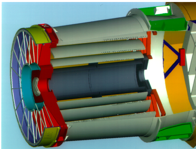
Figure 27. 3D model of XMM Newton telescope showing a few of its 58 full-revolution nickel shells that have been coated with gold.
