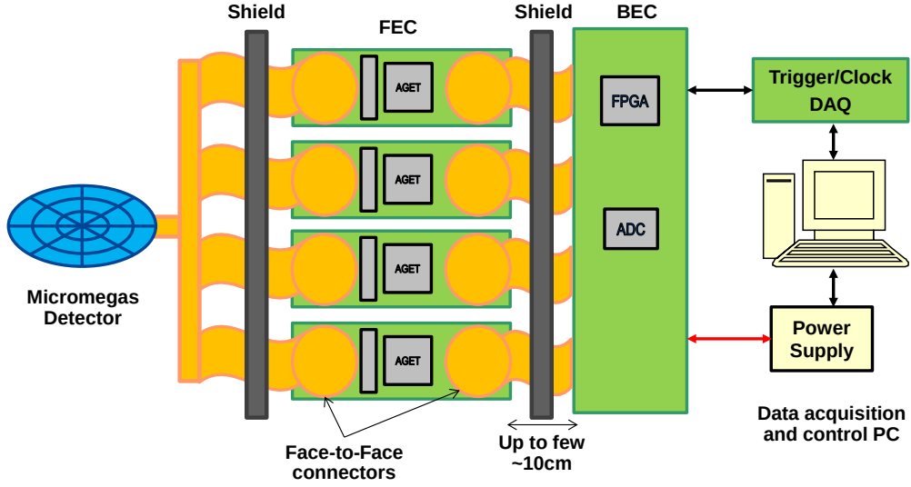
Figure 39. Electronics readout block diagram.
