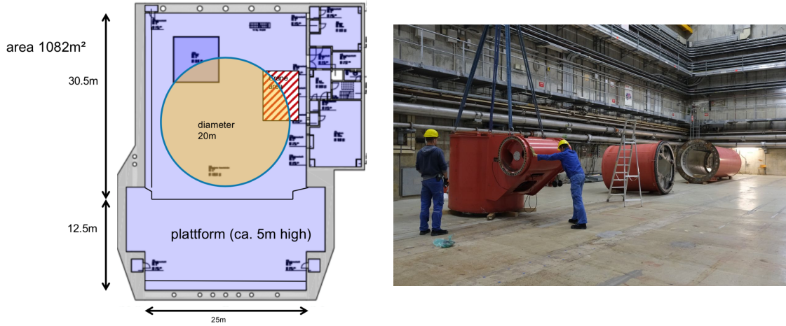
Figure 47. Left: Floor plan of the HERA South Hall including a circle of 20 m diameter indicating the movement of BabyIAXO. Right: Photograph of the South Hall craning in the head of the structure and drive system.
