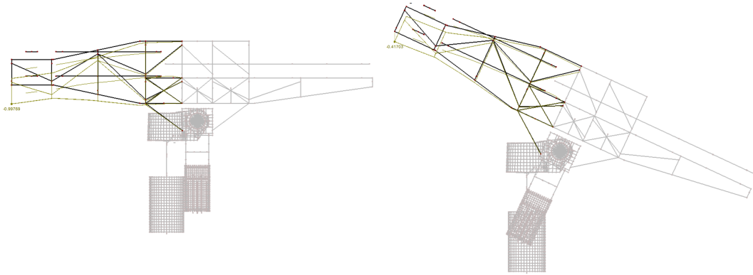
Figure 46. Deformation of the backside of the support frame due to the gravitational load at 0^\circ and 25^\circ . For illustration, the deformations are scaled up by a factor of 1000 (left) and 1200 (right figure).
