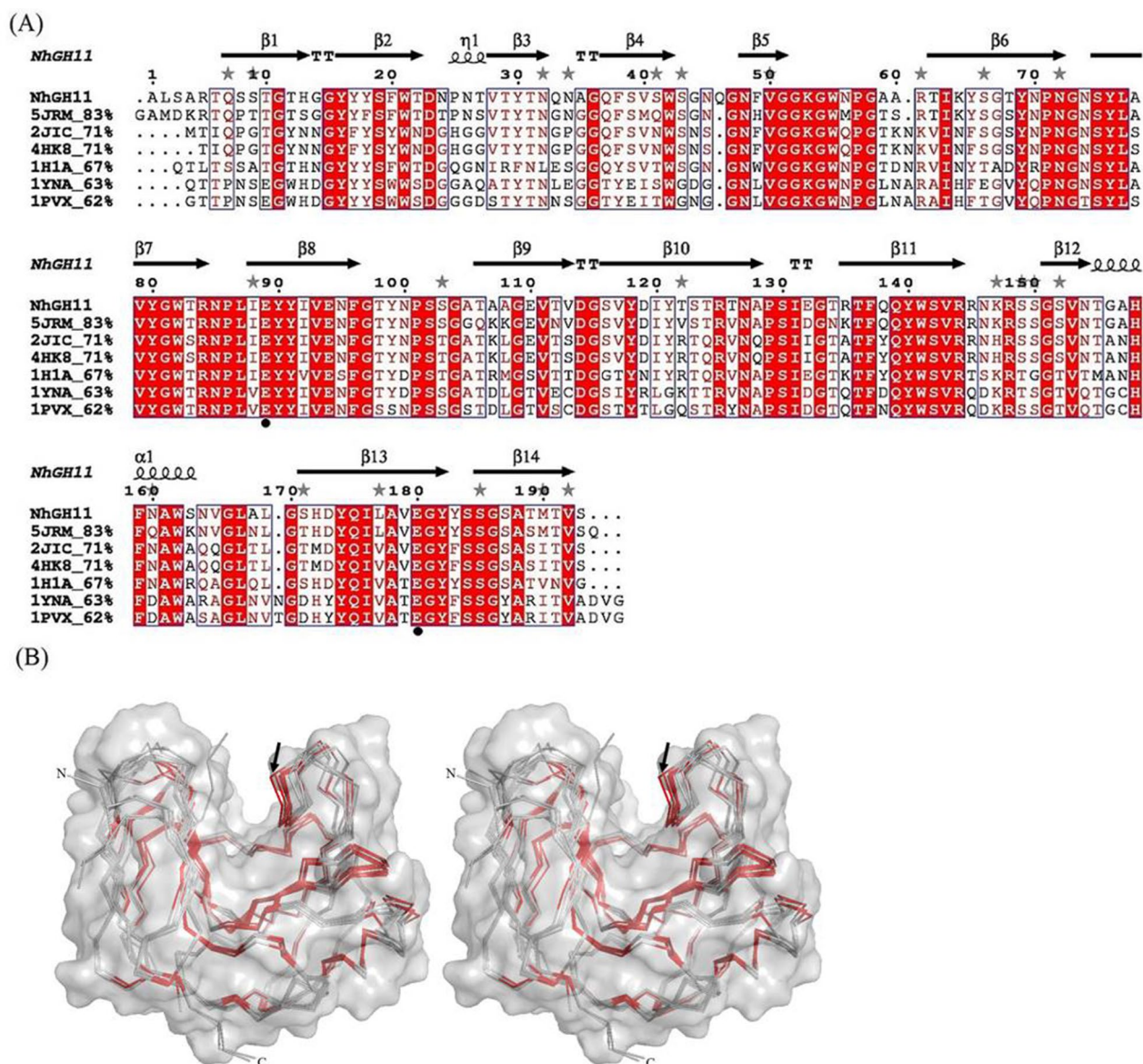
Figure 2. (A) Sequence alignment and comparison with homologous GH11 enzymes. Secondary structure regions are indicated along with gray stars indicating residues with alternative side chain conformations in the NhGH11 structure. Sequence alignment was done applying ESPript3 ( http://esprict.ibcp.fr/ESPript/ESPript ). Residues in red color are identical and residues in pink color show similarity among aligned sequences. Catalytic residues E89 and E180 are indicated with filled circles. For the structure with pdb code 4HK8 the second catalytic E180 was mutated to Q180 for ligand binding studies (B) Stereo view of the surface representation with under laid Ca tracing. NhGH11 superimposed with homologue structures (pdb codes: 5JRM, 2JIC, 4HK8, 1H1A, 1YNA and 1PVX) from F. oxysporum , T. longibrachiatum , H. jecorina , C. thermophilum , T. lanuginosus and B. spectabilis respectively. Backbone in red color indicates regions with sequence identity for all structures, the highly conserved thumb region is indicated by black arrows.
