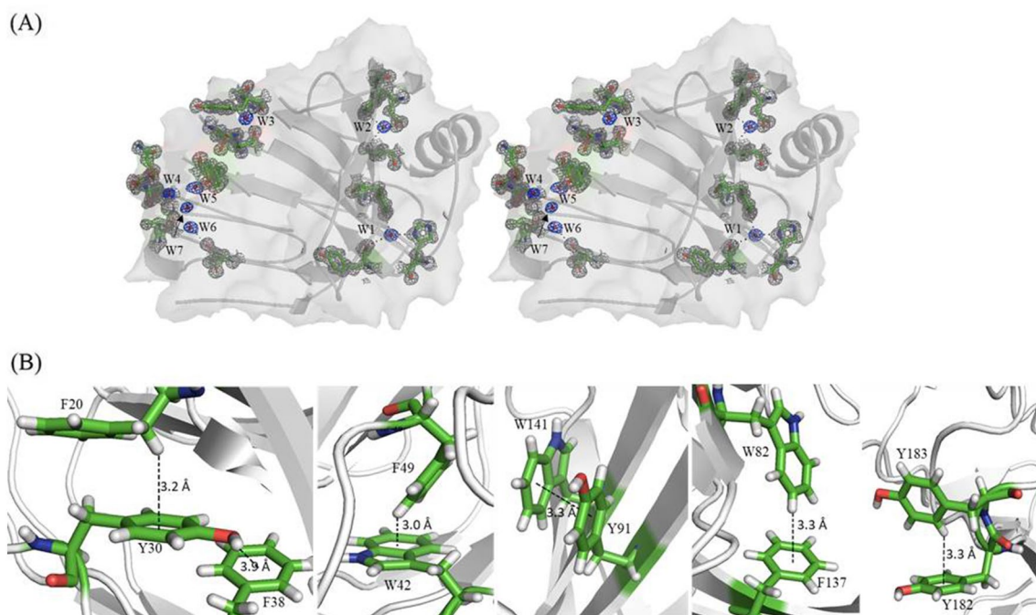
Figure 5. (A) Stereo figure showing buried water molecules with electron density within the cartoon surface representation. 2Fo-Fc electron density maps for water molecules and surrounding residues are shown at 1.0 \sigma level. (B) Selected intramolecular aromatic-aromatic ( \pi \cdots \pi ) interactions and C-H \cdots \pi interactions. Interactions were considered if the distance between the interacting proton and centroid of the phenyl group is less than 3.5 Å.
