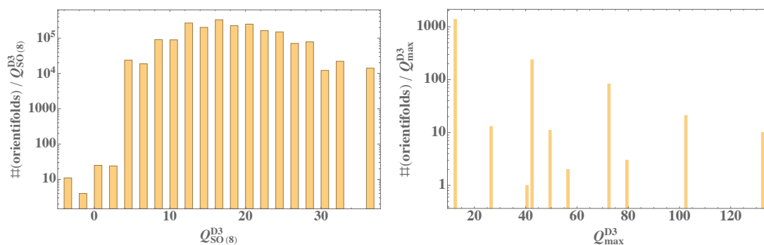
Figure 4. Left: histogram showing the number of orientifolds with given D3-tadpole -Q_{\text{SO}(8)}^{D3} = \chi_f/4 for local D7-charge cancellation. The tadpole takes even values in [-4, 36] . Right: D3-tadpole for a small set of examples with non-local tadpole cancellation by a generic D7-brane. We have restricted ourselves to the subset of smooth CICYs where the O7 divisor obviously descends from an ambient space divisor. The tadpole takes even values in a significantly larger range [12, 132] .
