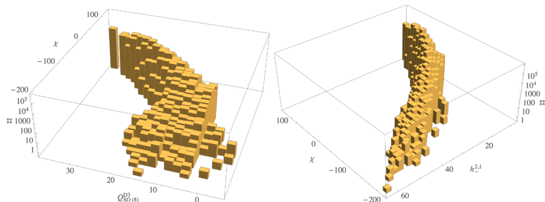
Figure 5. Histograms showing on a logarithmic scale the number of orientifolds. Left: count for each value of (Q_{\text{SO}(8)}^{D3}, \chi) . Right: count for each value of (h_-^{2,1}, \chi) . The steep cliffs carve out clear islands embedded in large otherwise empty regions.
