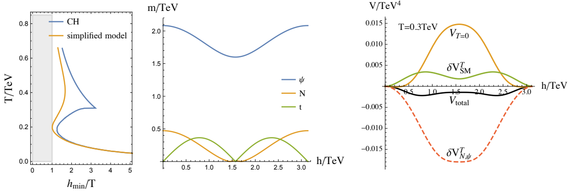
Figure 7. Left: h/T evolution with a temperature, in the simplified model ( \lambda_N/\Lambda = 0.4 \text{ TeV}^{-1} , m_N(v) = 0.45 \text{ TeV} , \Lambda = 2.1 \text{ TeV} , n = 15 ) and in the respective point of the parameter space of the CH model ( y_L = -y_R = 1 , m_N^0 = 0.1 \text{ TeV} , m_\psi^0 = -1.6 \text{ TeV} , f = 1 \text{ TeV} ). In the CH case we plot f \sin(h/f)/T instead of h/T , as EW gauge bosons masses are \propto f \sin(h/f) . The h/T lines are limited by the perturbativity from above. Center: mass spectrum of the fermions producing the dominant thermal effects. Right: overall Higgs potential at T = 0.3 \text{ TeV} (black), zero-temperature potential (orange), thermal potential from SM degrees of freedom (green) and thermal potential induced by N and \psi (red dashed).
