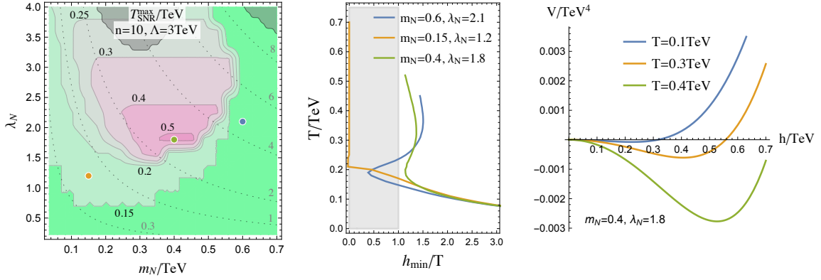
Figure 5. Left: maximal SNR temperature (colored regions, black labels) for \Lambda = 3 TeV, n = 10 and \mu = 1 TeV, in terms of the coupling \lambda_N and m_N — zero-temperature mass of N at h = 246 GeV. Grey dotted contours with grey labels show the values of \alpha = n\lambda_N m_N^{(0)}/\Lambda . Grey areas feature zero-temperature barriers at h < m_N^{(0)}\Lambda/\lambda_N . Center: temperature dependence of h/T , for three combinations of m_N and \lambda_N (corresponding to the three colored points on the left plot). The h/T lines are limited by the perturbativity from above. Right: Higgs potential at T = 0.1, 0.3, 0.4 TeV, for m_N = 0.4 TeV, \lambda_N = 1.8 .
