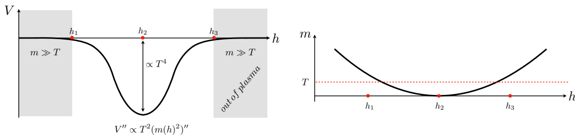
Figure 1. Sketch of the thermal correction to the Higgs potential (left panel) induced by particles in the plasma whose mass depends on the Higgs field as shown on the right panel. At high temperature, a dip is induced in the potential at the point where the particle mass term vanishes.
