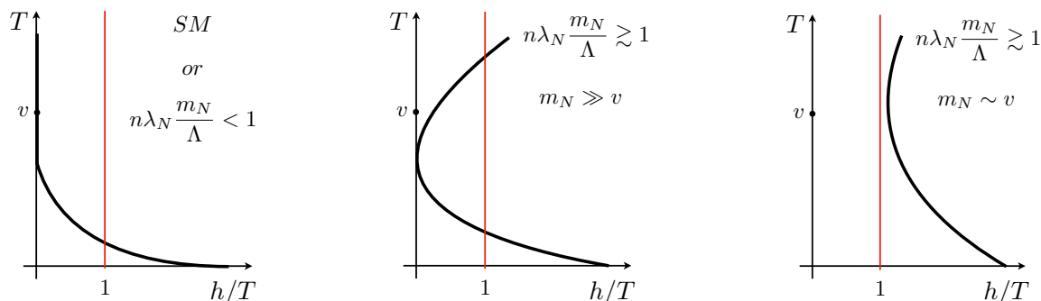
Figure 3. Schematic plots of h/T dependence on the temperature. Left: behaviour found in the SM, or in a model with new fermions where the SNR condition (2.13) is not met. Center: model with new fermions where the SNR condition is satisfied, but the fermions are too heavy to affect the Higgs potential at temperatures around the EW scale. Right: model with new fermions satisfying the SNR condition and light enough to contribute to the Higgs potential at temperatures around the EW scale, such that the sphaleron bound h/T \gtrsim 1 is always satisfied. For both the center and right plots, we have assumed that the position of the minimum of the thermal part of the potential induced by the new fermions, h^2 = m_N^{(0)} \Lambda / \lambda_N , is always greater than T^2 within the plotted temperature range. This explains why h/T exceeds 1 at high T .
