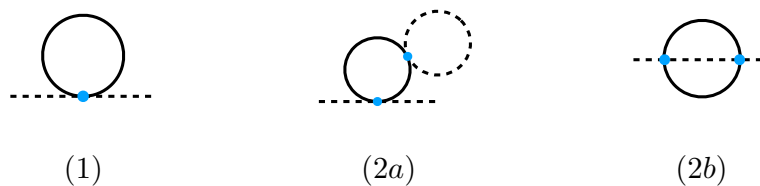
Figure 4. The leading one-loop correction to the Higgs mass (1) and two-loop corrections (2a, 2b). Dashed lines correspond to the Higgs boson and solid to N .
