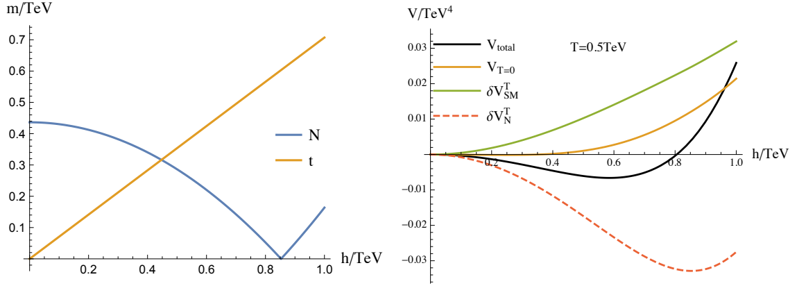
Figure 2. Left: top quark mass (orange) and the N fermion mass, which is minimized at large Higgs vev (blue). Right: corresponding 1-loop Higgs thermal potential featuring SNR at T = 0.5 TeV (black solid) and its decomposition into non-thermal part (orange solid), finite temperature corrections from the SM interactions (green solid) and from the interactions with the N fermions (red dashed). The maximal negative correction from the N fermions is at the point of vanishing N mass corresponding to large Higgs vev . For these plots we chose n = 10 , \Lambda = 1 TeV, \lambda_N = 0.6 , m_N(v_{\text{SM}}) = 0.4 TeV.
