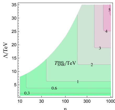
Figure 6. Contours of maximal T of SNR (such that h/T > 1 down to T = 0 ), as a function of \Lambda and n . In the white area the perturbativity constraint on \lambda_N (3.14) prevents SNR.
