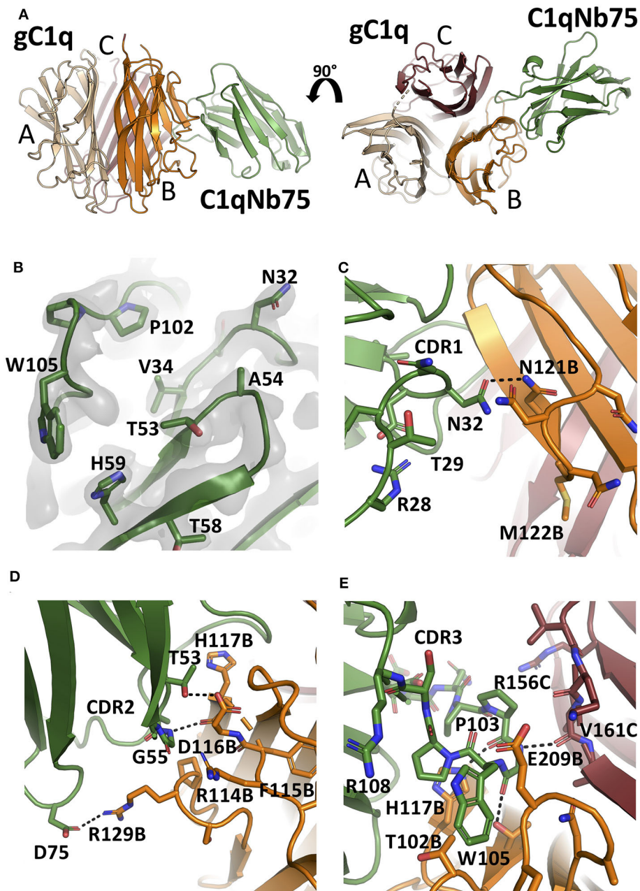
FIGURE 4 | The crystal structure of the gC1q-C1qNb75 complex reveals the epitope. (A) Side view (left) and top view (right) of the gC1q-C1qNb75 complex. The different subunits of gC1q are colored in wheat (A-chain), orange (B-chain) and brown (C-chain) whereas C1qNb75 is displayed in green. (B) Omit 2mF o -DF c electron density map contoured at 1.2σ around the three CDRs. Residues shown with side chains in sticks were omitted for map calculation. (C-E) The interface between gC1q and C1qNb75 with selected residues shown in sticks. (C) CDR1 contacts, (D) CDR2 contacts, (E) CDR3 contacts. Hydrogen bonds are shown with black dashes. The gC1q residues are labeled with their chain identifier as suffix.
