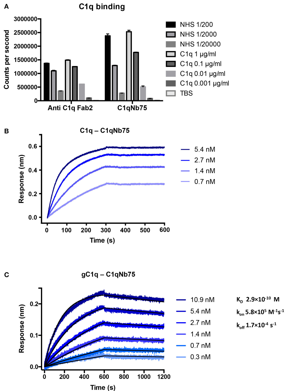
FIGURE 1 | C1qNb75 binds with high affinity to human C1q. (A) Solid-phase immunoassay (TRIFMA) with anti-C1q Fab2 or C1qNb75 coated in microtiter wells. The binding of purified C1q or C1q in NHS is measured. The signal is given as counts per second after measurement by time-resolved fluorometry. Shown are mean and SD. (B) Bio-layer interferometry (BLI) measurement of the interaction between purified C1q in solution and immobilized C1qNb75. (C) As in previous panel but showing the interaction between recombinant gC1q and immobilized C1qNb75 with calculated k_{on} , k_{off} , and K_D . The Experimental data (blue curves) was globally fitted to a 1:1 binding model (black curves).
