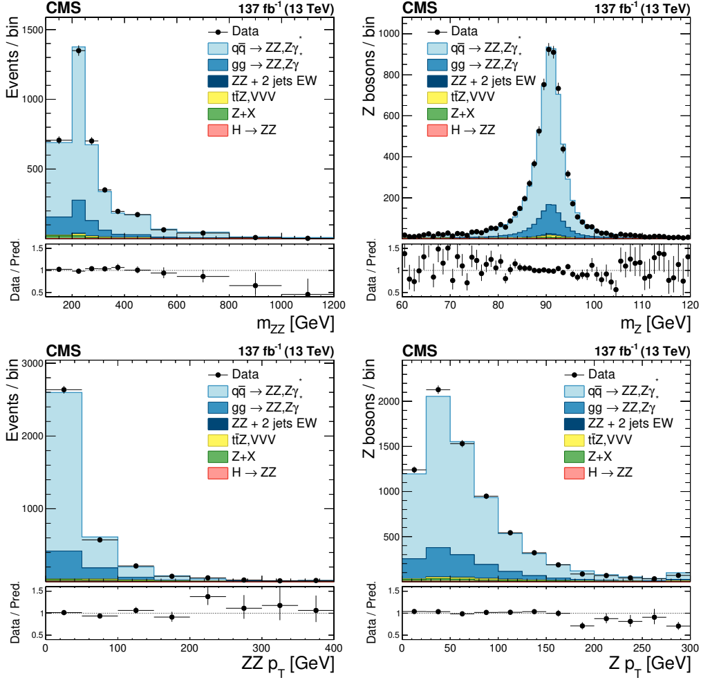
Figure 2: Distributions of (upper left) m_{ZZ} for ZZ events with 60 < m_{Z_1 Z_2} < 120 GeV; (upper right) mass of selected Z boson candidates; (lower left) transverse momentum of the ZZ system; (lower right) transverse momentum of individual Z boson candidates. Points represent the data with error bars showing the statistical uncertainties, histograms the expected SM predictions and reducible background estimated from data.
