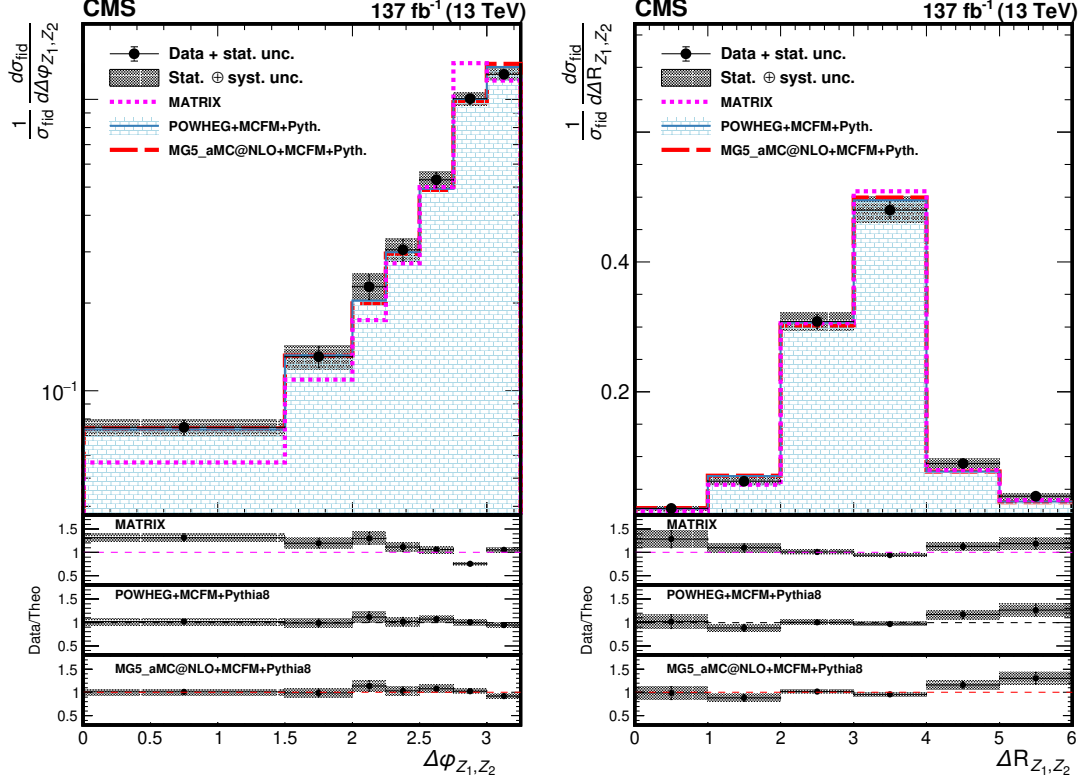
Figure 6: Differential cross sections normalized to the fiducial cross section for the combined 4e , 2e2\mu , and 4\mu decay channels as a function of the azimuthal and \Delta R separation of the two Z bosons. The points represent the unfolded data with error bars showing the statistical uncertainties, the shaded histogram the POWHEG+MCFM ZZ predictions, and the dashed curves correspond to the results of the MATRIX and MADGRAPH5_aMC@NLO+MCFM calculations. The three lower panels represent the ratio of the measured cross section to the expected distributions from MATRIX, POWHEG+MCFM and MADGRAPH5_aMC@NLO+MCFM. The shaded areas in all the panels represent the full uncertainties calculated as the quadratic sum of the statistical and systematic uncertainties, whereas the crosses represent only the statistical uncertainties.
