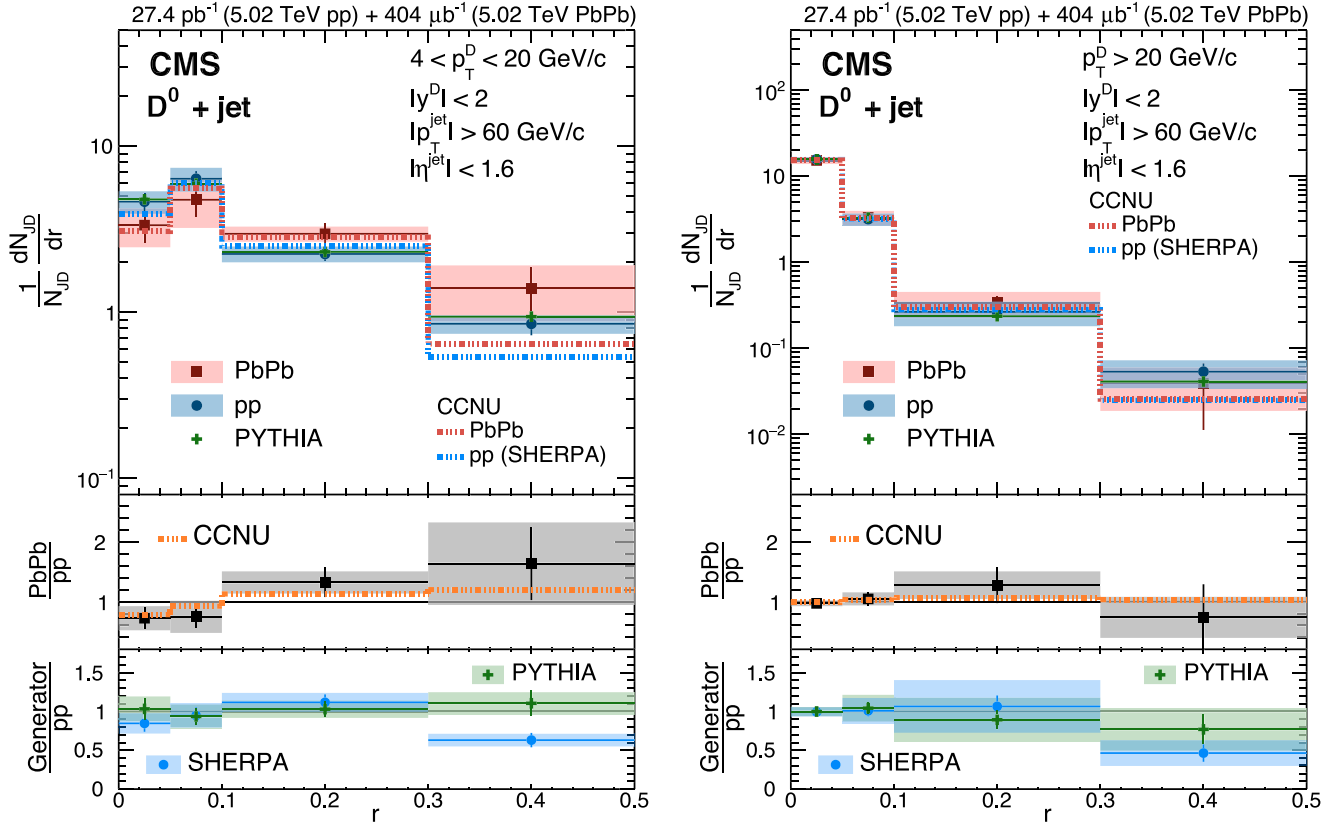
FIG. 1. Distributions of D^0 mesons in jets, as a function of the distance from the jet axis ( r ) for jets of p_T^{\text{jet}} > 60 GeV/ c and |\eta^{\text{jet}}| < 1.6 measured in pp and Pb-Pb collisions at \sqrt{s_{NN}} = 5.02 TeV. The measurement is performed in the p_T^D range 4 – 20 GeV/ c (left) and p_T^D > 20 GeV/ c (right). Each spectrum is normalized to its integral in the region 0 < r < 0.3 . The vertical bars (boxes) correspond to statistical (systematic) uncertainties. The Pb-Pb spectra are compared to the CCNU energy loss model [21], while the pp spectra are compared with predictions from the PYTHIA and SHERPA pp MC event generators. The ratios of the D^0 meson radial distributions in Pb-Pb and pp data are shown in the middle panels. In the bottom panels, the ratios of the D^0 meson radial distributions of pp over the two MC event generators are presented.
