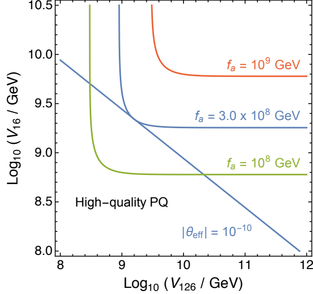
Figure 2: Parameter space of the accidental SO(10) axion leading to a high-quality U(1) PQ . For the estimate of the induced QCD theta term we used Eq. (3.9) with |k| = 1 and \sin \delta = 1 .
