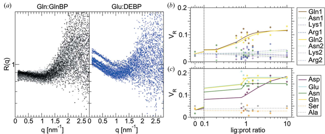
Figure 6 Summary of SAXS-based screening performance on GlnBP and DEBP. (a) Ratio curves of R(q) for the titration between GlnBP and DEBP with its cognate ligands Gln and Glu, respectively. (b) V_R curves for the prospective screening trial of GlnBP with native and other amino acid targets. (c) V_R curves for the prospective screening trial of DEBP with native and other amino acid targets. For comparison, equivalent curves using other metrics are shown in Fig. S14.
