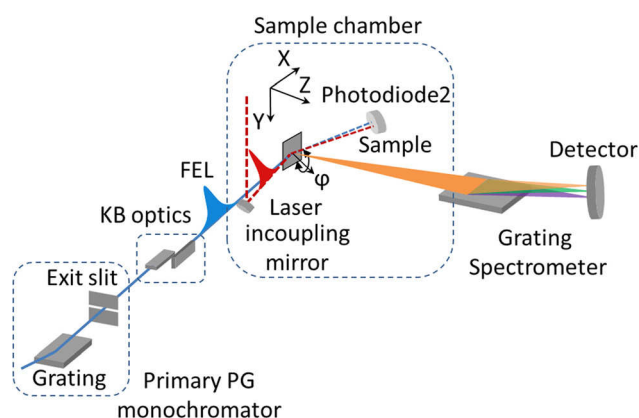
FIG. 1. Schematic overview of the TRIXS end-station including the monochromator beamline PG1 and its focusing optics. Spectrometer is shown without focusing optics.
