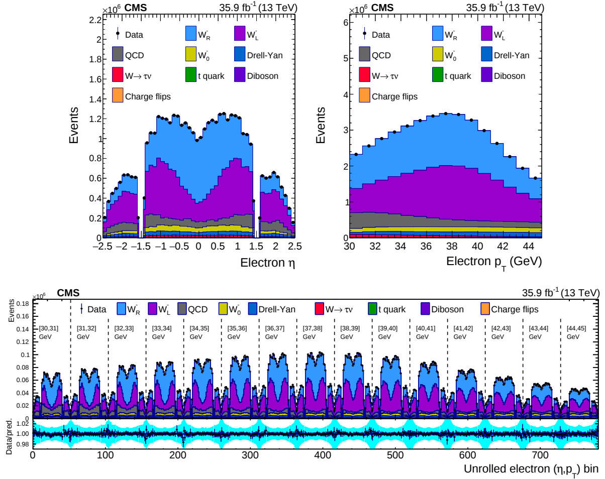
Figure 8: Distributions of \eta^e (upper left), p_T^e (upper right) and \text{bin}_{\text{unrolled}} (lower) for W^- \rightarrow e^- \bar{\nu} events for observed data superimposed on signal plus background events. The signal and background processes are normalized to the result of the template fit. The cyan band over the data-to-prediction ratio represents the uncertainty in the total yield in each bin after the profiling process.
