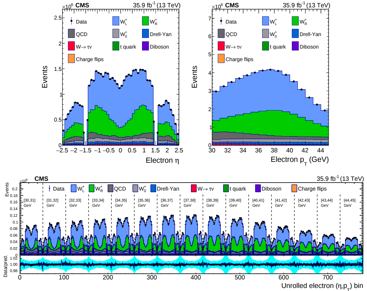
Figure 7: Distributions of \eta^e (upper left), p_T^e (upper right) and \text{bin}_{\text{unrolled}} (lower) for W^+ \rightarrow e^+ \nu events for observed data superimposed on signal plus background events. The signal and background processes are normalized to the result of the template fit. The cyan band over the data-to-prediction ratio represents the uncertainty in the total yield in each bin after the profiling process.
