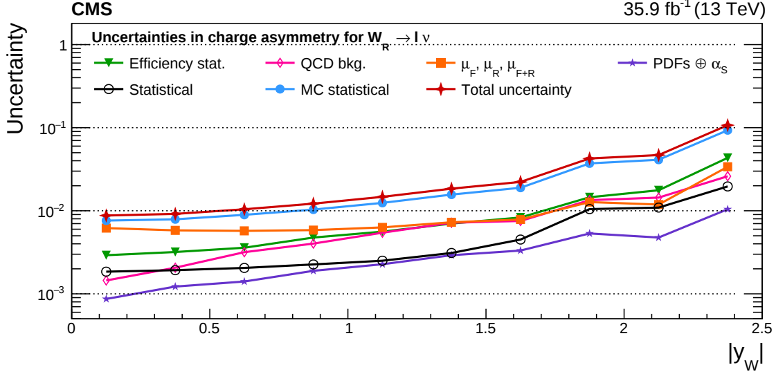
Figure A.13: Impacts on the charge asymmetry as functions of the W boson rapidity for W_R bosons in the helicity fit. The groups of uncertainties subleading to the ones shown are suppressed for simplicity.
