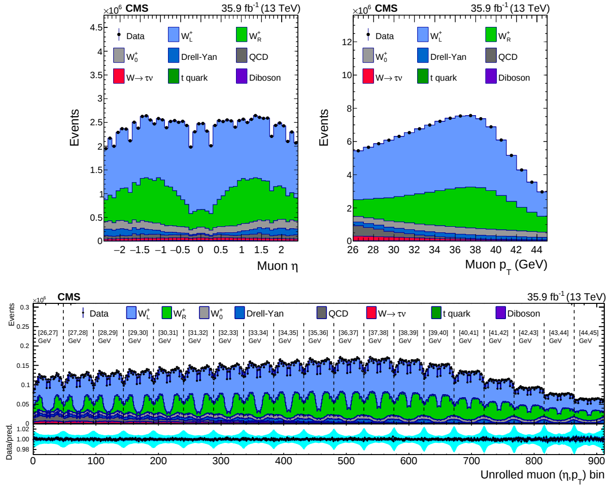
Figure 5: Distributions of \eta^\mu (upper left), p_T^\mu (upper right) and \text{bin}_{\text{unrolled}} (lower) for W^+ \rightarrow \mu^+ \nu events for observed data superimposed on signal plus background events. The signal and background processes are normalized to the result of the template fit. The cyan band over the data-to-prediction ratio represents the uncertainty in the total yield in each bin after the profiling process.
