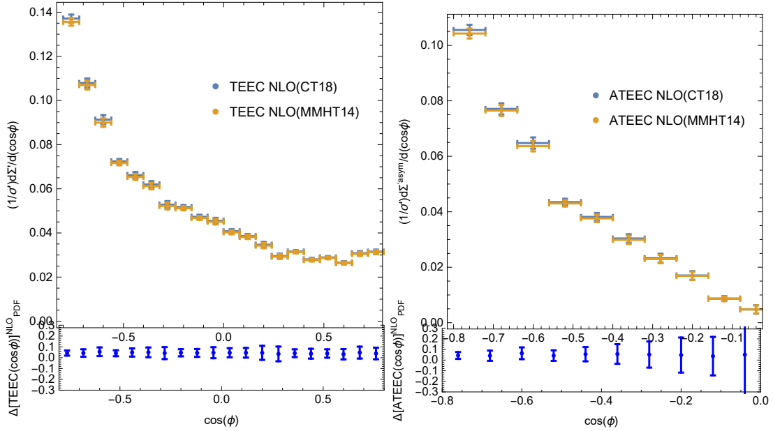
FIG. 3: Differential distribution 1/\sigma' d\Sigma'/d(\cos \phi) and its asymmetry 1/\sigma' d\Sigma'^{asym}/d(\cos \phi) as in Fig. 2, but for the high- Q^2 range 150 \text{ GeV}^2 < Q^2 < 1000 \text{ GeV}^2 at HERA.
