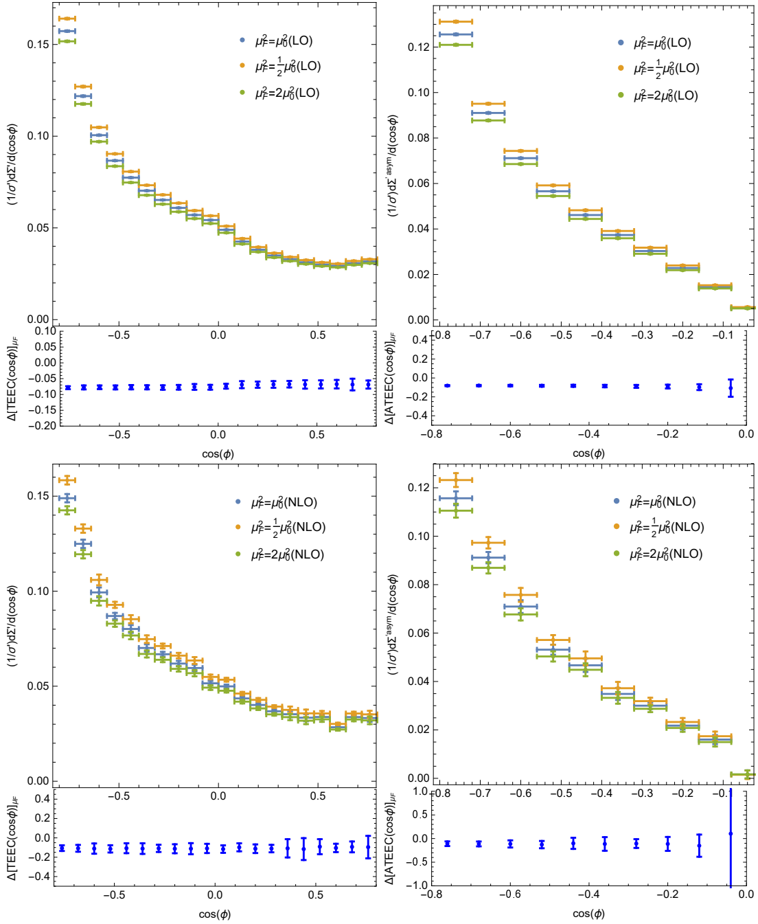
FIG. 4: Factorization scale dependence of the differential distribution 1/\sigma' d\Sigma'/d(\cos\phi) and its asymmetry 1/\sigma' d\Sigma'^{asym}/d(\cos\phi) in the leading order (upper frames), and the next to leading order (lower frames), varying \mu_F^2 in the range [0.5, 2] \times \mu_0^2 , where \mu_0 is the nominal scale defined in the text, calculated with the MMHT14 PDFs for the low- Q^2 : 5.5 \text{ GeV}^2 < Q^2 < 80 \text{ GeV}^2 at HERA. The corresponding \mu_F -dependence is also shown in terms of \Delta[\text{TEEC}(\cos\phi)]_{\mu_F} and \Delta[\text{ATEEC}(\cos\phi)]_{\mu_F} , defined in Eq. (16).
