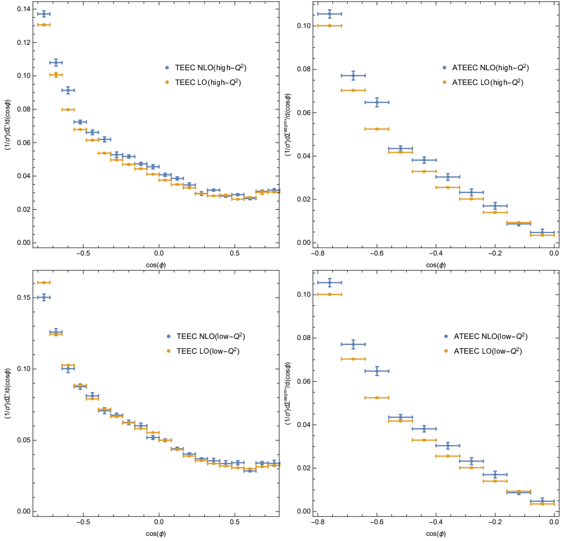
FIG. 10: A comparison of the LO and the NLO differential distribution 1/\sigma' d\Sigma'/d(\cos\phi) (left) and its asymmetry 1/\sigma' d\Sigma'^{asym}/d(\cos\phi) (right) at HERA ( \sqrt{s} = 314 GeV) in the high- Q^2 range (upper frames) and low- Q^2 range (lower frames), with \mu_F = \mu_R = \mu_0 = \sqrt{\langle E_T \rangle^2 + Q^2} and \alpha_s(M_Z) = 0.118 .
