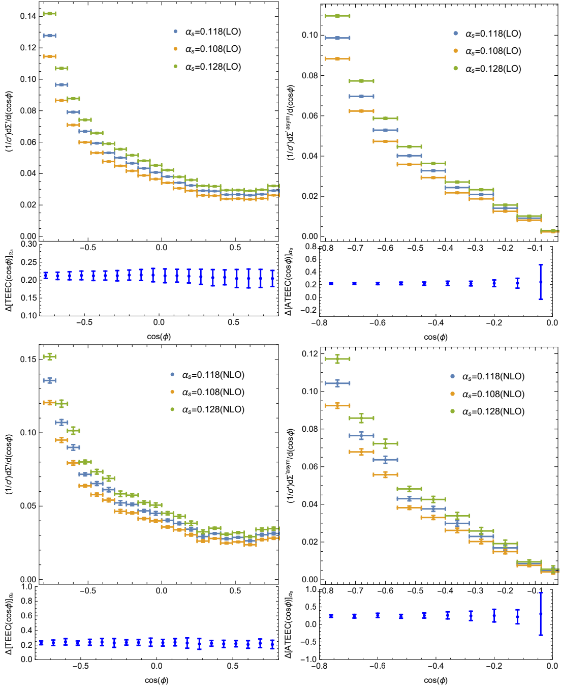
FIG. 9: Dependence of the differential distribution 1/\sigma' d\Sigma'/d(\cos\phi) (left) and its asymmetry 1/\sigma' d\Sigma'^{a.sym}/d(\cos\phi) (right) on the QCD coupling constant \alpha_s(M_Z) as in Fig. 8, but for the high- Q^2 range at HERA.
