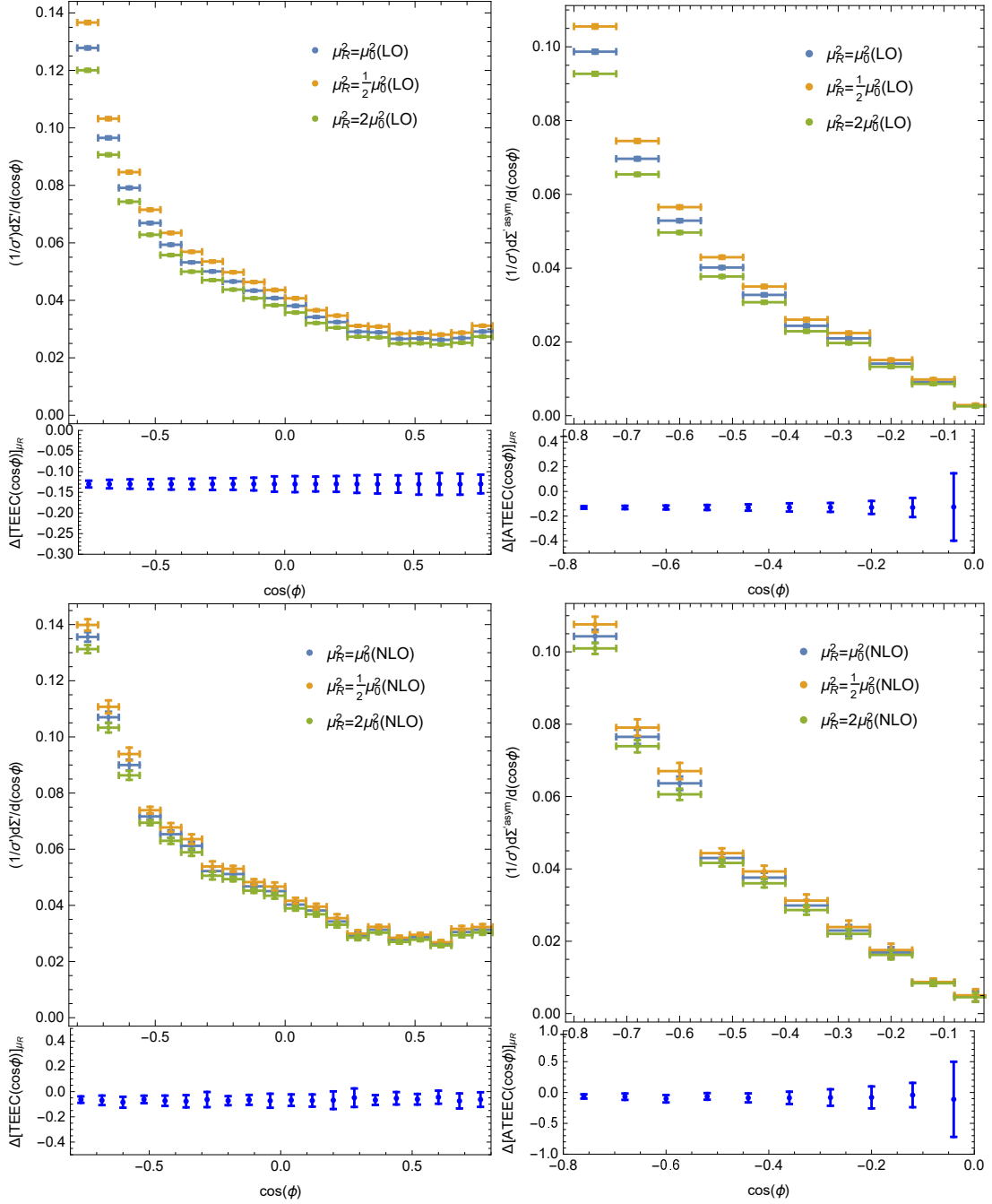
FIG. 7: Renormalization scale dependence of the differential distribution 1/\sigma' d\Sigma'/d(\cos\phi) and its asymmetry 1/\sigma' d\Sigma'^{asym}/d(\cos\phi) in the leading order (upper frames) and the next to leading order (lower frames) as in Fig. 6, but for the high- Q^2 range: 150 \text{ GeV}^2 < Q^2 < 1000 \text{ GeV}^2 at HERA.
