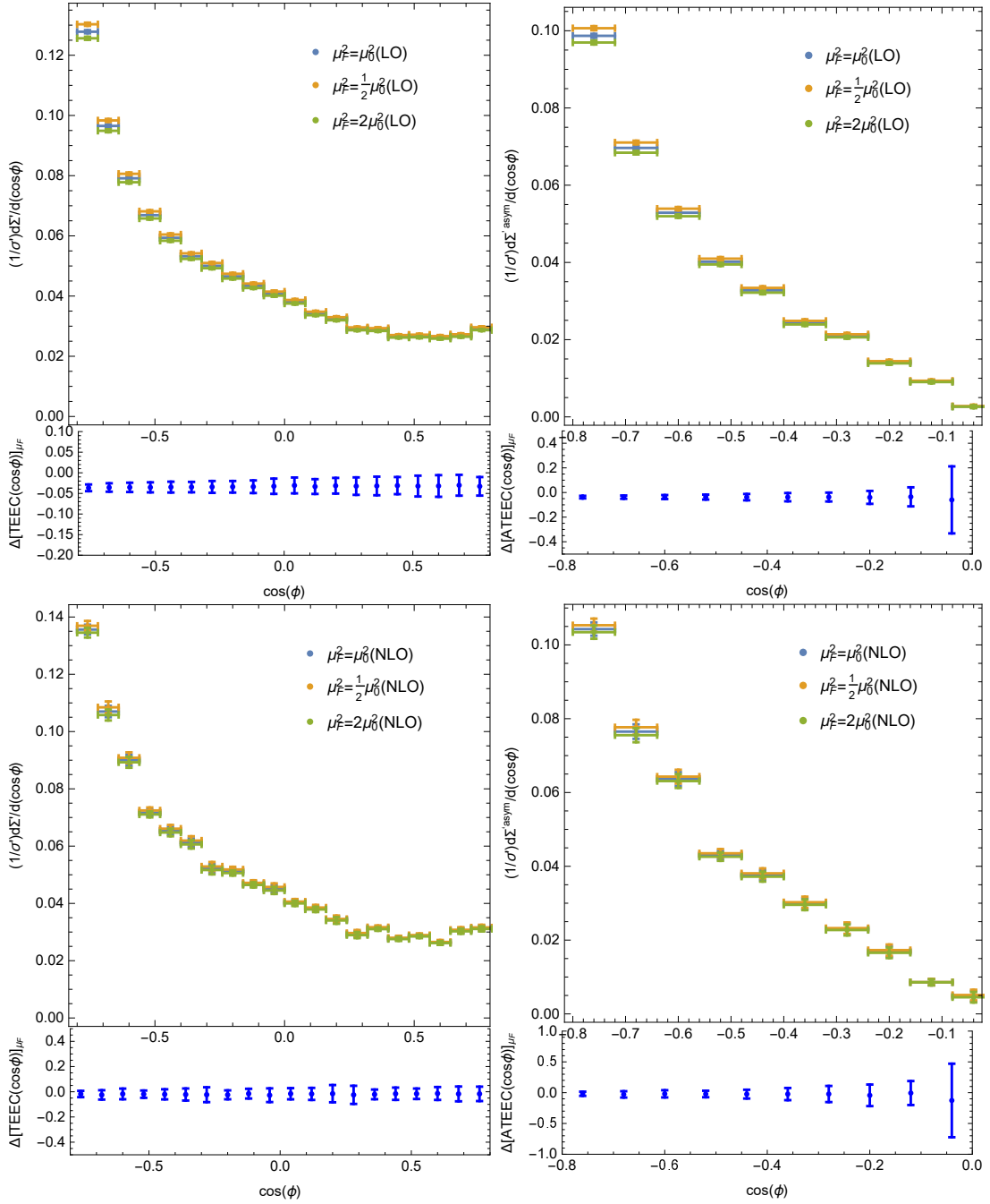
FIG. 5: Factorization scale dependence of the differential distribution 1/\sigma' d\Sigma'/d(\cos \phi) and its asymmetry 1/\sigma' d\Sigma'^{asym}/d(\cos \phi) in the leading order (upper frames) and the next to leading order (lower frames) as in Fig. 4, but for the high- Q^2 range 150 \text{ GeV}^2 < Q^2 < 1000 \text{ GeV}^2 at HERA.
