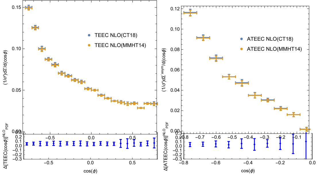
FIG. 2: Differential distribution 1/\sigma' d\Sigma'/d(\cos \phi) and its asymmetry 1/\sigma' d\Sigma'^{\text{asym}}/d(\cos \phi) , calculated in Next-to-Leading order for the low- Q^2 range 5.5 \text{ GeV}^2 < Q^2 < 80 \text{ GeV}^2 for the ep center-of-mass energy \sqrt{s} = 314 GeV at HERA. The two input PDFs are indicated on the upper frames. The lower frames show \Delta[\text{TEEC}(\cos \phi)]_{\text{PDF}} and \Delta[\text{ATEEC}(\cos \phi)]_{\text{PDF}} , defined in Eq. (15).
