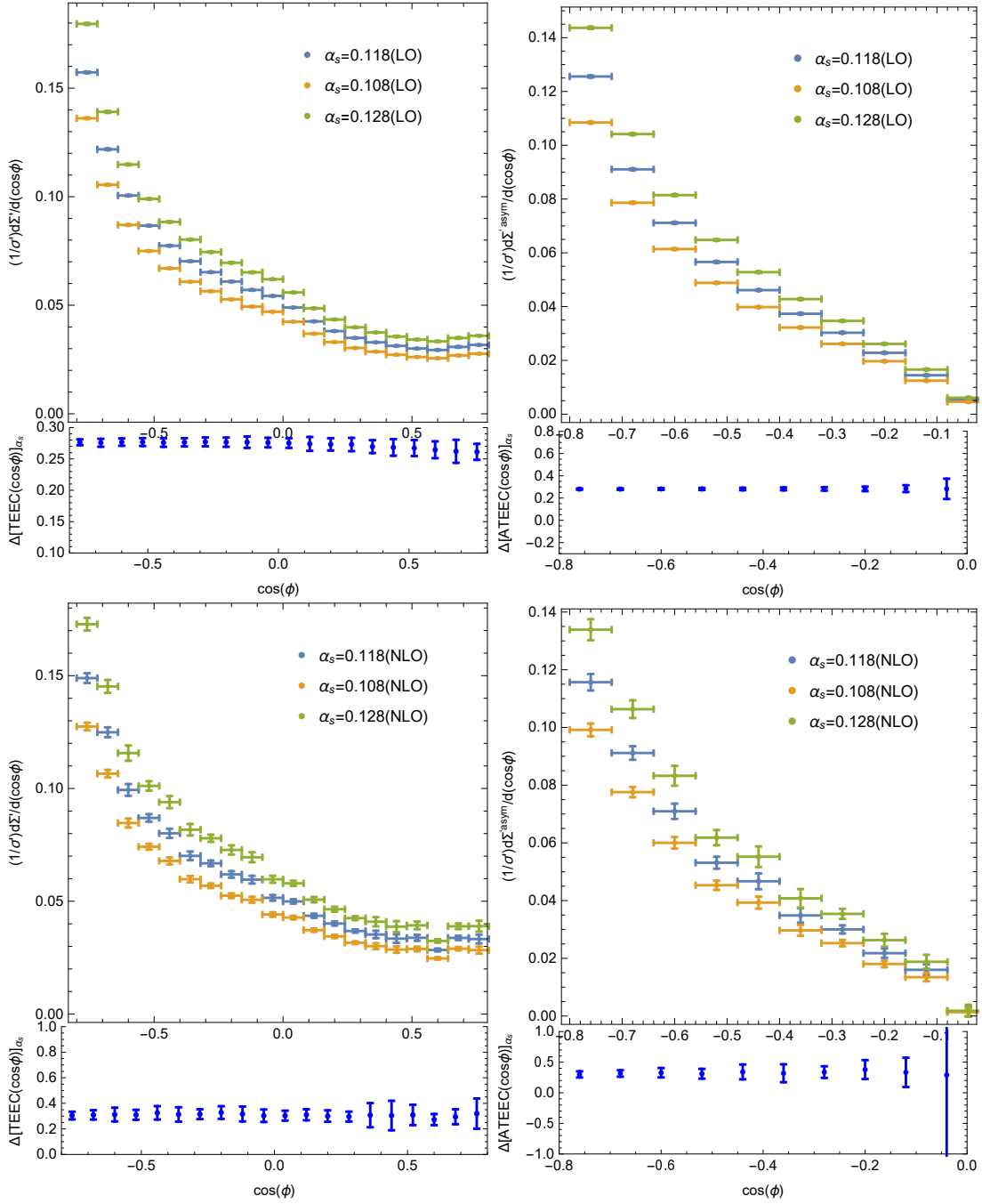
FIG. 8: Dependence of the differential distribution 1/\sigma' d\Sigma'/d(\cos\phi) (left) and its asymmetry 1/\sigma' d\Sigma'^{a,asym}/d(\cos\phi) (right) on the QCD coupling constant \alpha_s(M_Z) for three indicated values of \alpha_s(M_Z) = 0.108, 0.118, 0.128 using the PDFs of MMHT14 in the low- Q^2 range at HERA setting the scales \mu_F = \mu_R = \mu_0 .
