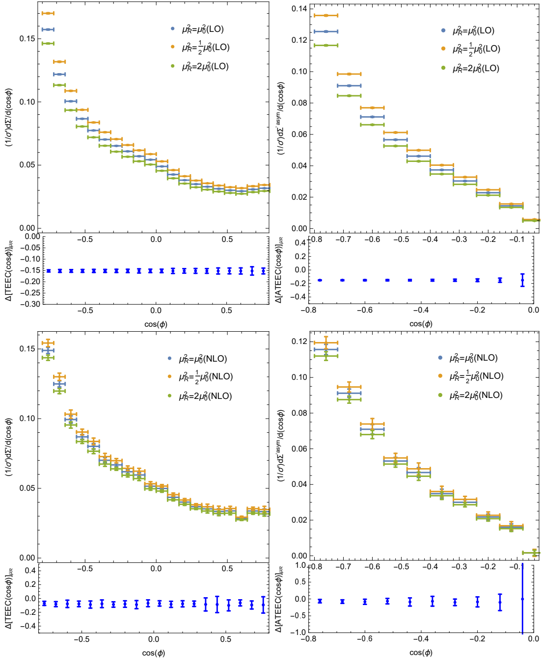
FIG. 6: Renormalization scale dependence of the differential distribution 1/\sigma' d\Sigma'/d(\cos\phi) and its asymmetry 1/\sigma' d\Sigma'^{asym}/d(\cos\phi) in the leading order (upper frames) and the next to leading order (lower frames) varying \mu_R^2 in the range [0.5, 2] \times \mu_0^2 , where \mu_0 is the nominal scale defined in the text, calculated with the MMHT14 PDFs for the low- Q^2 : 5.5 \text{ GeV}^2 < Q^2 < 80 \text{ GeV}^2 at HERA. The corresponding \mu_R -dependence is also shown in terms of \Delta[\text{TEEC}(\cos\phi)]_{\mu_R} and \Delta[\text{ATEEC}(\cos\phi)]_{\mu_R} , defined in Eq. (16).
