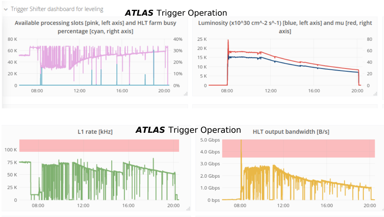
Figure 18: An example of a P-BEAST dashboard as used by the shifters during 2017 operation. The HLT farm availability (top left), the luminosity and the pile-up, ' \mu ' (top right), the total L1 accept rate (bottom left), and the total HLT output bandwidth (bottom right) are shown.
