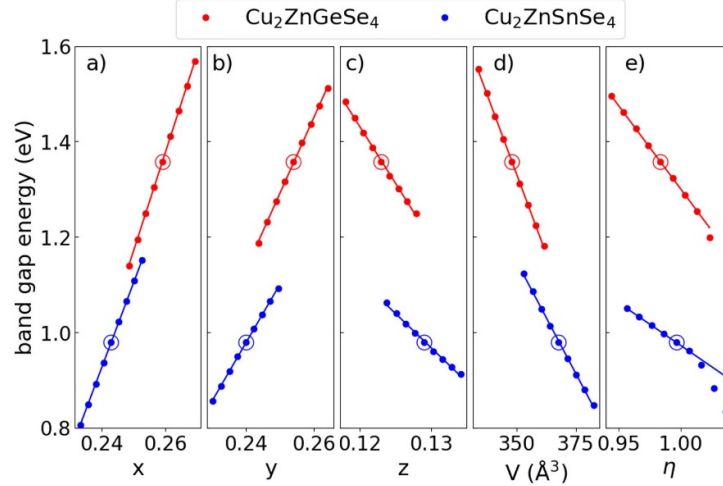
Figure 5. Band gap energies for \text{Cu}_2\text{ZnGeSe}_4 (red) and \text{Cu}_2\text{ZnSnSe}_4 (blue) from theoretical calculations as a function of anion position x (a), y (b) and z (c) and as a function of the unit cell volume V (d) and tetragonal distortion \eta = \frac{c}{2a} (e). The circles mark the experimental values derived from XRD measurements. Calculations were performed for deviations of \pm 4\% from these values. The red and blue lines are linear approximations of the respective data.
