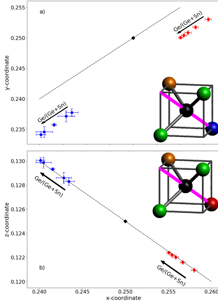
Figure 4. Projection of the relative anion position on the xy (a) and the xz plane (b) for the Ge (red) and Sn (blue) tetrahedron. The Ge content increases from right to left as indicated by the black arrows. The dashed line is the projection of the body diagonal of the quasi-cube spanned by the cations of the tetrahedron (thick magenta line in the inset images).
