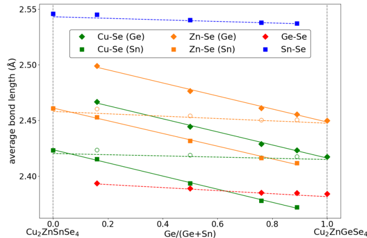
Figure 3. Modelled bond lengths for the tetrahedra containing Sn (squares) and Ge (diamonds) as a function of the Ge content. The individual bond lengths are depicted by full symbols while their weighted average is plotted as open symbols for Cu-Se and Zn-Se. The solid lines are linear fits of the Cu-Se and Zn-Se modelled bond lengths. The dashed lines represent the linear fits from figure 1.
