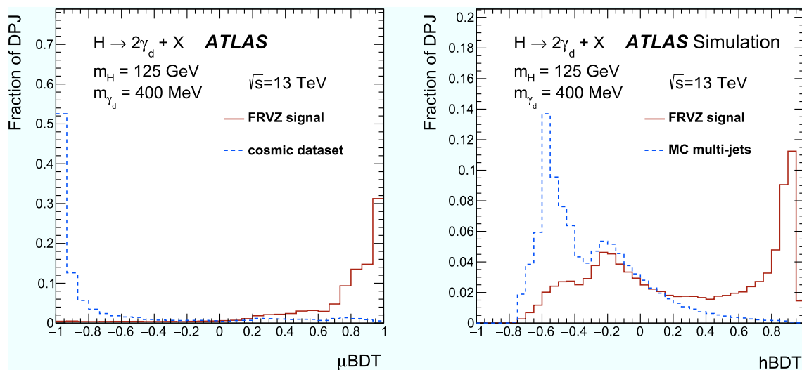
Fig. 2 BDT output distributions for signal and background for \mu DPJs (left) and hDPJs (right). For muonic-DPJs the background is the cosmic dataset and the FRVZ signal sample is the H \rightarrow 2\gamma_d + X process
