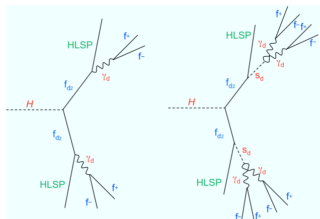
Fig. 1 The two processes of the FRVZ model used as benchmarks in the analysis. In the first process (left), the dark fermion f_{d2} decays into a \gamma_d and an HLSP. In the second process (right), the dark fermion f_{d2} decays into an HLSP and a dark scalar s_d that in turn decays into a pair of dark photons. The \gamma_d decays into SM fermions, denoted by f^+ and f^-
