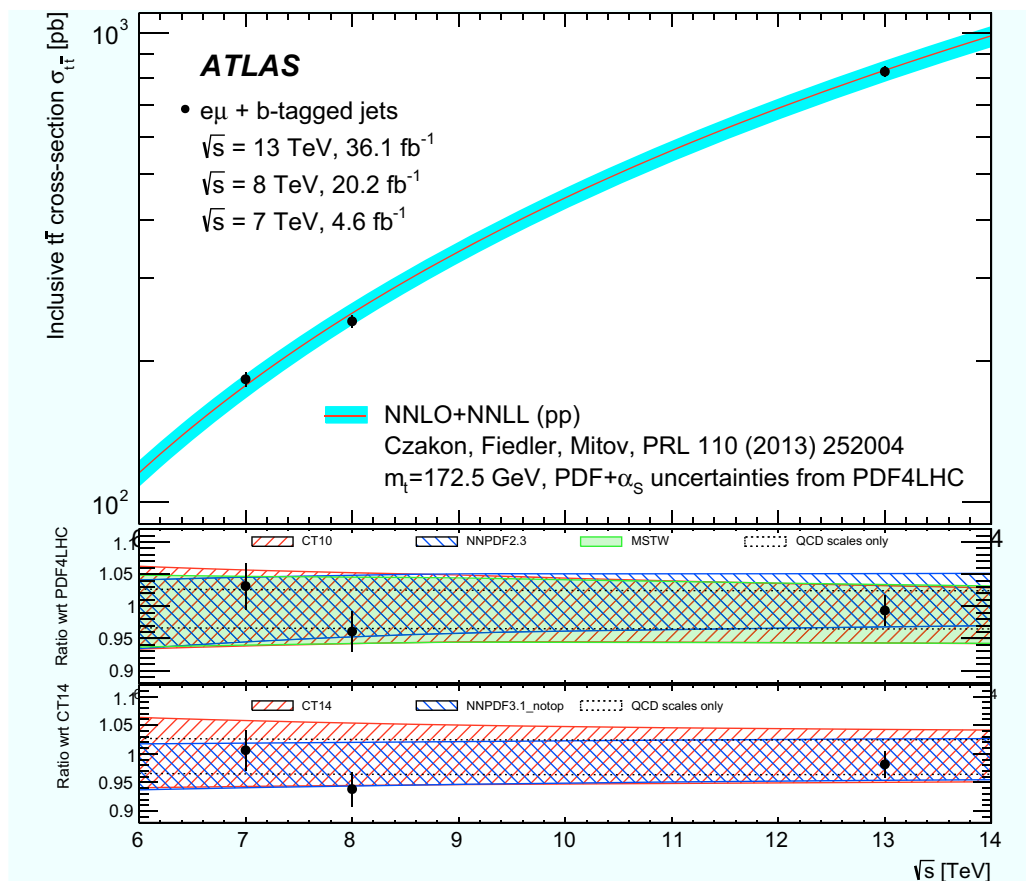
Fig. 8 The upper plot shows the inclusive t\bar{t} cross-section \sigma_{t\bar{t}} as a function of centre-of-mass energy \sqrt{s} , comparing ATLAS results from the e\mu plus b -tagged jets final state at \sqrt{s} = 7, 8 and 13 TeV with NNLO+NNLL theoretical predictions [5] calculated using Top++ [14] using the PDF4LHC prescription for PDF and \alpha_s uncertainties [15], and m_t = 172.5 GeV. The middle plot shows the ratios of the measurements and predictions to the central value of the prediction using PDF4LHC.
