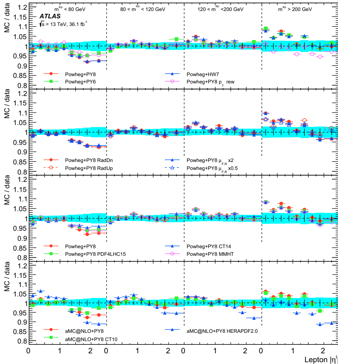
Fig. 20 Ratios of predictions of the normalised double-differential cross-sections to data as a function of |\eta^\ell| and m^{e\mu} . The data statistical uncertainties are shown by the black error bars around a ratio of unity, and the total uncertainties are shown by the cyan bands. The
