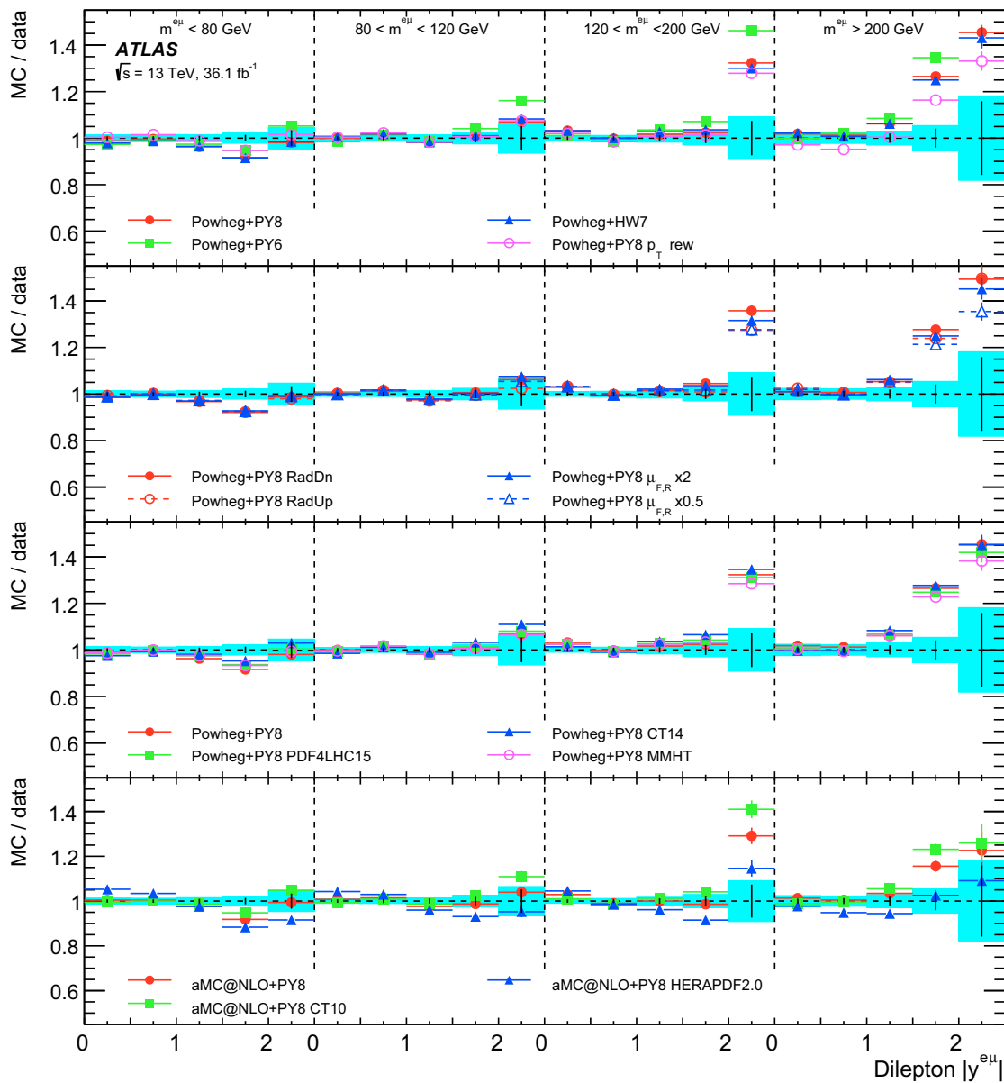
Fig. 21 Ratios of predictions of the normalised double-differential cross-sections to data as a function of |y^{e\mu}| and m^{e\mu} . The data statistical uncertainties are shown by the black error bars around a ratio of unity, and the total uncertainties are shown by the cyan bands. The
