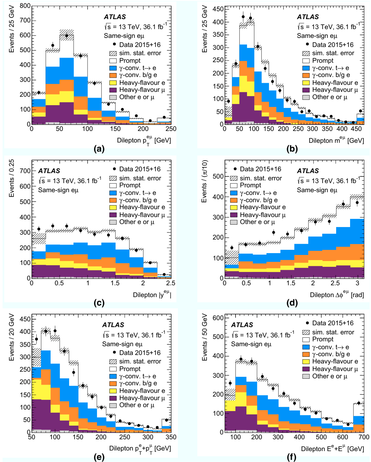
Fig. 4 Distributions of a the dilepton p_T^{e\mu} , b invariant mass m^{e\mu} , c rapidity |y^{e\mu}| , d azimuthal angle difference \Delta\phi^{e\mu} , e lepton p_T sum p_T^e + p_T^\mu and f lepton energy sum E^e + E^\mu , in events with a same-sign e\mu pair and at least one b -tagged jet. The simulation prediction is normalised to the same integrated luminosity as the data, and broken down into contributions where both leptons are prompt, or one is
