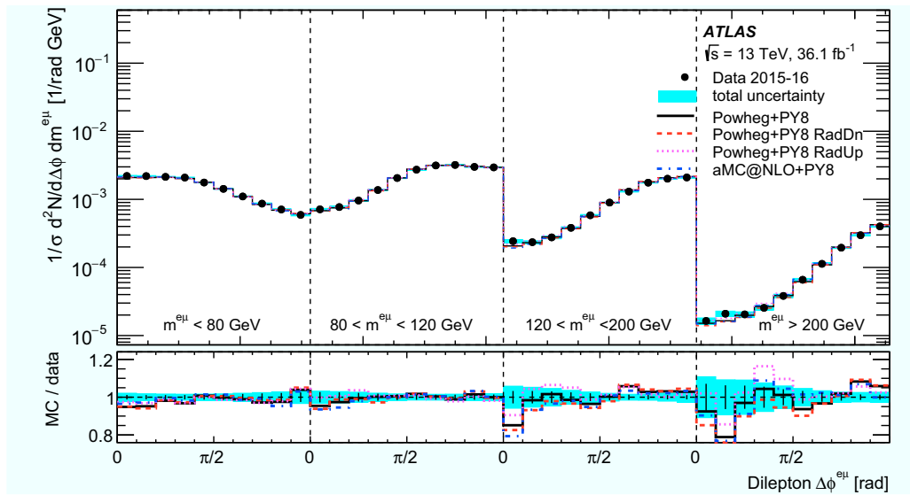
Fig. 15 Normalised double-differential cross-sections as a function of \Delta\phi^{e\mu} and m^{e\mu} . The measured values are shown by the black points with error bars corresponding to the data statistical uncertainties and cyan bands corresponding to the total uncertainties in each bin, and include the contributions via W \rightarrow \tau \rightarrow e/\mu decays. The data points are placed at the centre of each bin. The results are compared with the
