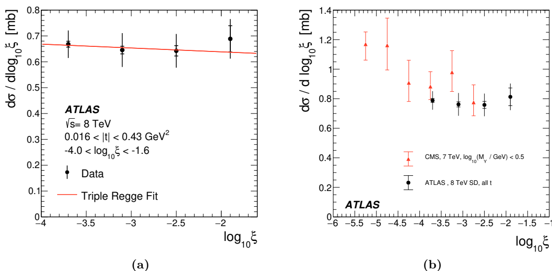
Figure 5. The differential cross section as a function of \log_{10}\xi . (a) Data in the fiducial t range, compared with the results of the triple Regge fit described in the text. (b) ATLAS data extrapolated to the full t range, compared with a rapidity-gap-based CMS measurement [15] that contains a small DD admixture (see text). The inner error bars represent only statistical uncertainties while the outer error bars display the combination of statistical and systematic uncertainties in quadrature.
