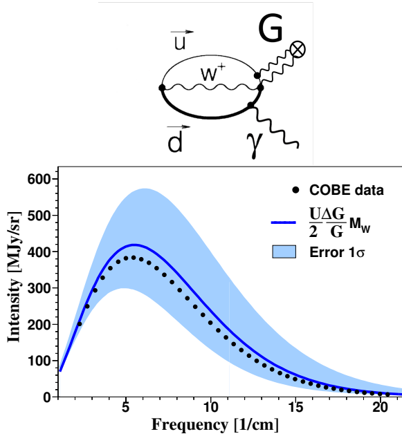
FIG. 2. Diagram of QCD vacuum decay process (upper part) induced by chiral gravitation. Gravitational parity violation measurement fitted to the Cosmic Microwave Background spectrum (lower part).
