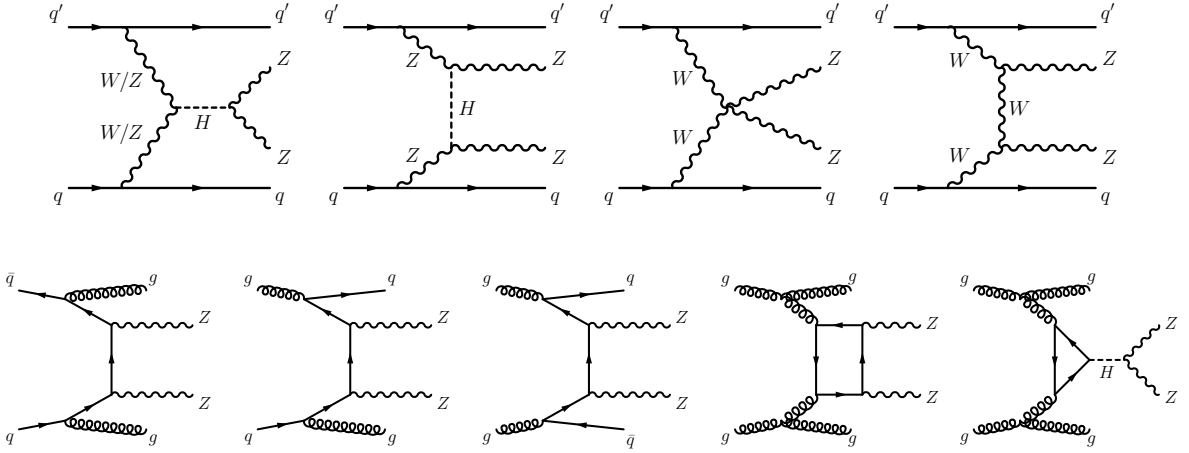
Figure 1: Typical diagrams for the production of ZZjj , including the relevant EW VBS diagrams (first row) and QCD diagrams (second row).
