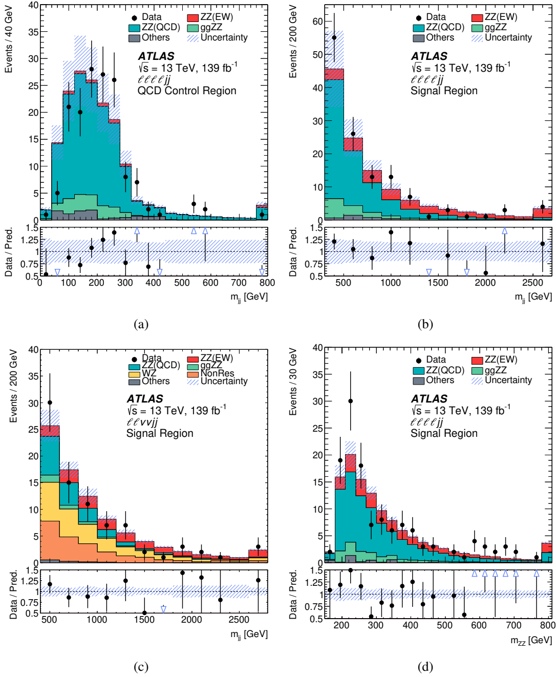
Figure 2: Observed and expected m_{jj} distributions in the (a) lllljj QCD CR and the (b) lllljj and (c) llvvjj signal regions, as well as the m_{zz} distribution in the (d) lllljj signal region. The error bands include the expected experimental and theoretical uncertainties. The contributions from the QCD and EW production of ZZjj events are scaled by 0.96 and 1.35, respectively, which correspond to the observed normalisation factors in the statistical fit to the combined channel (Table 2). All the minor backgrounds are summed together as ‘Others’. The last bin includes the overflow events. The open arrows represent the out-of-range markers.
