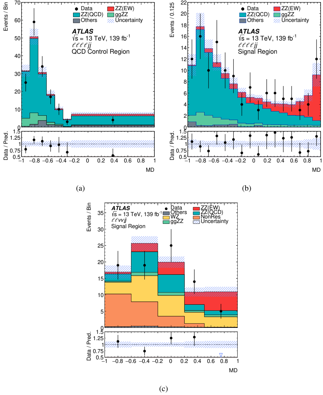
Figure 3: Observed and expected multivariate discriminant distributions after the statistical fit in the (a) lllljj QCD CR, and in the (b) lllljj and (c) llvvjj signal regions. The error bands include the experimental and theoretical uncertainties, as well as the uncertainties in \mu_{EW} and \mu_{QCD}^{lllljj} . All the minor backgrounds are summed together as ‘Others’. The statistical uncertainties of the data are shown as error bars. The open arrows represent the out-of-range markers.
