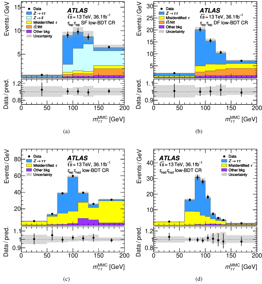
Fig. 3. Post-fit m_{\tau\tau}^{\text{MMC}} distributions in the low- \text{BDT}_{\text{score}} CR for the (a) \tau_{\text{lep}}\tau_{\text{lep}} SF, (b) \tau_{\text{lep}}\tau_{\text{lep}} DF, (c) \tau_{\text{lep}}\tau_{\text{had}} and (d) \tau_{\text{had}}\tau_{\text{had}} analysis channels. The ratios of the data to the prediction are shown in the lower panels. The contamination of the CR by signal is negligible. “Other bkg” denotes all background contributions not listed explicitly in the legend. The size of the combined statistical, experimental, and theoretical uncertainties in the background is indicated by the hatched bands. The rightmost bins in each of the subfigures include event yields with m_{\tau\tau}^{\text{MMC}} values larger than the shown range.
