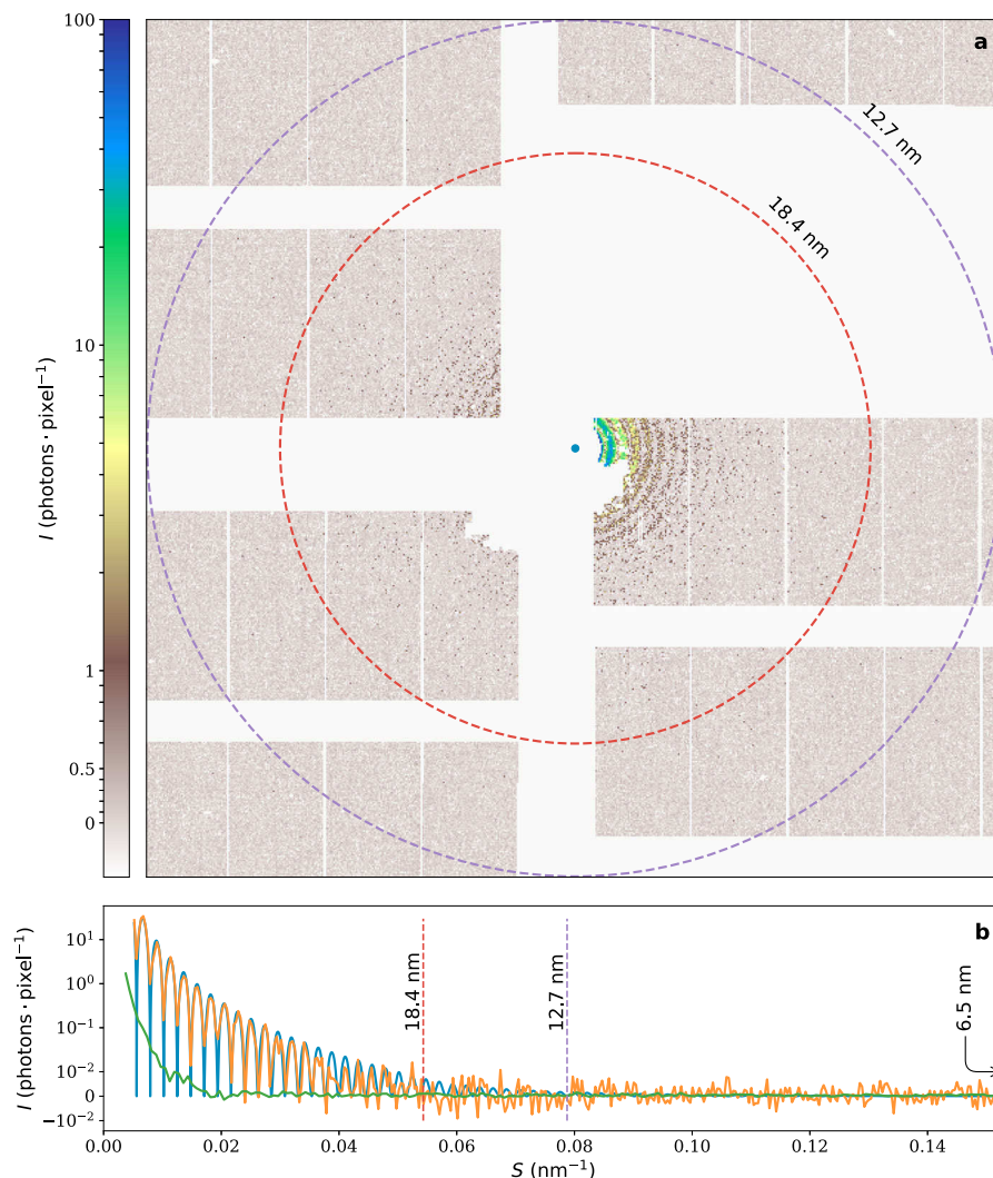
Fig. 5 Comparison of signal with background for a single diffraction pattern. a Single strong diffraction pattern of an \text{IrCl}_3 sphere of 439 nm in diameter, cropped to an edge resolution of 12.7 nm. b Comparison between the radially averaged scattering of the \text{IrCl}_3 sphere (orange), fitted model (blue), and radially averaged background with injection (green). Note that the scale is linear below 10^{-2} photons per pixel. The red dashed lines (18.4 nm resolution) mark the angle at which the modeled scattering is stronger than the noise in a single frame; the purple dashed lines (12.7 nm resolution) mark the angle where the modeled scattering exceeds an average background; detector edge resolution is 6.5 nm.
