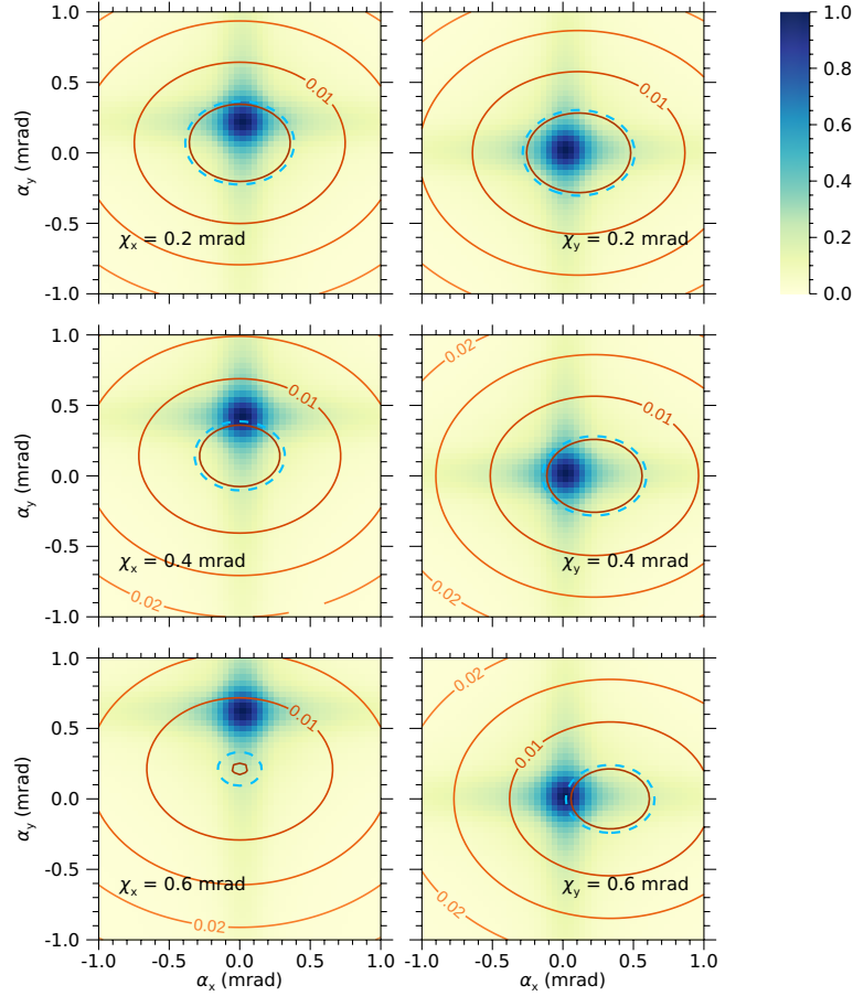
Figure 13. Field maps (in false colour) of the transmission of a system of misaligned crossed flat MLLs of NA = 0.0375 and focal lengths f_1 = 1.25 mm and f_2 = 1 mm, for various rotations \chi_x and \chi_y of the first lens relative to the second. Contour maps of the RMS aberrations are superimposed, with the Marechal condition indicated by the dashed sky-blue line.
