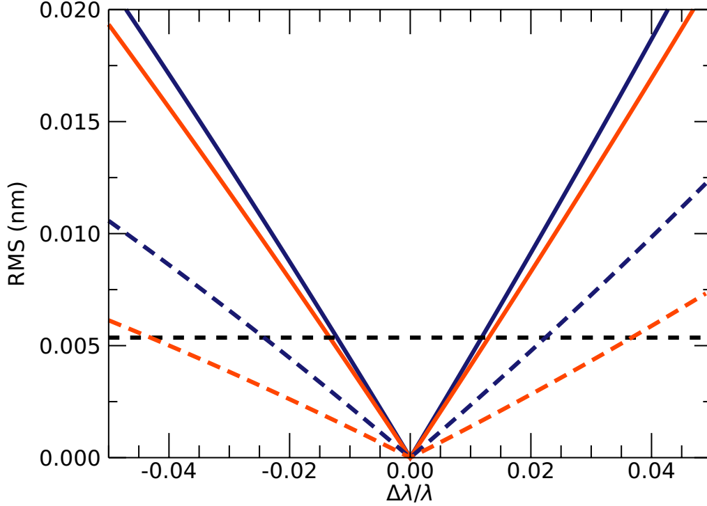
Figure 11. RMS wavefront aberration (excluding defocus and astigmatism) of crossed MLLs of \text{NA} = 0.0375 , f_1 = 1.25 \text{ mm} and f_2 = 1 \text{ mm} as a function of the relative deviation of the wavelength from the design for curved lenses ( R_1 = f_1 and R_2 = f_2 ) (orange) and flat lenses ( R_1 = \infty and R_2 = \infty ) (blue). The solid lines assume a corrector with a phase profile that is independent of wavelength and the dashed lines are for a phase corrector made of carbon. The Marechal condition of \lambda/14 is indicated by the black dashed line.
