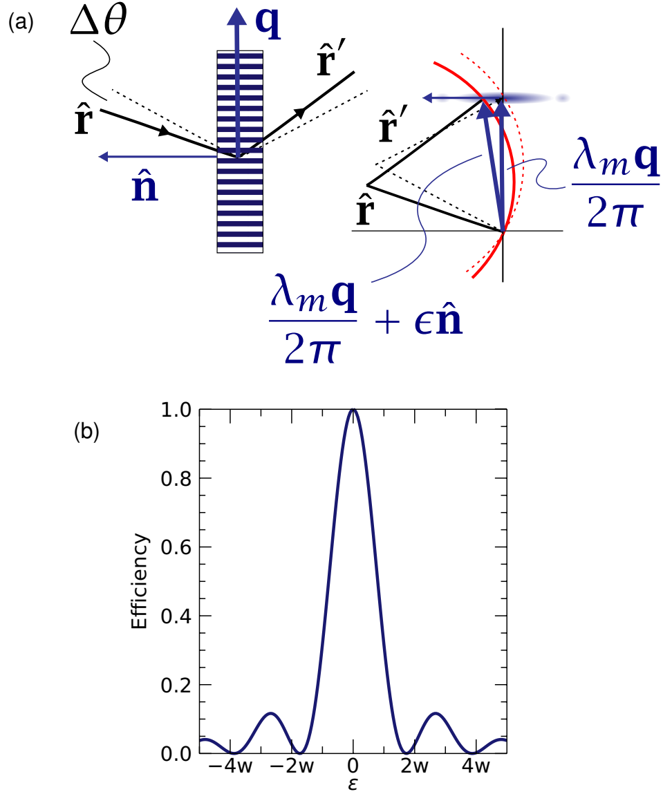
Figure 2. (a) The off-Bragg reflection from a periodic multilayer in Laue geometry shown in real space to to left is found from the reciprocal-space Ewald sphere construction at right, considering that the diffraction peak lies along a truncation rod normal to the surface. (b) Rocking curve of a multilayer reflecting in a Laue geometry with an optimum thickness and neglecting absorption, as a function of the deviation parameter \epsilon \approx \Delta\theta \lambda_m |\mathbf{q}| / (2\pi) and for a width w_\epsilon .
