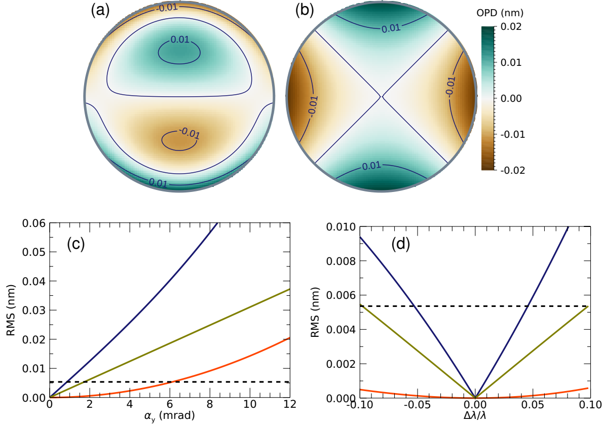
Figure 4. Wavefront errors (excluding defocus) of axisymmetric lenses with \text{NA} = 0.0375 and a focal length f = 1 mm and (a) a flat surface R = \infty at a field angle \alpha_y = 1 mrad and (b) a spherical surface with R = f at a field angle \alpha_y = 7.5 mrad. (c) Plot of the RMS errors as a function of field angle for R = \infty (blue), R = (2/3)f (olive green) and R = f (red). (d) RMS error as a function of the relative wavelength deviation from the design, where \Delta\lambda = \lambda_m - \lambda , and for R = \infty (blue), R = (2/3)f (olive green) and R = f (red). The Marechal condition of \lambda/14 is shown by the dashed line for a wavelength of 0.075 nm. The wavefront magnitude scales proportionally with the focal length f .
