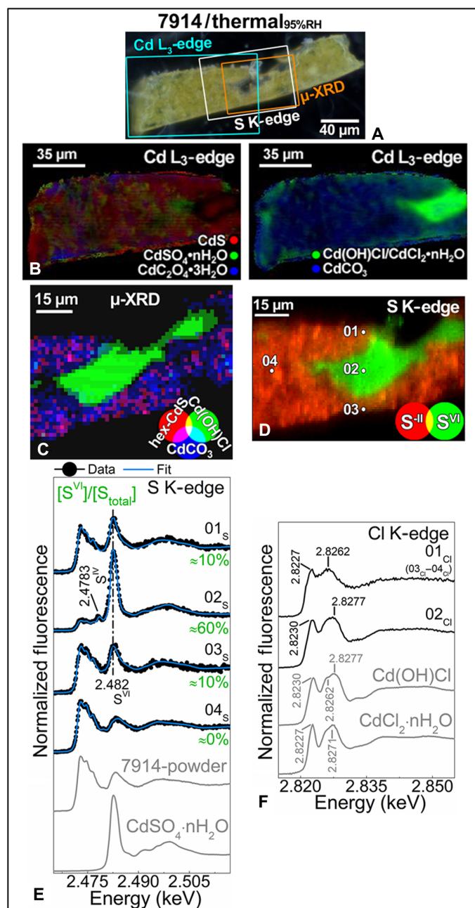
Fig. 6. Artificially aged 7914 mock-up. (A) Photomicrograph of 7914 thin section after thermal aging (RH \geq 95%, T = 40°C, 90 days). (B) Quantitative Cd phase images obtained from the LCF of the full-field (FF)-XANES stack using the profiles of CdS (red), CdSO 4 ·nH 2 O/(Cd,Cl) chlorides (green), and CdC 2 O 4 ·3H 2 O/CdCO 3 (blue). RGB composite (C) SR \mu -XRD images of hex-CdS/Cd(OH)Cl/CdCO 3 [step size (h \times v), 1.5 \times 1.5 \mu m 2 ; exp. time, 1 s per pixel; energy, 21 keV] and (D) SR \mu -XRF maps of S II /S VI [step size (h \times v), 1 \times 1 \mu m 2 ; exp. time, 100 ms per pixel] acquired from the regions shown in (A). Selection of \mu -XANES spectra at (E) S K-edge and (F) Cl K-edge obtained from the points indicated in (D) and LCF results (cyan) of different S-based reference compounds. In (E) and (F), the spectral profiles of selected reference compounds are reported in gray color for comparison, whereas numbers in brackets refer to the spectra showing similar features to those reported (see figs. S3 to S5 and table S1 for additional results).
