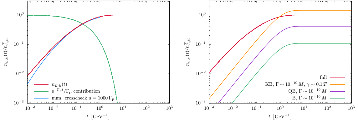
Figure 9. Time evolution of the lepton number density. Left: Full result obtained by different orders of integration (see text). The green curve gives the time-dependent contribution. Right: Comparison of the full result with Boltzmann (B), quantum Boltzmann (QB) and Kadanoff-Baym (KB) computations, where gauge corrections are not computed but parametrised by thermal widths.
