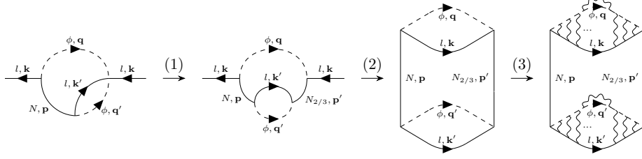
Figure 6. Transformation of the lepton self-energy diagram to a form amenable to resummation.
