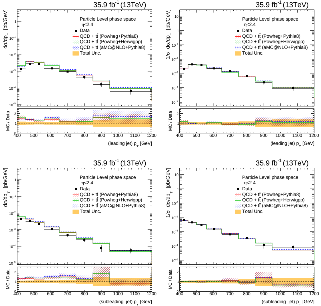
Figure 11.9: Cross section (left plots) and normalized distributions (right plots) differentially in (upper plots) the p_T of the leading jet, (lower plots), the p_T of the subleading jets, compared to theory predictions. The total uncertainty are shown for each measurements in the lower panels, while in the upper panels only the statistical uncertainties are shown. The shown uncertainty in the theory predictions are the statistical uncertainties. The distributions correspond to the inclusive top-jet cross section.
