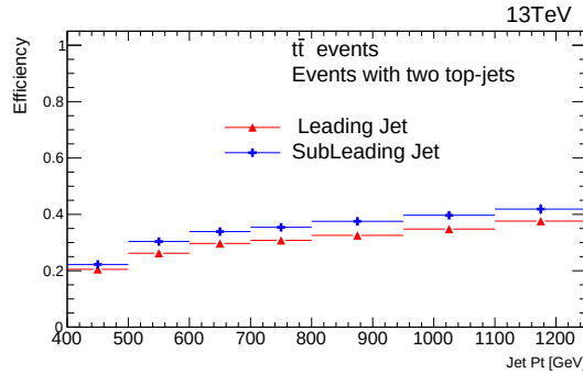
Figure 6.6: Selection efficiency as a function of p_T for leading and subleading jets, after applying the top-jet selection criteria. The efficiency is estimated with respect of the events selected by the boosted-dijet criteria.
