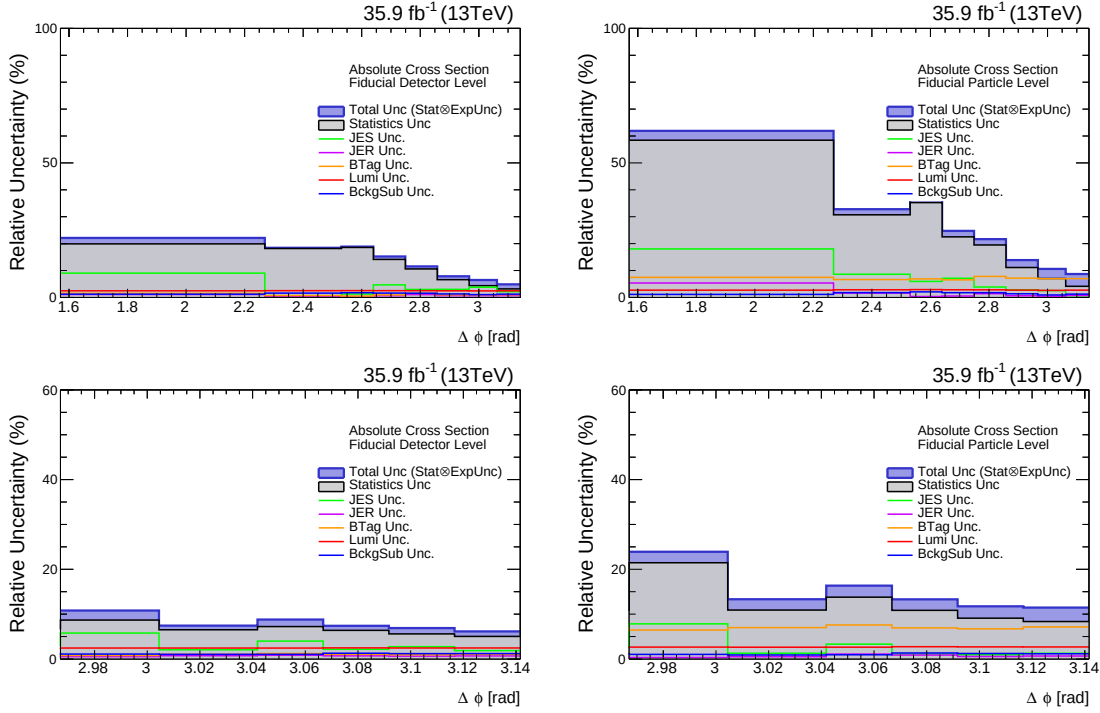
Figure 10.4: Breakdown of the experimental systematic uncertainties of the cross section measurements differential in \Delta\phi in the whole phase space (upper plots) and in \Delta\phi in the most back to back region (lower plots) at: detector level (left plots) and particle level (right plots). The plots correspond to the measurements of the t\bar{t} cross section.
