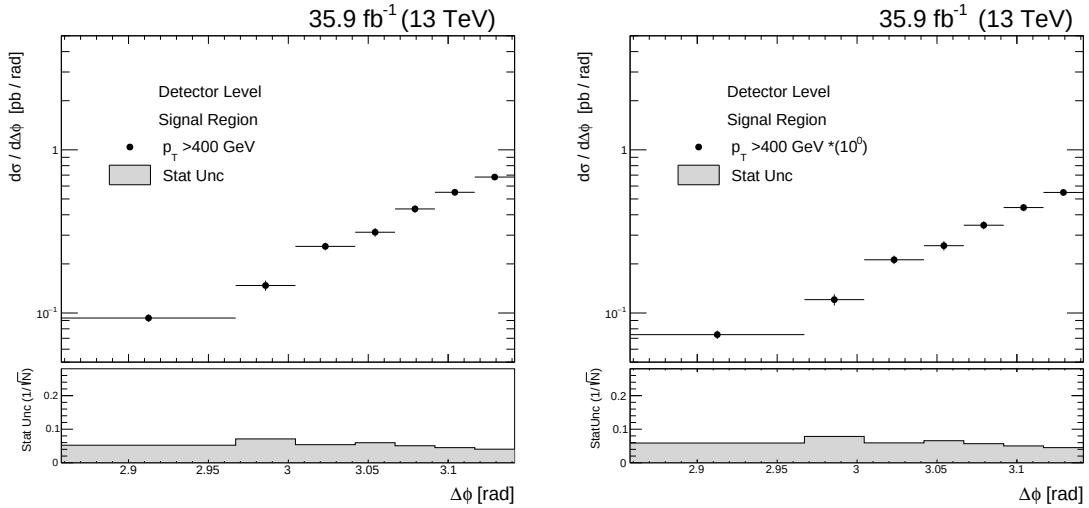
Figure 8.4: Absolute cross section in the fiducial phase space (detector level) differential in the azimuthal separation between the two leading jets \Delta\phi : (left) inclusive top jet measurements (right) t\bar{t} measurements . The fine binning in the most back-to-back region is considered.
