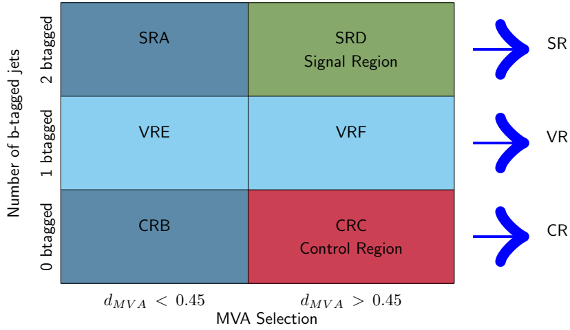
Figure 8.5: Schematic picture of different regions defined by using the multivariate selection and the b-tagging requirements. A base-line selection is previously assumed: the boosted dijet selection and the top jet selection. The Signal Region (SRD) is represented in green color, while the Control Region (CRC) is represented in red color.
