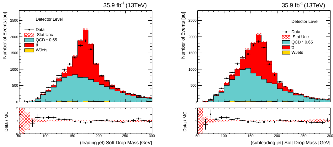
Figure 6.9: Data distributions representing the number of events as a function of the soft drop jet mass for: (left) leading jet, (right) subleading jet. The data are compared to simulated signal ( t\bar{t} ) and background (QCD multijet, W+Jets) contributions. Events are selected by requiring the boosted dijet selection, the top-jet selection, and the b-tagging selection criteria.
