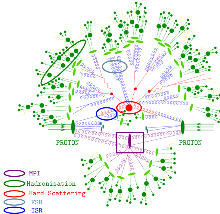
Figure 1.5: (figure modified from [33]) Schematic picture of a hadronic p - p collision and the subsequent interactions considered in a Monte Carlo event simulations.
