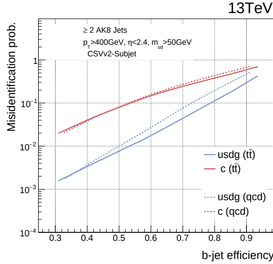
Figure E.2: b -tagging efficiency performance for the CSVv2 algorithm applied to the subsets obtained by the Soft Drop Mass mechanism in simulated t\bar{t} and QCD events with two Ak8 jets with p_t > 400\text{ GeV} , |\eta| < 2.4 and m_j^{sd} > 50\text{ GeV} .
