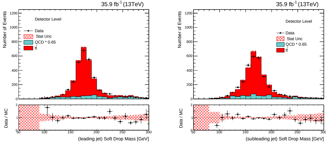
Figure 7.10: Data distributions representing the number of events as a function of the soft drop jet mass for: (left) leading jet, (right) subleading jet. The data are compared to simulated signal ( t\bar{t} ) and background (QCD multijet) contributions. Events are selected by requiring the boosted dijet selection, the top-jet selection, the MVA selection and the b-tagging selection criteria.
