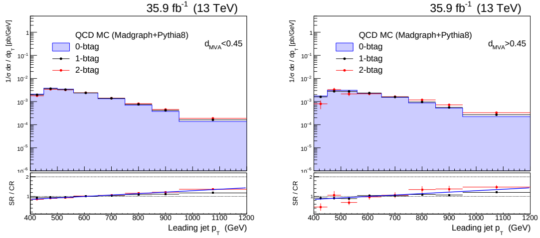
Figure 8.11: Transfer function with respect to the p_T of the leading jet (right) when d_{MVA} < 0.45 (left) when d_{MVA} > 0.45 . The plot at the left give the ratio of the distributions between, i.e SR and CRB , while the plot at the right corresponds to the ratio between the distributions in SRD and CRC .
