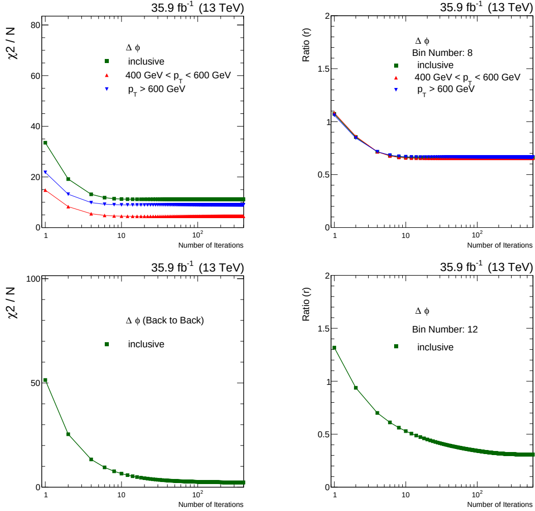
Figure 9.9: (left) \chi^2 (9.23) distribution and (right) r (9.24) distributions as function of the number of iterations of the unfolding procedure for \Delta\phi spectra. The whole \Delta\phi phase space (upper plots), and a fine binning in the most back-to-back region (lower plots) are illustrated. For the plots, the inclusive fiducial phase space and exclusive regions defined by the p_T^{lead} are considered.
