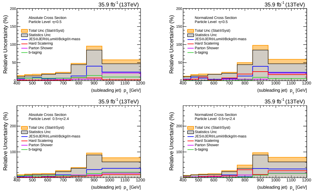
Figure H.3: Systematic and statistical uncertainty corresponding to the distributions differential in p_T of the subleading jet in two different \eta regions: |\eta| < 0.5 (upper plots) and 0.5 < |\eta| < 2.4 (lower plots). The systematic uncertainty corresponding to the absolute (left) and normalized (right) distributions are illustrated.
