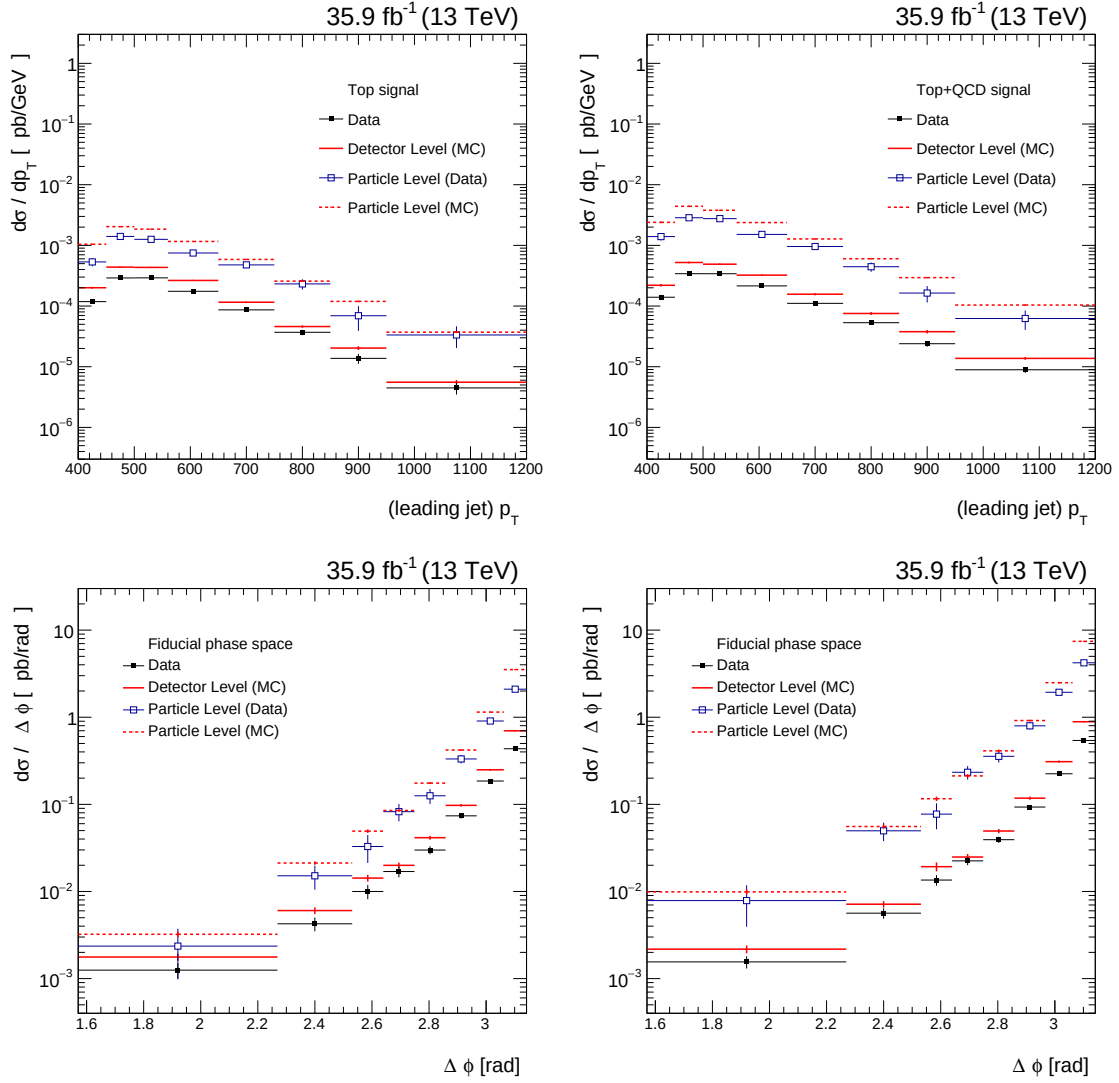
Figure 9.1: Monte Carlo and data comparison at particle and detector level, for (left) t\bar{t} measurements, (right) inclusive top jet measurements. The unfolded distributions have been estimated with the iterative D’Agostini method [168]
