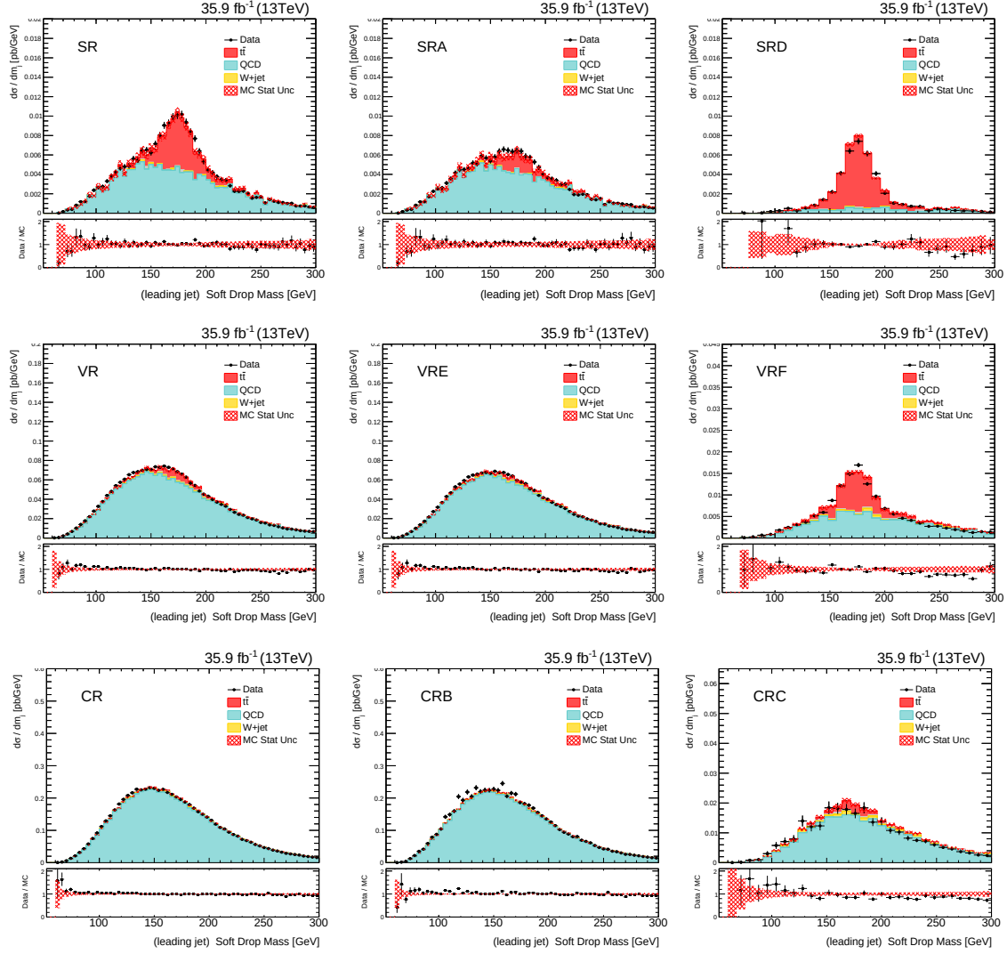
Figure 8.6: Soft Drop Mass distributions for the leading jet in different regions defined in Figure 8.5. The normalization factor for the t\bar{t} contribution has been taken as N_{t\bar{t}} = 0.654 , while for the QCD multijet contribution: N_{QCD} = 0.74 in the first row (2-btagged jets), N_{QCD} = 0.67 in the second row (exclusively 1-btagged jet), N_{QCD} = 0.6 in the third row (zero btagged jet).
