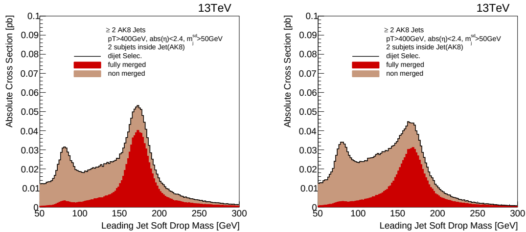
Figure D.1: Soft Drop jet mass distributions in t\bar{t} events considering two categories: fully merged and non-merged. Fully merged refers to the condition that the jet is classified as b -flavour jet with the additional requirement that \tau_{32} < 0.7 , while the non-merged sample are the remaining jets. The (left) leading jet, and (right) subleading jet are considered separately.
