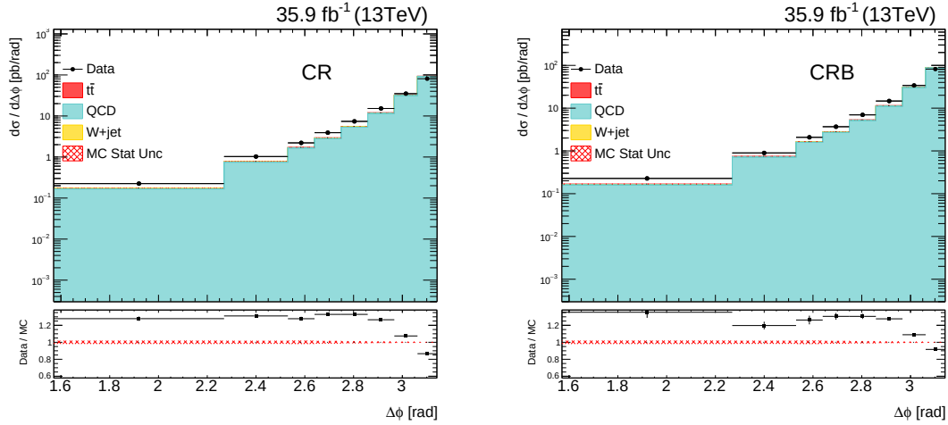
Figure 8.7: Comparison of the \Delta\phi distribution in data with the Monte Carlo predictions in two different regions (left) CR (right) CRB. The only non-negligible contribution in this region is the QCD multijet events.
