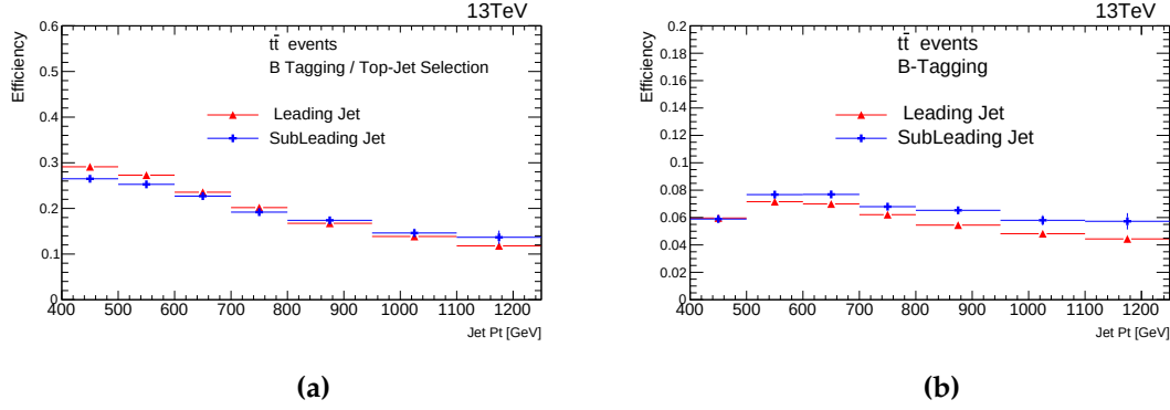
Figure 6.10: Efficiency selection as a function of p_T of the leading and subleading jets after the b-tagging selection criteria: (a) with respect of the events selected after top-jet selection (b) with respect to the boosted-dijet selection.
