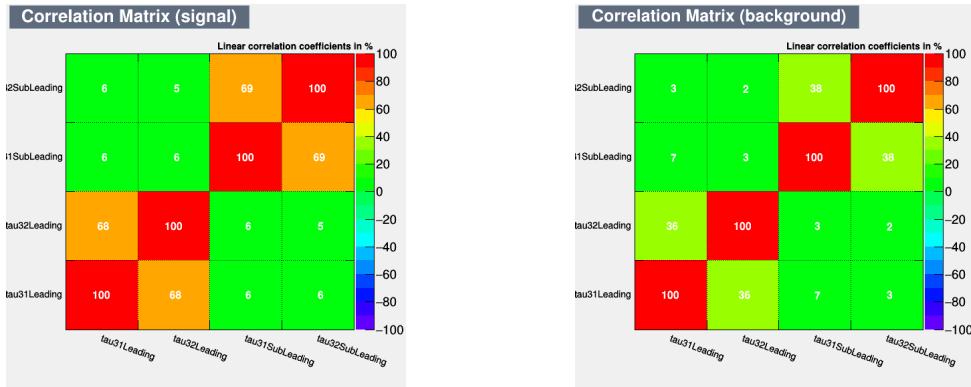
Figure 7.5: Linear correlation of the four substructures variables provided as input information for the MVA algorithm for: (left) signal events, (right) background events. The symbols \tau_{31} and \tau_{32} mean the ratio \tau_3/\tau_1 and \tau_3/\tau_2 respectively.
