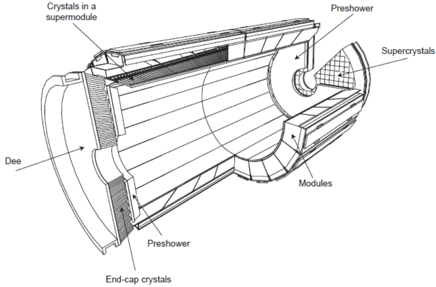
Figure 4.6: (taken from [117]) Sketch showing the Electromagnetic calorimeter (ECAL), the part of the detector responsible to measure the energy of the electrons and photons.
