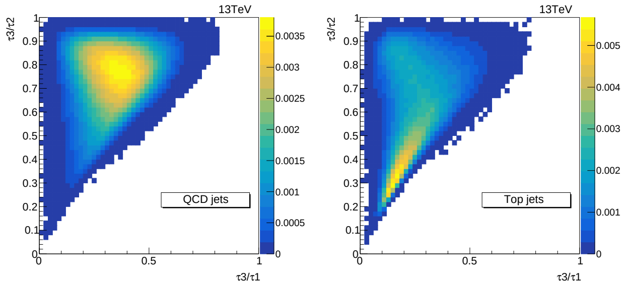
Figure 3.5: Correlation between N -subjettiness variables ( \tau_3/\tau_1 and \tau_3/\tau_2 ) in (left) QCD jets (right) top jets. Distributions correspond to the particle level after applying the boosted selection.
