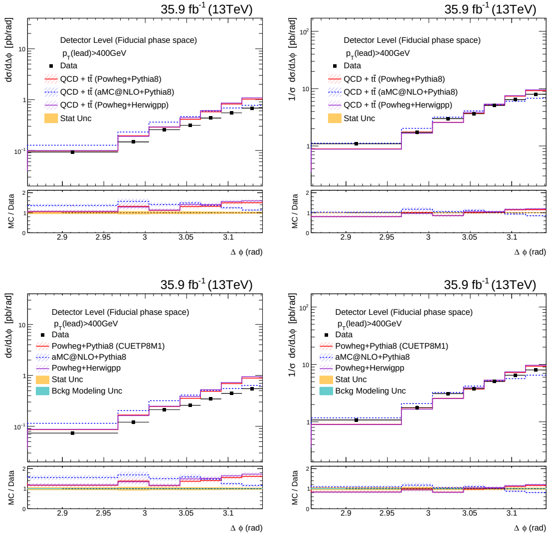
Figure 8.19: Measurements in the inclusive fiducial phase space differential in \Delta\phi : (left) cross section (right) normalized distribution, (upper plots) corresponding to the inclusive top jet measurements (lower plots) and to the t\bar{t} measurements. The plots correspond when a fine binning is considered in the most back-to-back region. The data points in the upper panel only include the statistical uncertainties.
