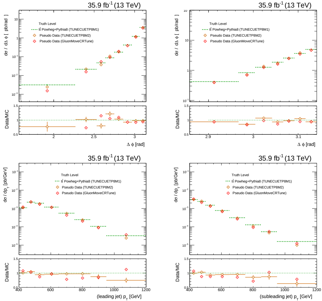
Figure G.2: Comparison of the Monte Carlo predictions and the unfolded pseudo-data at stable level (truth level). The unfolded procedure is implemented using different Monte Carlo samples for the input information. The following observables are illustrated: (upper left) the \Delta\phi observable in the whole azimuthal phase space, (upper right) the \Delta\phi observable in the most back-to-back region, (down left) the p_T of the leading jet, (down right) the p_T of the subleading jet.
