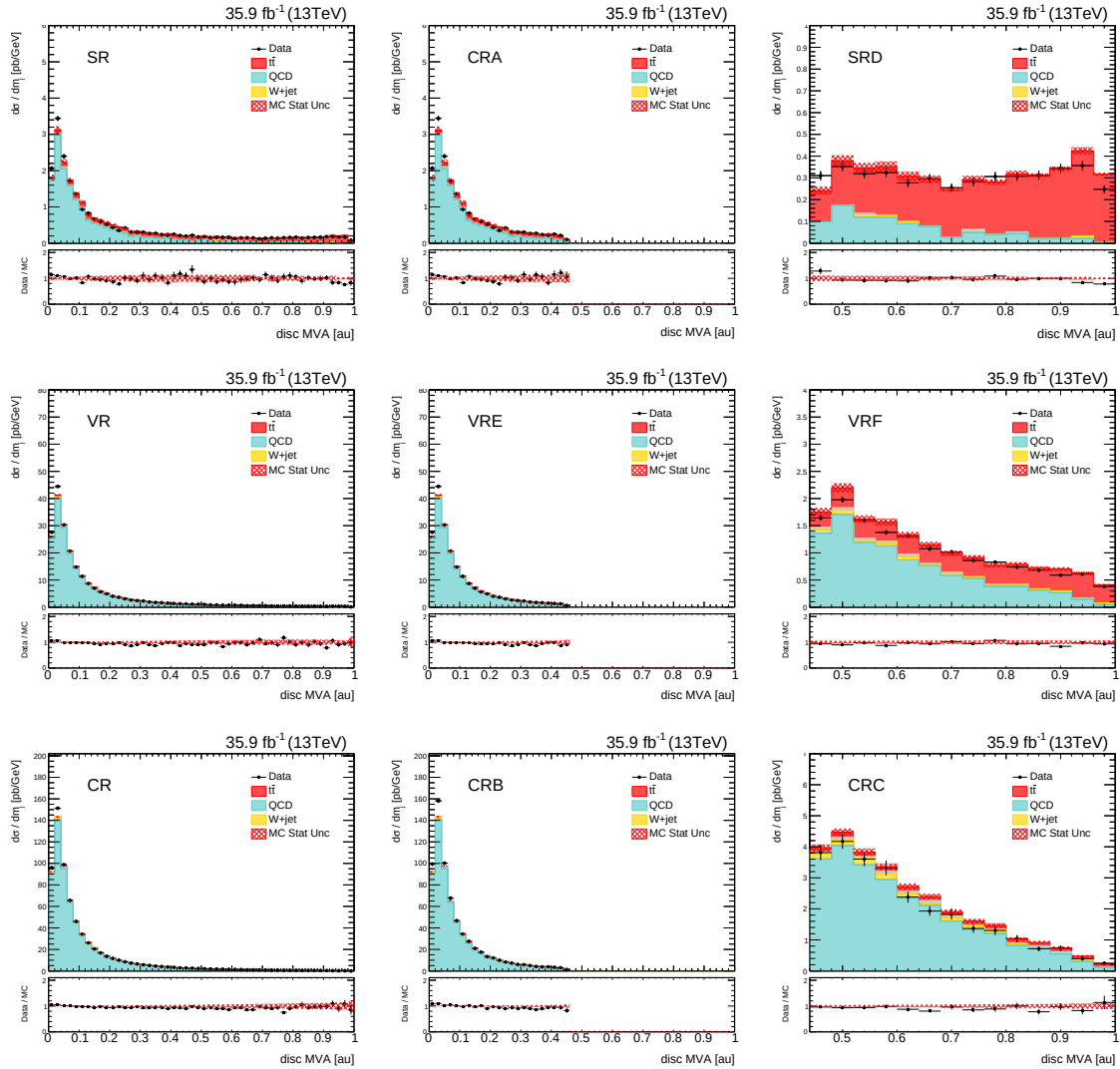
Figure F.1: d_{MVA} distributions for the leading jet in different regions defined in Figure 8.5. The normalization factor for the t\bar{t} contribution has been taken as N_{t\bar{t}} = 0.654 , while for the QCD multijet contribution: N_{QCD} = 0.74 in the first row (2-btagged jets), N_{QCD} = 0.67 in the second row (exclusively 1-btagged jet), N_{QCD} = 0.6 in the third row (zero btagged jet).
