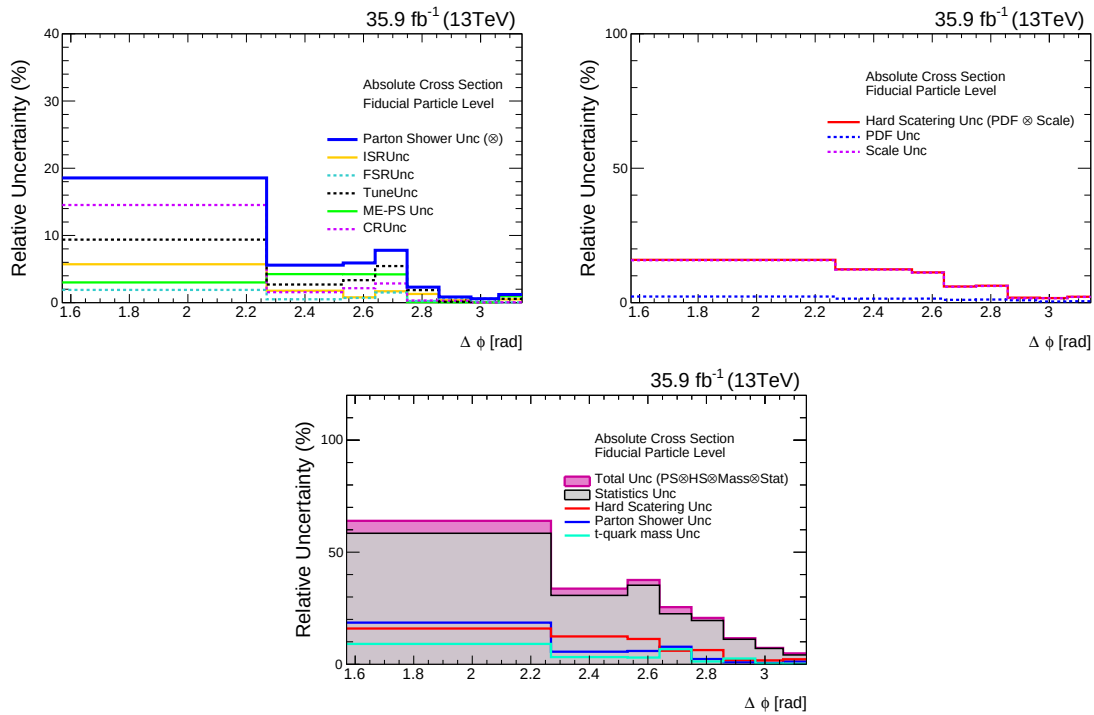
Figure 10.6: Breakdown of the relative systematic uncertainties of the cross section measurements differential in \Delta\phi : (upper-left plot) the Parton Shower modeling uncertainties, (upper-right) the Hard Scattering modeling uncertainties, (lower plot) the total uncertainties counting the modeling and the statistical uncertainties
