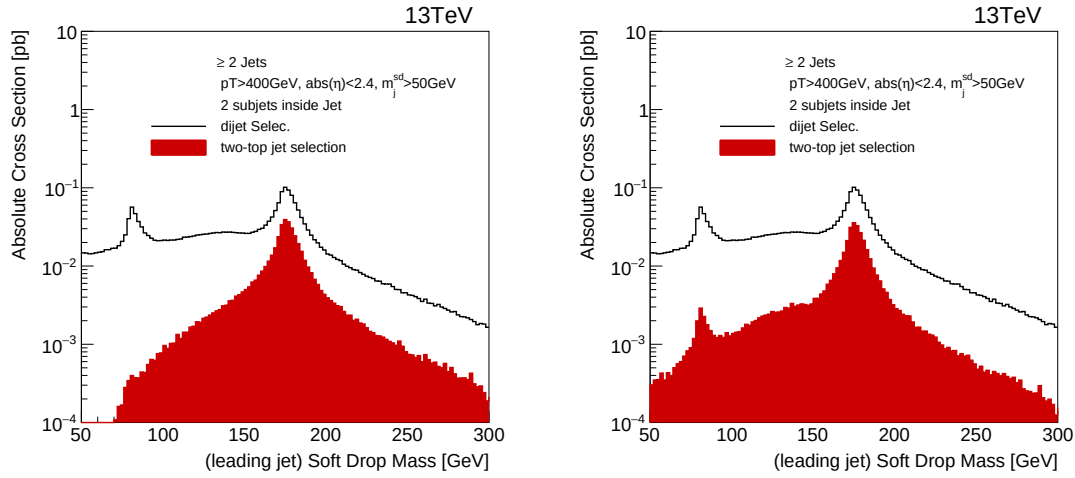
Figure C.5: Soft Drop jet mass distribution corresponding to the leading jet in simulated t\bar{t} events. First, the events are selected with the boosted dijet selection criteria, and secondly by requiring two top jets using: the definition A (left plot), the definition B (right plot) provided in Table C.1
