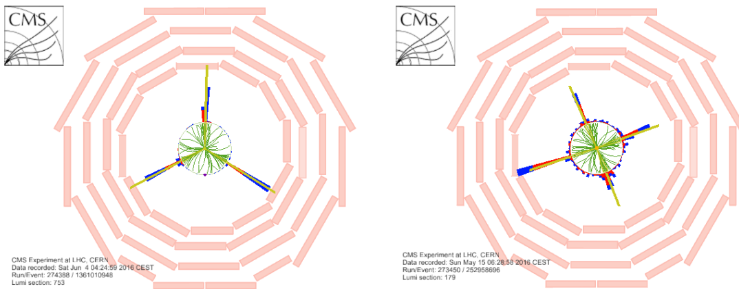
Figure 2.4: (taken from [86]) Display of events recorded by the CMS experiment in 2016 (left) for three jet topology and (right) for four jet topology.
