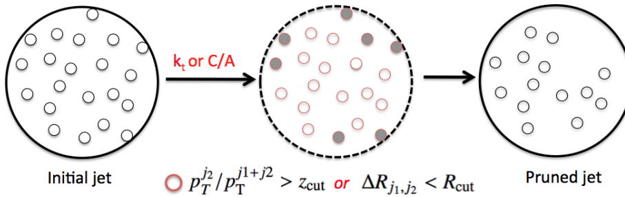
Figure 2.8: (taken from [95]) Jet pruning as grooming technique: as a first step, a jet is re-clustered with k_t (or CA) algorithm; as second step, for each pair of constituents two conditions are checked, for each pair not satisfying any of the conditions, the softer of them is removed from the set of constituents. Finally the remaining constituents define a pruned jet, where all the constituents are hard enough to be considered itself as subjects. R_{cut} in the figure has the same meaning that R_{prune} in the text.
