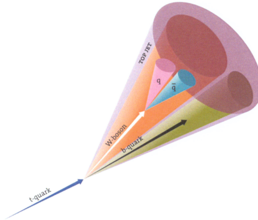
Figure 3.9: Schematic representation of the reconstruction of the t quark into the jet. The top jet candidate is represented, as well as the soft drop subjets (the inner cones). This case represents a fully merged scenario where all the decay products are inside the fat jet, and the hadronic products of the W -boson can be clustered in the first subjet, while the second subjet gathers all the remaining soft radiation and the decay products of the b -quark.
