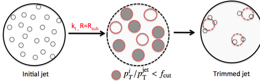
Figure 2.7: (taken from [95]) Jet trimming as grooming technique: as first step, a jet is clustered with k_t algorithm (taking as radius parameter R ); as a second step, a set of subjects are defined with radius parameter R_{sub} , and only those ones with p_{T,i} > f_{cut} p_T are kept to finally define the trimmed jet.
