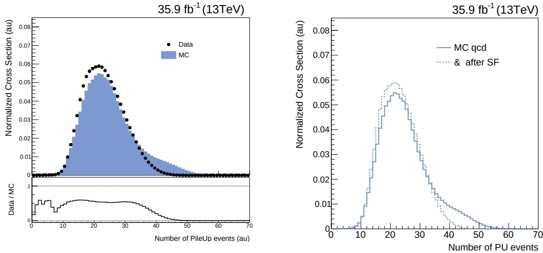
Figure 6.12: (left) Pileup distributions in a QCD Monte Carlo sample, compared to the pileup distribution in data collected during 2016. (right) Pileup distribution in Monte Carlo sample before and after applying the scale factors for re-weighting of the events.
