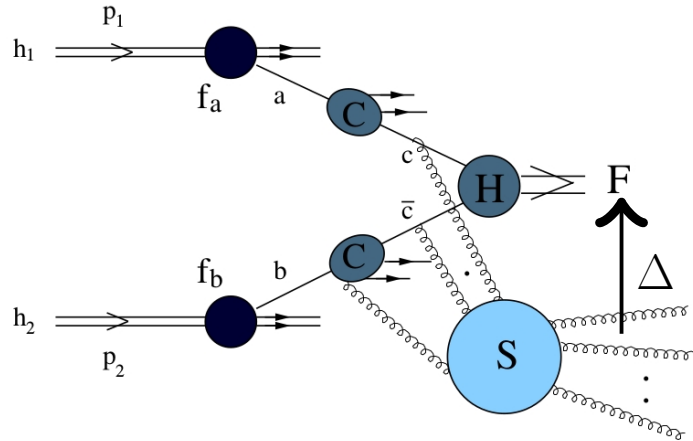
Figure 1.14: (modified from [70]) Factorization theorem of the hard process: the factors C represents the collinear radiations of a parton a or b at scale 1/b ; S is the Sudakov form factor representing the soft and flavour conserving collinear radiation in the scale 1/b \leq q_T \leq M , M is the top-quark mass, and H represents the hard process calculated at a fixed order. The factorization breaking introduces an additional term ( \Delta ) to account for the colour-connection between the initial state radiation (contained in the Sudakov factor) and the final state radiation.
