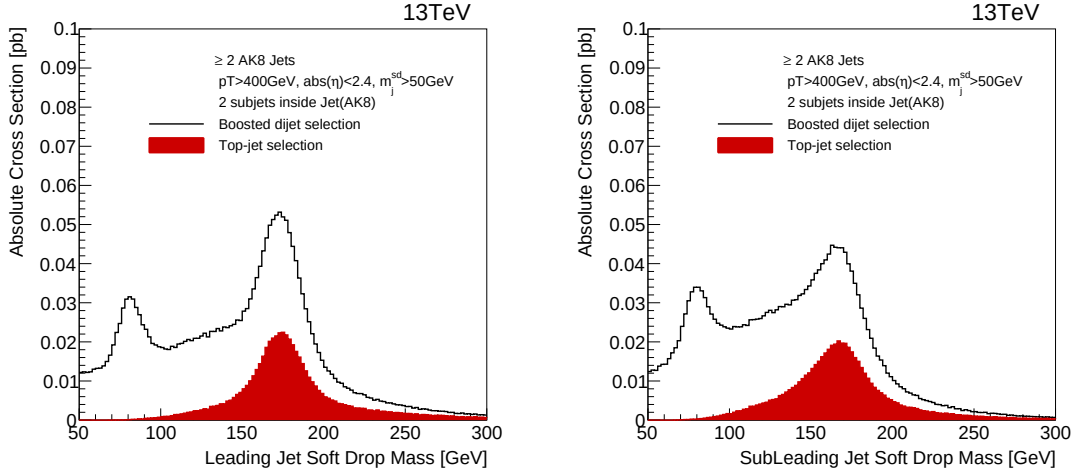
Figure 6.5: Soft Drop jet mass distributions in t\bar{t} simulated events, after applying the boosted-dijet selection criteria, and after applying in addition the top-jet selection for: (left) leading and (right) subleading jets.
