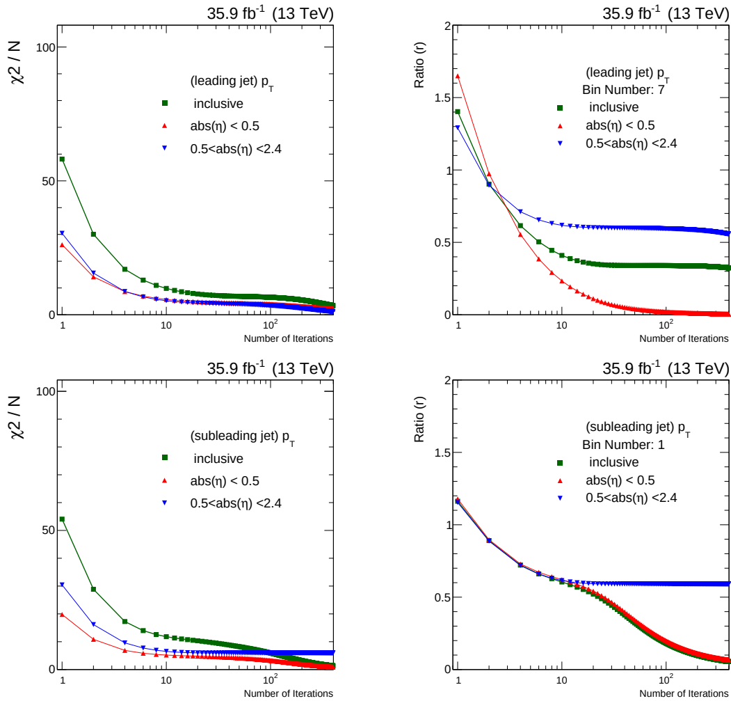
Figure 9.7: (left) \chi^2 (equation 9.23) distribution and (right) r (equation 9.24) distributions as function of the number of iterations of the unfolding procedure, performed for the p_T spectra of the leading jet (upper plots), subleading jet (lower plots). The inclusive fiducial phase space, and the exclusive regions defined with |\eta| observable are shown in each plot.
