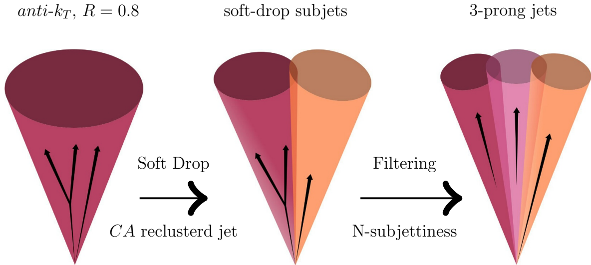
Figure 3.1: Schematic picture showing how the jet clustering and jet substructure techniques are used in this thesis (top jet tagging in the boosted regime).
