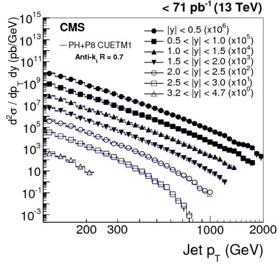
Figure 2.1: (taken from [79]) Double differential cross section as function of p_T of the jet. Jets are clustered with anti\text{-}k_t algorithm with radius parameter R = 0.7 . The solid lines represent predictions at NLO produced with POWHEG+PYTHIA8.
