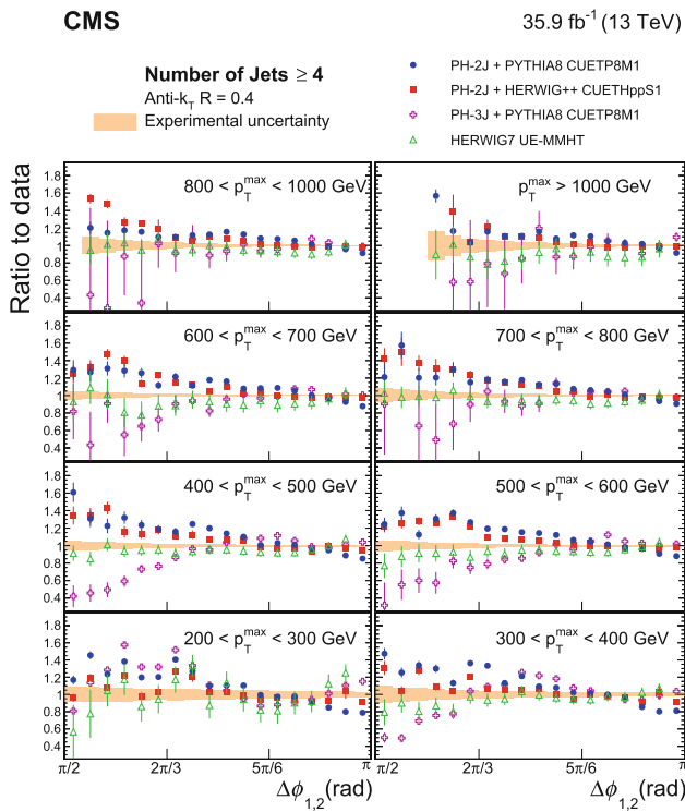
Fig. 9 Ratios of PH-2J + PYTHIA 8, PH-2J + HERWIG++, PH-3J + PYTHIA 8, and HERWIG 7 predictions to the normalized inclusive 4-jet cross section differential in \Delta\phi_{1,2} , for all p_T^{\max} regions. The solid band indicates the total experimental uncertainty and the vertical bars on the points represent the statistical uncertainties in the simulated data
