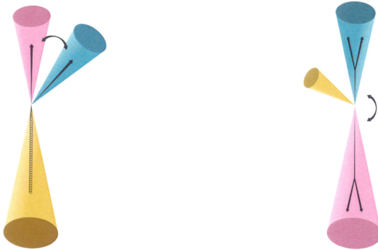
Figure 3.6: Sketch representing t\bar{t} events. The top-jets are shown with blue and pink cones, and the additional jet with a yellow cone. Two scenarios are represented. (Left picture) the t\bar{t} system is boosted itself, and the two top-jets are the leading and third jets, while the leading jet (yellow colour) contains the recoiling QCD radiation of the t\bar{t} system. (Right picture) the two leading jets are the two top jets, while the third jet (yellow colour) contains additional radiation, having low p_T value. The decay products of the t -quarks (right picture) are contained within the top jets.
