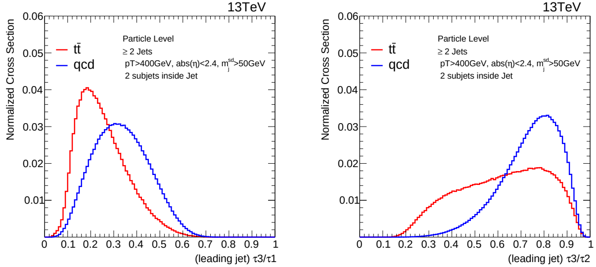
Figure 3.4: N -subjettiness observables in QCD and t\bar{t} simulated events (left) \tau_3/\tau_1 (right) \tau_3/\tau_2 . Distributions correspond to the particle level after applying the boosted selection.
