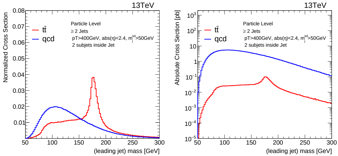
Figure 2.6: Jet mass distribution for the leading jet in QCD and t\bar{t} simulated events: (left) normalized distributions (right) absolute cross section. Jets are reconstructed using anti- k_t with R = 0.8 .
