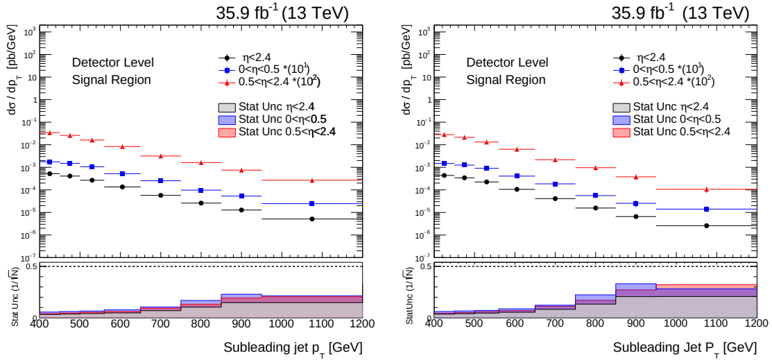
Figure 8.2: Cross section in the fiducial phase space (detector level) differential in the transverse momentum p_T of the subleading jet: (left) inclusive top jet measurements (right) t\bar{t} measurements.
