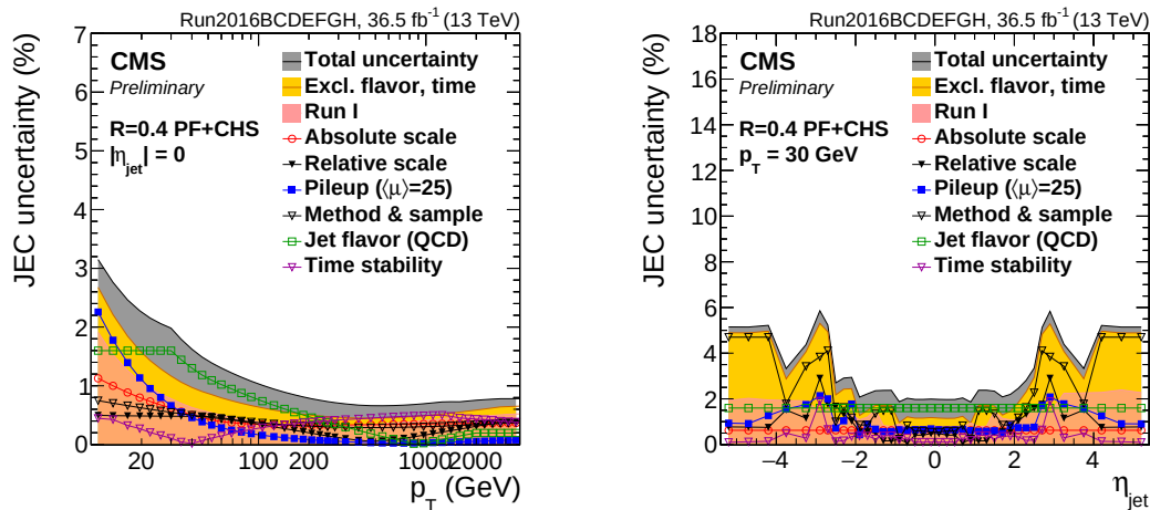
Figure 5.7: (from[140])Uncertainty of Jet Energy Scale with sum of all uncertainties in quadrature and the sources (left) as a function of p_t , (right) as a function of \eta .
