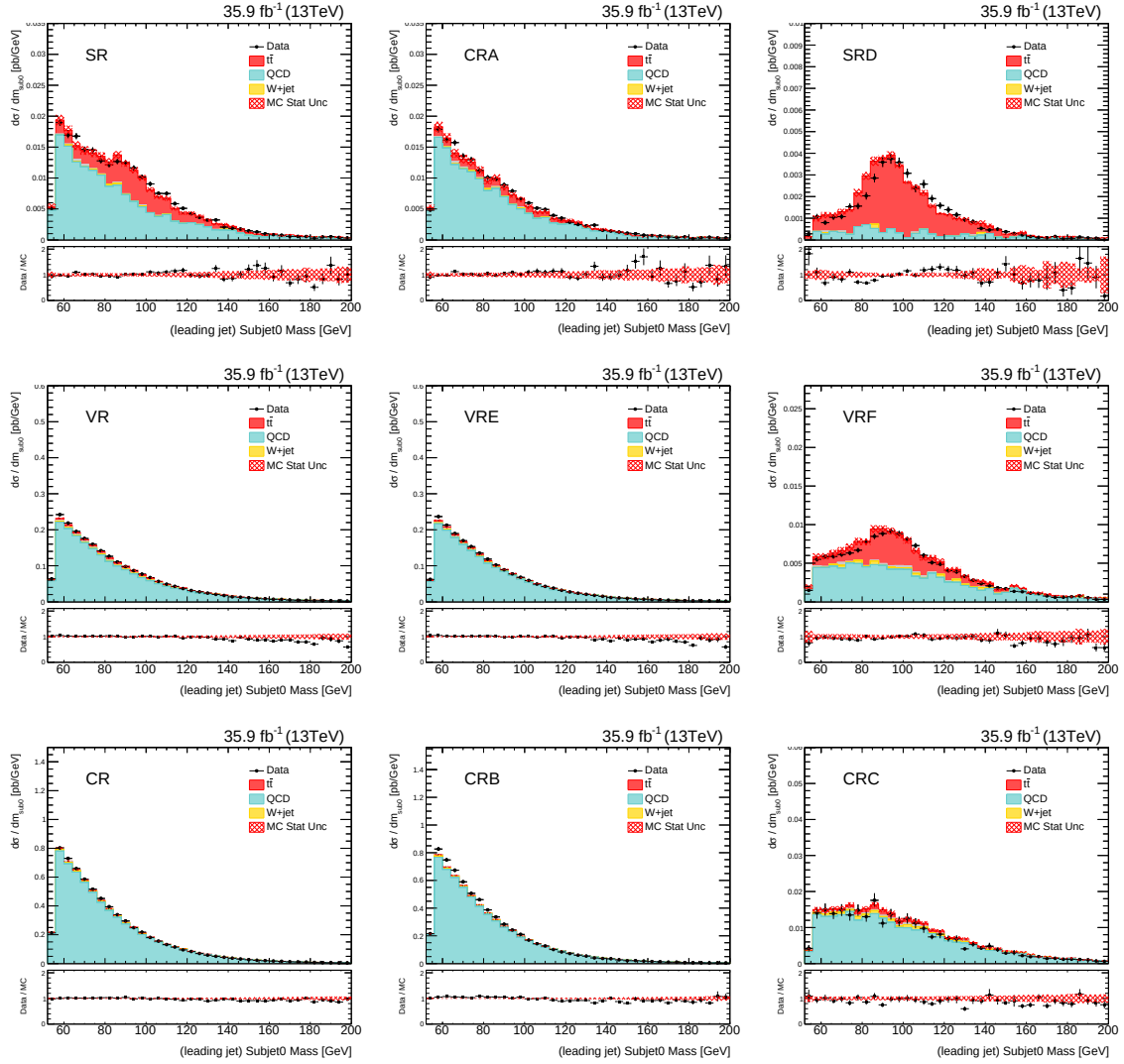
Figure F.2: First subjet soft drop mass distributions for the leading jet in different regions defined in Figure 8.5. The normalization factor for the t\bar{t} contribution has been taken as N_{t\bar{t}} = 0.654 , while for the QCD multijet contribution: N_{QCD} = 0.74 in the first row (2-btagged jets), N_{QCD} = 0.67 in the second row (exclusively 1-btagged jet), N_{QCD} = 0.6 in the third row (zero btagged jet).
