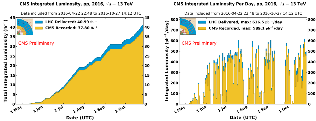
Figure 4.2: (taken from [111]) (left) integrated luminosity over the whole 2016 taking data period, (right) integrated luminosity on a day-per-day basis during the 2016 taking data period. Both, LHC delivery luminosity and CMS recorded luminosity are shown.
