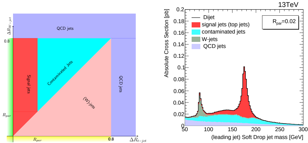
Figure C.1: (left) Sketch picture representing the phase space region defined by \Delta R_{W-jet} and \Delta R_{t-jet} observables. Different jet categories defined in this section are illustrated. (right) Soft Drop jet mass distribution for the leading jet in t\bar{t} events. Jets are classified following the jet categories in the sketch.
