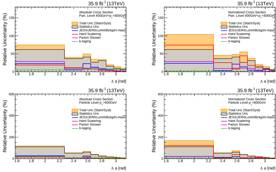
Figure H.1: Systematic and statistical uncertainty corresponding to the distributions differential in \Delta\phi in two p_T^{lead} regions: (upper plots) 400\text{GeV} < p_T < 600\text{GeV} , (down plots) p_T > 600\text{GeV} . The systematic uncertainty corresponding to the absolute and normalized distributions are illustrated.
