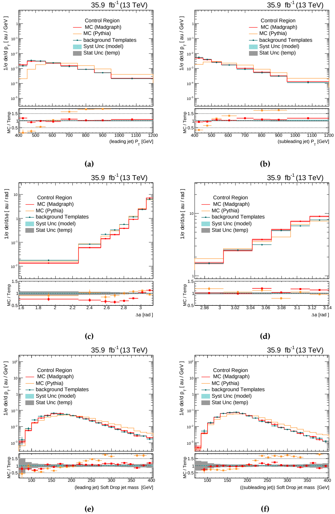
Figure 8.10: Comparison of background templates obtained with a data-driven method with respect to the Monte Carlo prediction in the Control Region. The plots corresponds to the following observables: (upper left) leading jet p_T (upper right) subleading jet p_T , (middle left) \Delta\phi between the two leading jets (middle right) \Delta\phi in the back to back region (lower left) soft drop jet mass of the leading jet (lower right) soft drop jet mass of the subleading jet.
