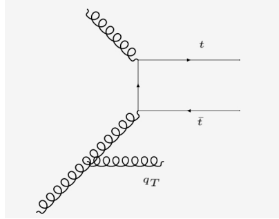
Figure 1.12: Feynman diagram representing a t\bar{t} pair production process, in which, additionally, a gluon with transverse momentum q_T is emitted.
