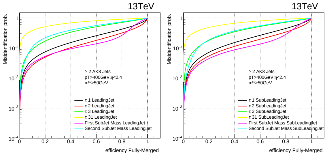
Figure D.3: Efficiency of correctly identifying fully merged top jets with respect to the misidentification probability of classifying non-merged jets as fully merged: (left) leading jet, (right) subleading jet.
