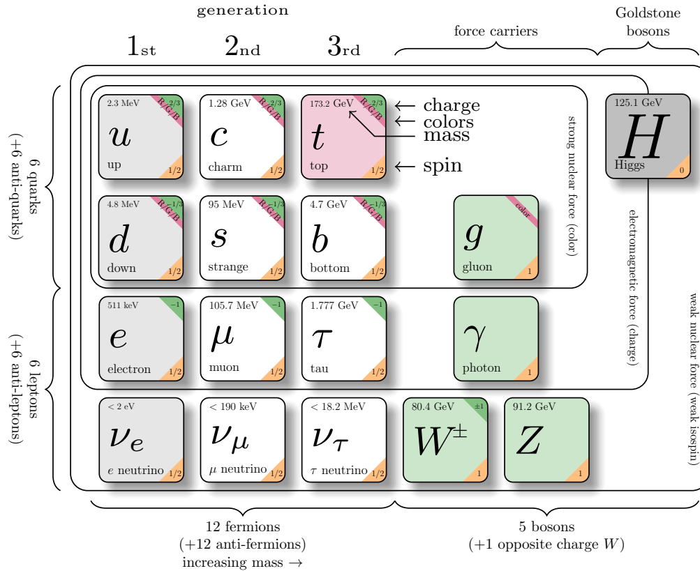
Figure 1.1: (figure modified using a template from [12]) Summary of particles building the Standard Model of fundamental particles in the nature. In the model, two main groups can be distinguished, the fermions (left) and bosons (right). The former ones are the particles building up matter while the latter ones are responsible for their interactions and masses. The fermions can be divided into two main groups: quarks and leptons, and in three generations, depending on their mass. The bosons are represented in the picture according to the interactions that they are responsible for. The gluons are responsible for the strong interaction, the photons for the electromagnetic interaction, and the bosons W^\pm and Z for the weak interaction. The Higgs boson appears as a result of the spontaneous symmetry breaking and its field is responsible for giving mass to all the particles in the SM. The information like the electric charge, the colour charge, the mass and the spin of each particle is provided.
