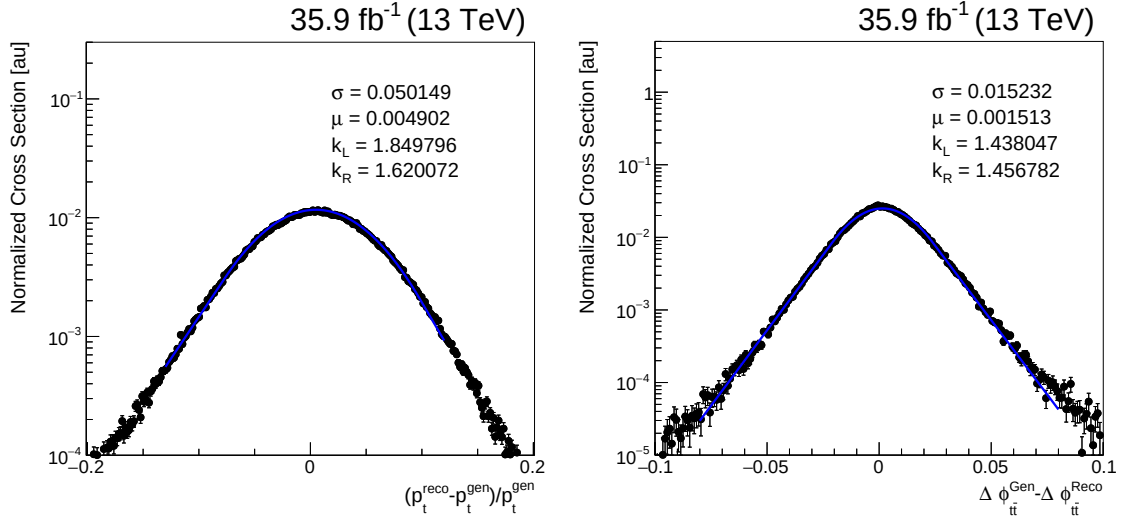
Figure 9.2: Resolution response with respect to: (left) p_T observable (given by equation 9.3), (right) \Delta\phi observable (given by equation 9.2). The resolution response are fitted to a ExpGaussianExp (9.6) distribution with four free parameters, whose values after the fits are illustrated in each plot.
