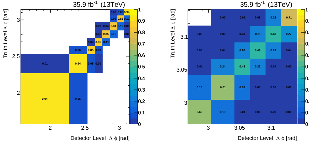
Figure 9.4: Response matrices for the \Delta\phi observable in the inclusive fiducial phase space ( p_T > 400 GeV, |\eta| < 2.4 ) taking into account different regions in \Delta\phi : (left) \pi/2 < \Delta\phi < \pi (right) 2.96 < \Delta\phi < \pi (back to back region). The two last bins in the left plot correspond to the bins shown in the right plot. Each row has been normalized to the number of events in each corresponding stable particle bin.
