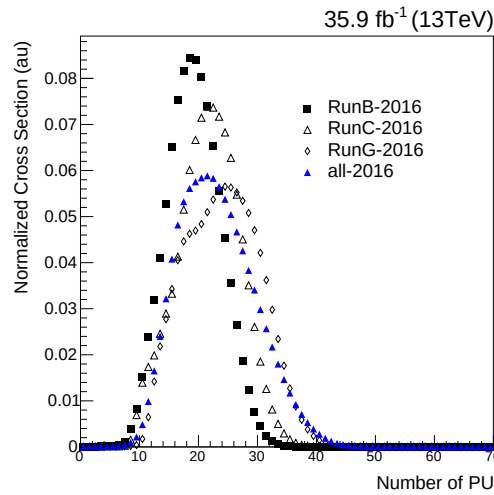
Figure 6.1: Pileup distributions measured in data during different runs periods. The blue points represent the whole data recorded during the year 2016.
