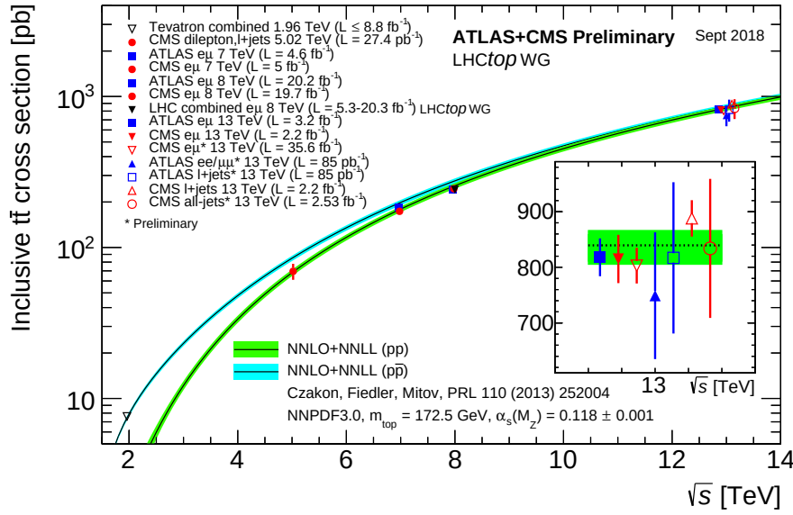
Figure 1.6: (taken from [64]) Summary Measurements of the inclusive t\bar{t} cross section in pp and p\bar{p} collisions compare to SM theory predictions. The SM predictions correspond to NNLO-NNLL accuracy of the QCD processes [53], while the coloured bands represent the theory uncertainties.
