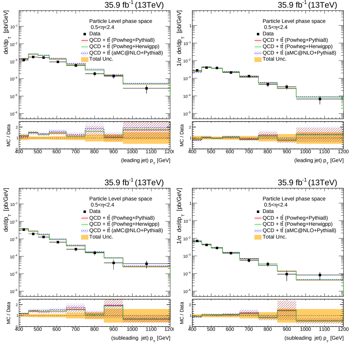
Figure I.3: Cross section (left plots) and normalized distributions (right plots) differentially in (upper plots) the p_T of the leading jet, (lower plots) the p_T of the subleading jet, compared to theory predictions. The total uncertainty are shown for each measurements in the lower panels, while in the upper panels only the statistical uncertainties are shown. The shown uncertainty in the theory predictions are the statistical uncertainties. The distributions correspond to the inclusive top-jet cross section, when the exclusive region of the phase space: 0.5 < |\eta| < 2.4 is considered.
