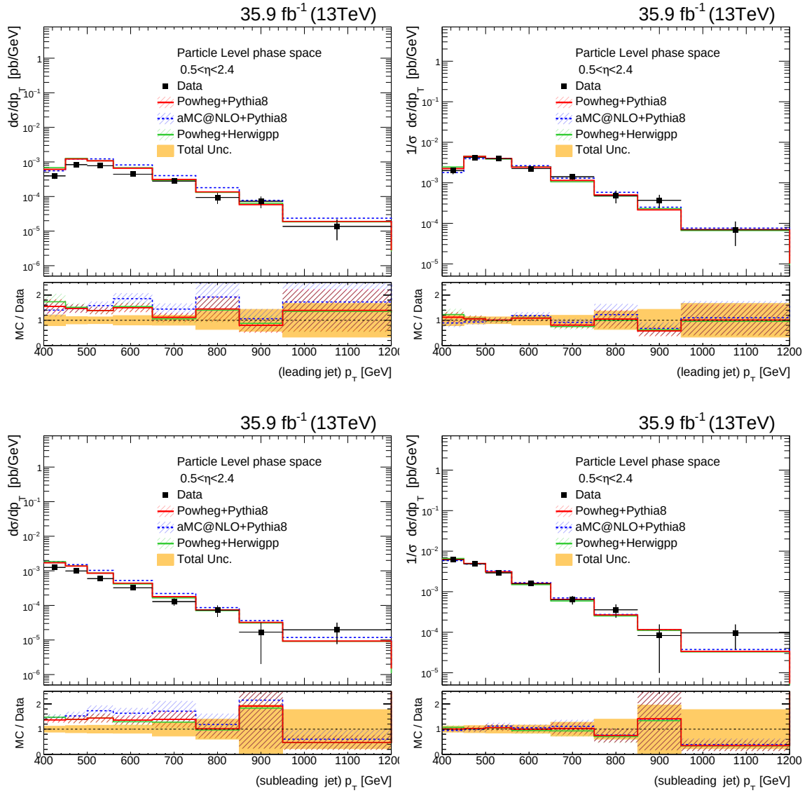
Figure 11.4: Cross section (left plots) and normalized distributions (right plots) differential as function of the p_T of the leading jet (upper plots), subleading jet (lower plots) compared to theory predictions. The total uncertainty are shown for each measurements in the lower panels, while in the upper panels only the statistical uncertainties are shown. The shown uncertainty in the theory predictions are the statistical uncertainties. The t\bar{t} measurements are performed in 0.5 < |\eta| < 2.4 .
