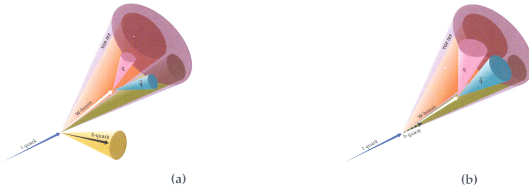
Figure 3.7: Schematic representation of the jets not properly reconstructing the t -quarks. The top jet candidate is represented, as well as subjets (the inner cones). Two cases are shown (a) non boosted topologies, the b -quark is outside the jet (b) the p_T of the b -quark has small p_T and is removed by the soft Drop Mass.
