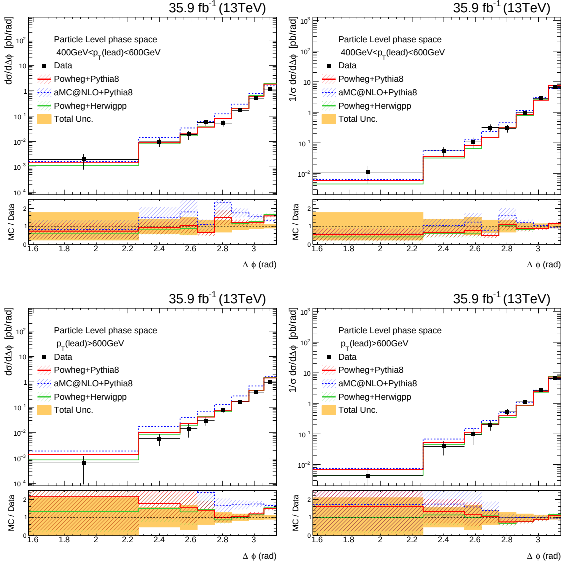
Figure 11.7: Cross section (left plots) and normalized distributions (right plots) differential as function of the \Delta\phi between the two top-jets, compared to theory predictions. The total uncertainty are shown for each measurements in the lower panels, while in the upper panels only the statistical uncertainties are shown. The shown uncertainty in the theory predictions are the statistical uncertainties. The t\bar{t} measurements are performed in: (upper plots 400 \text{ GeV} < p_T^{\text{lead}} < 600 \text{ GeV} ), (lower plots) p_T^{\text{lead}} > 600 \text{ GeV} .
