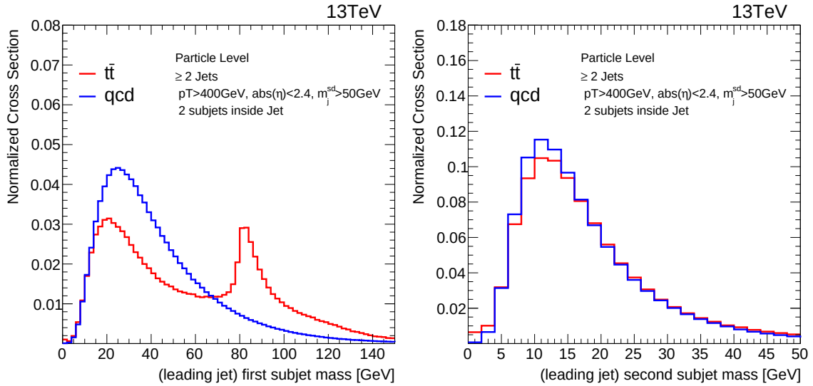
Figure 3.3: Jet mass distribution for the subjets in QCD and t\bar{t} simulated events (left) first subjet (right) second subjet. Distributions correspond to the particle level after applying the boosted selection.
