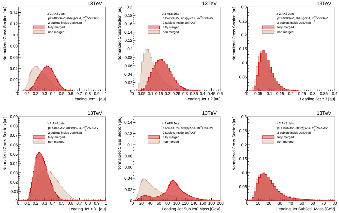
Figure D.2: Discriminating variables considering the leading jet in order to select fully and non merged jets: (upper, left) \tau_1 , (upper, middle) \tau_2 , (upper, right) \tau_3 , (down, left) \tau_{31} , (down middle) first subjet soft drop mass, (down right) second subjet soft drop mass.
