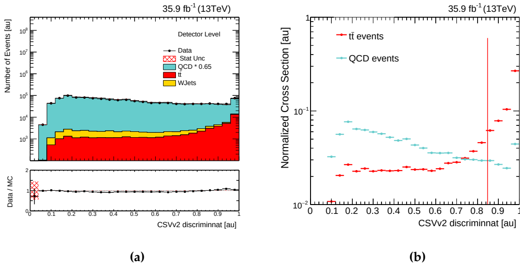
Figure 6.8: (left) Output discriminant of the CSVv2 in data, before the b-tagging selection criteria is applied, with the respective contributions of different sources of events, estimated by Monte Carlo simulations. (right) Normalized distribution as function of the CSVv2 tagger, in t\bar{t} and QCD multijet events.
