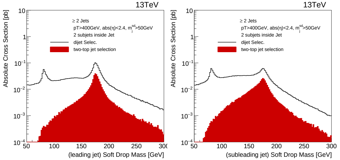
Figure 3.10: Soft drop jet mass distributions in t\bar{t} simulated events for: (left) leading jet (right) subleading jet. Two selections are shown, the dijet boosted selection (black line curve) and when two top-jets are required (red shaded curve).
