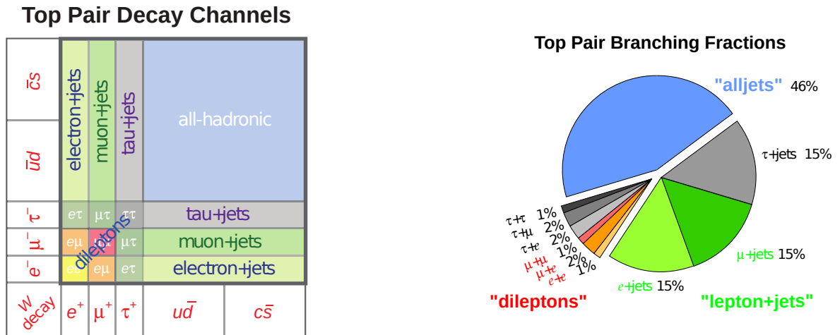
Figure 1.9: (taken from [66]) (Left picture) Possible decay channels for the t\bar{t} pair given by the decays of the W -bosons. (Right picture) relative probabilities for each of the decay channels. In the case of the leptonic decays, the corresponding neutrino accompanying the leptons is not mentioned (i.e W^+ \rightarrow e^+\nu_e is recognized as e^+ channel).
