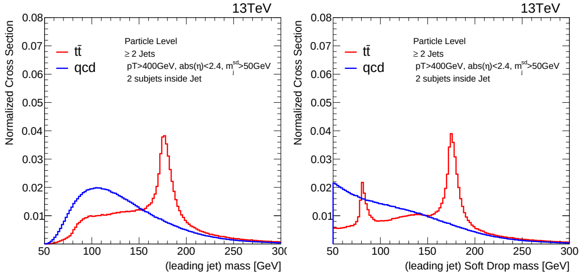
Figure 3.2: Jet mass distribution for the leading jet in QCD and t\bar{t} simulated events (left) the pure jet mass (right) the soft drop jet mass. Distributions correspond to the particle level after applying the boosted selection.
