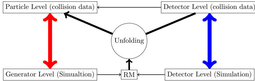
Figure 9.6: Sketch showing the unfolding procedure: the response matrix (RM) is obtained from the simulation of both levels (particle level and detector level distributions). Based on this input information, the unfolding method corrects the collision data at detector level to the data distribution at the corresponding stable particle level.
