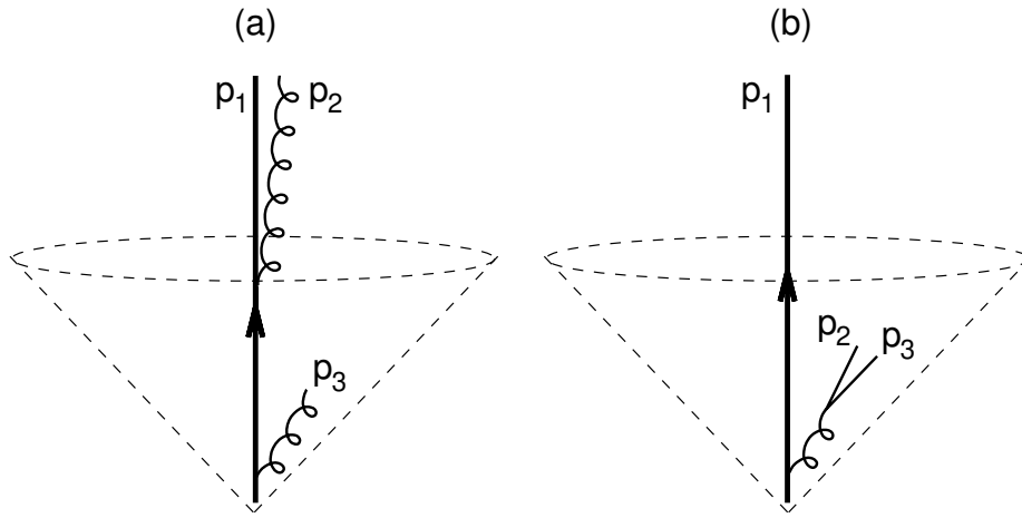
Figure 2.9: (taken from [97]) (a) a jet defined by a hard parton p_1 emitting two gluons p_2 and p_3 (b) a jet defined as a hard parton p_1 emitting a gluon, the gluon emits later two partons p_2, p_3 .
