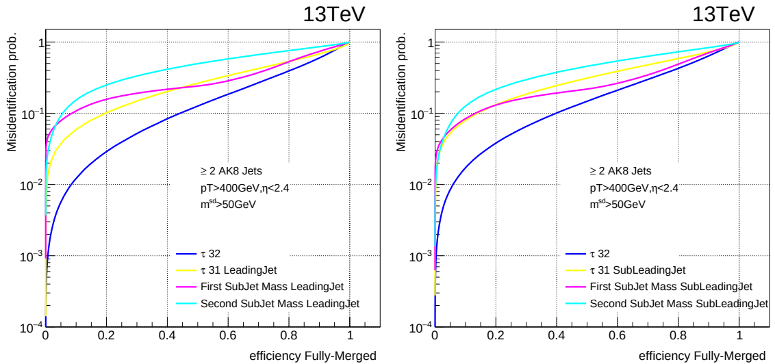
Figure C.4: Signal efficiency for top-jet selection as function of the misidentification probability of classifying as signal jet a non-top jet. Different observables are considered as discriminating variables. The leading jet (left plot) and the subleading jet (right plot) are considered independently.
