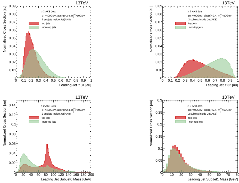
Figure C.3: Normalized distributions considering top jets and non-top jets for the leading jet in simulated t\bar{t} events. The classification for top-jets and non-top jets corresponds to the parton level definition presented in section C.1. The following observables are considered: (upper, left) \tau_3/\tau_1 ; (upper, right) \tau_3/\tau_2 ; (down, left) m_j^{sub0} ; (down, right) m_j^{sub1} .
