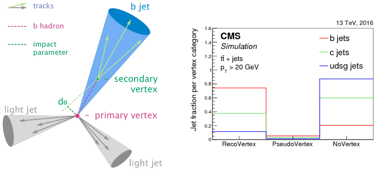
Figure 5.8: Secondary Vertex Reconstruction: (left) schematic picture of the second vertex reconstruction in a jet containing a B-Hadron (b-jet), Two light jets are also represented, which are originated directly from the primary vertex, and been distinguished from the one containing a secondary vertex ( taken from[146]) , (right) probability of each vertex category for secondary vertices reconstructed with the Inclusive Vertex Finder [145] algorithm for light, c, and b-jets (take from [143] )
