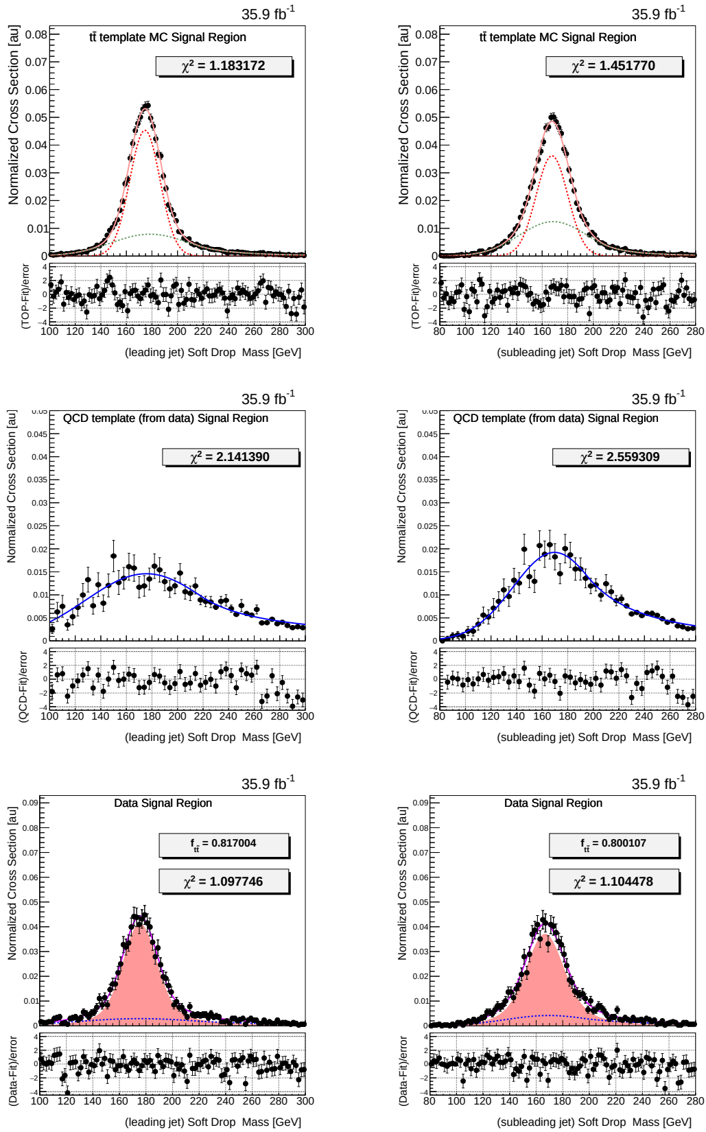
Figure 8.15: Different steps in the fit procedure in the signal region considering the Soft Drop Mass distribution of: (left) the leading jet, (right) the subleading jet. The upper plots show the fit of the signal template, S(m) , the middle plots show the fit of the background templates ( B(m) ) and the lower plots show the fit of the data distributions ( D(x) )
