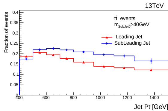
Figure 3.11: Event selection efficiency as function of the transverse momentum of the leading and sub-leading jets. As selection criteria two signal top jets are required, and as baseline selection, the boosted dijet selection is considered.
