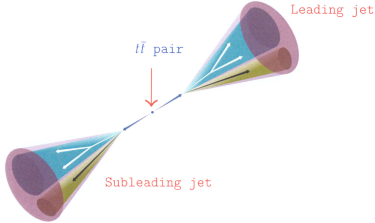
Figure 6.4: Schematic picture of an event where both leading jets are defined as signal top jets.
