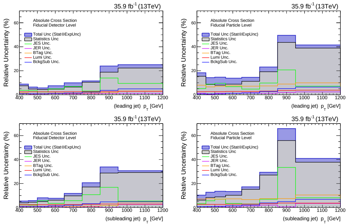
Figure 10.3: Breakdown of the experimental systematic uncertainties of the cross section measurements differential in p_T of the leading jet (upper plots) and subleading jet (lower plots) at: detector level (left plots) and particle level (right plots). The plots correspond to the measurements of the t\bar{t} cross section.
