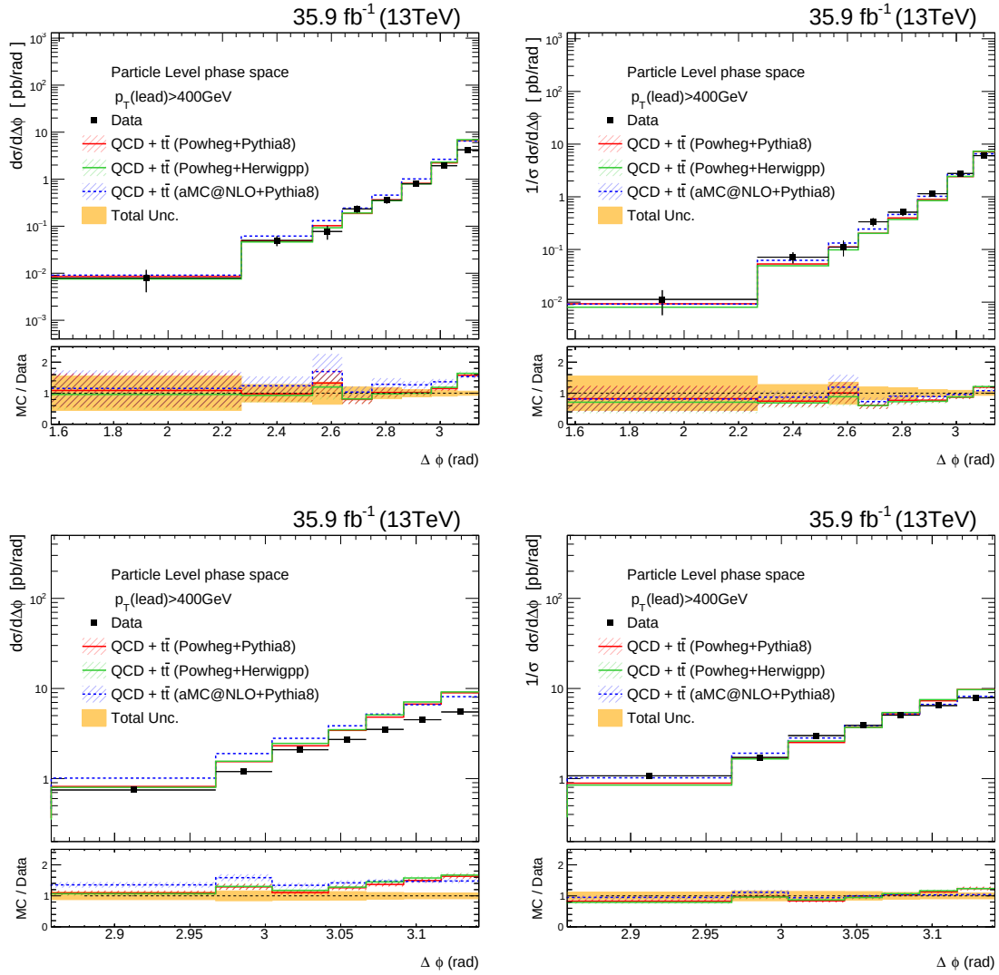
Figure 11.10: Cross section (left plots) and normalized distributions (right plots) differential in \Delta\phi between the two leading jets, compared to theory predictions. The total uncertainty are shown for each measurements in the lower panels, while in the upper panels only the statistical uncertainties are shown. The shown uncertainty in the theory predictions are the statistical uncertainties. The distributions correspond to the inclusive top-jet cross section.
