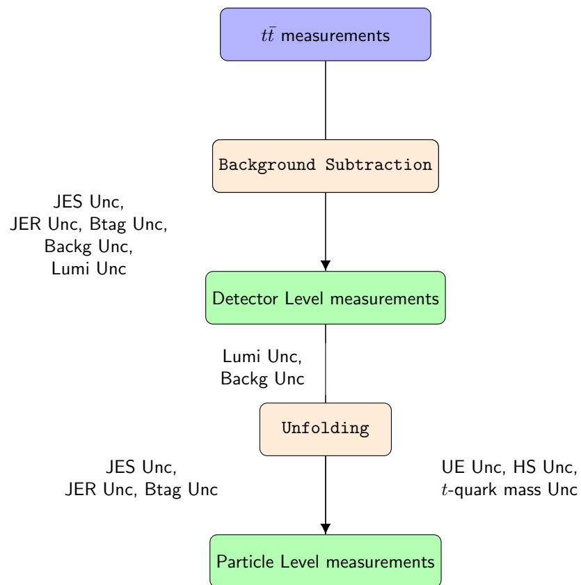
Figure 10.1: Sketch representing the systematic uncertainties in the measurement when the QCD background contribution has been subtracted.
