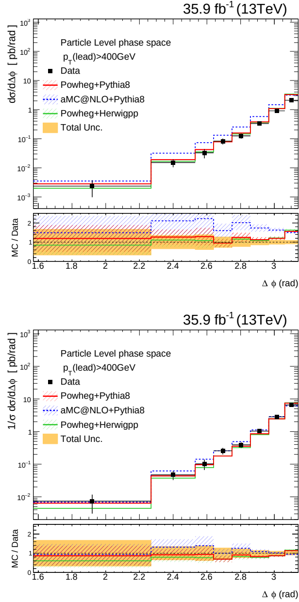
Figure 11.5: Cross section (upper plot) and normalized distributions (lower plot) differential as function of the \Delta\phi between the two top-jets, compared to theory predictions. The total uncertainty are shown for each measurements in the lower panels, while in the upper panels only the statistical uncertainties are shown. The shown uncertainty in the theory predictions are the statistical uncertainties. The t\bar{t} measurements are performed in the inclusive fiducial phase space region ( |\eta| < 2.4 , p_T > 400 GeV).
