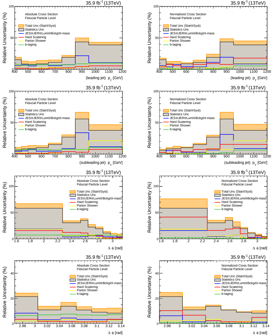
Figure 10.8: Systematic and statistical uncertainties corresponding to the distributions differential in p_T of the leading jet (two first plots), p_T of the subleading jets (second row), \Delta\phi (third row), and \Delta\phi in the back to back region (lower plots), in the fiducial particle level. The systematic uncertainties corresponding to the absolute and normalized distributions are illustrated.
