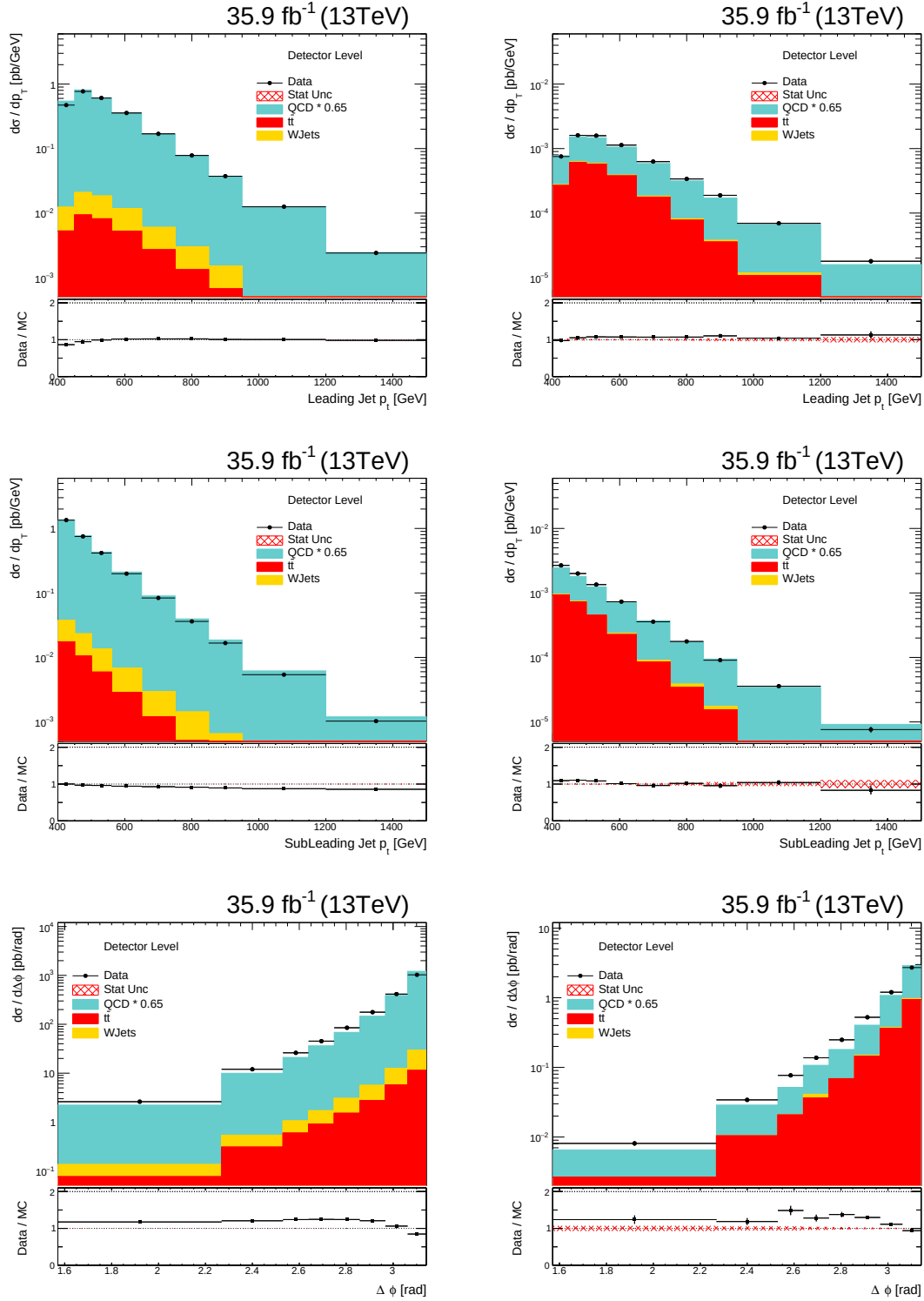
Figure 6.11: Cross section distributions differentially as function of: (upper plots) p_T of the leading jet (middle plots) p_T of the subleading jet, (lower plots) \Delta\phi between the two leading jets. Two phase regions are illustrated: (left) after boosted dijet selection, (right) signal region
