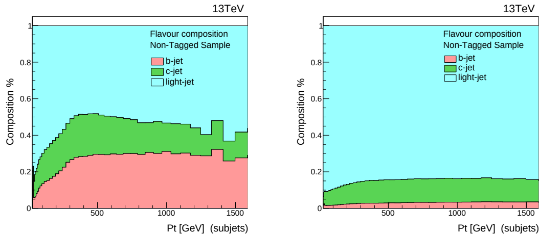
Figure E.4: Flavour composition for the non- b tagged sample: (left) t\bar{t} events, (right) QCD events.
