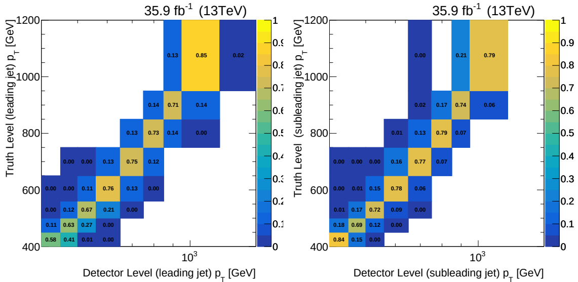
Figure 9.5: Response matrices for (left) p_T of the leading jet (right) p_T of the subleading jet. Each row has been normalized to the number of events in each corresponding stable particle bin.
