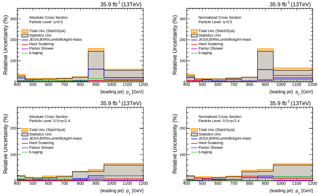
Figure H.2: Systematic and statistical uncertainty corresponding to the distributions differential in p_T of the leading jet in two different \eta regions: |\eta| < 0.5 (upper plots) and 0.5 < |\eta| < 2.4 (lower plots). The systematic uncertainty corresponding to the absolute (left) and normalized (right) distributions are illustrated.
