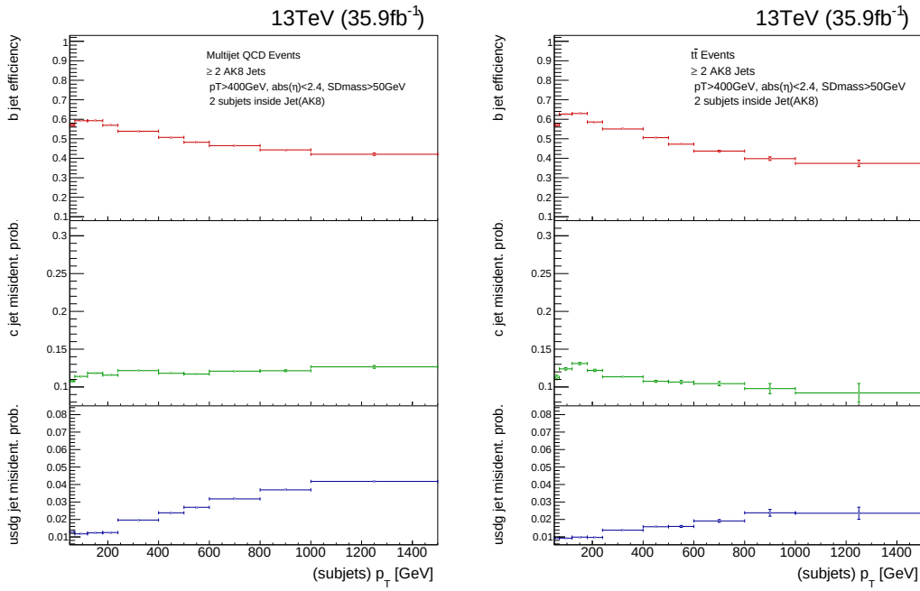
Figure 6.13: Monte Carlo b-tagging efficiencies as a function of p_T of the subjects, for each jet flavour: b-jets , c-jets , light-jets : for QCD events (left) and t\bar{t} events (right). The events are selected by applying the dijet boosted selection criteria.
