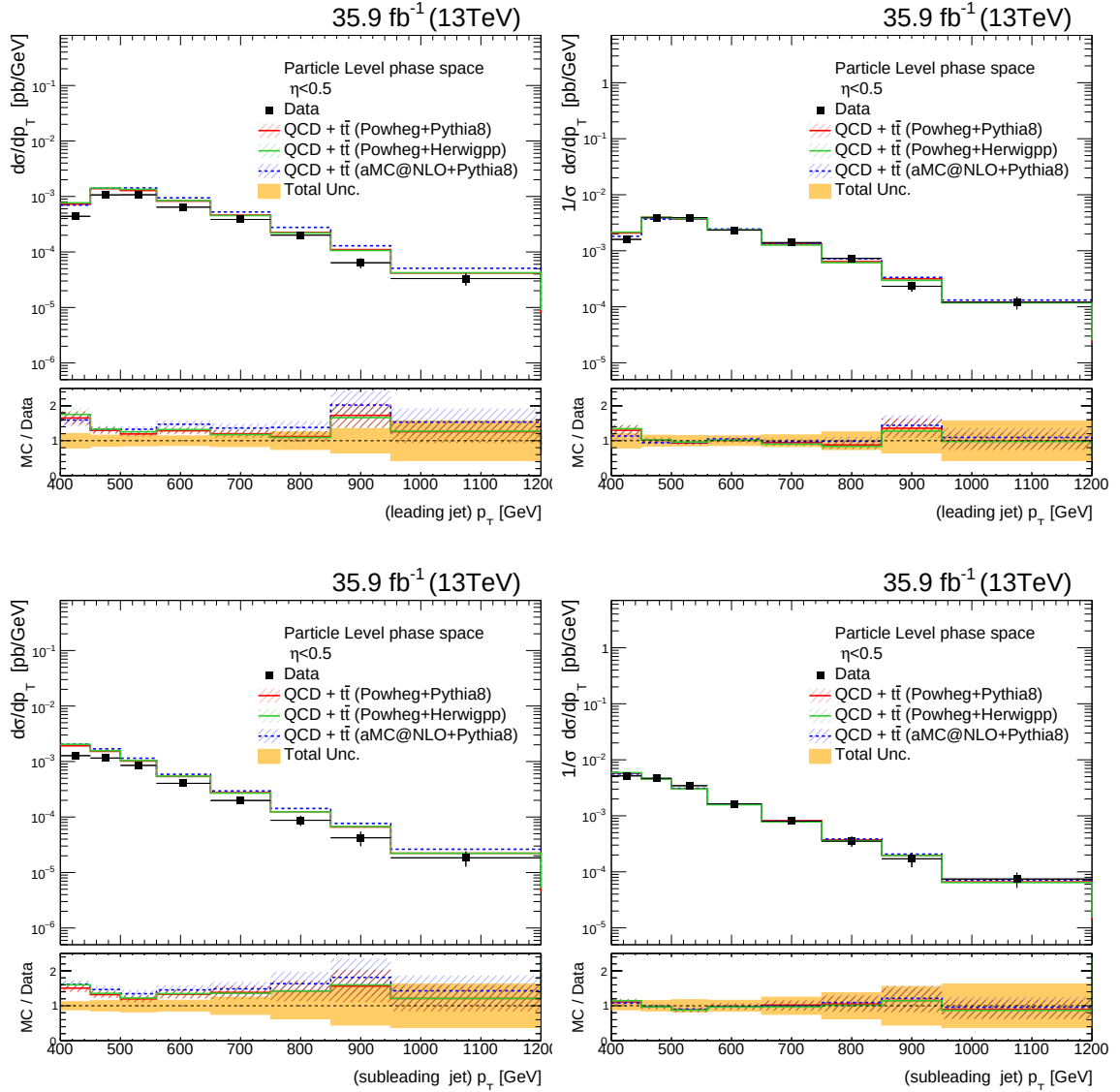
Figure I.2: Cross section (left plots) and normalized distributions (right plots) differentially in (upper plots) the p_T of the leading jet, (lower plots) the p_T of the subleading jet, compared to theory predictions. The total uncertainty are shown for each measurements in the lower panels, while in the upper panels only the statistical uncertainties are shown. The shown uncertainty in the theory predictions are the statistical uncertainties. The distributions correspond to the inclusive top-jet cross section, when the exclusive region of the phase space: |\eta| < 0.5 is considered.
