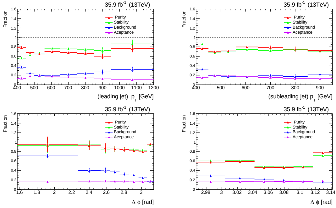
Figure 9.3: Purity, stability, background and acceptance in the fiducial - particle phase space, for the following observables: (upper left) p_T leading, (upper right) p_T subleading, (lower) \Delta\phi .
