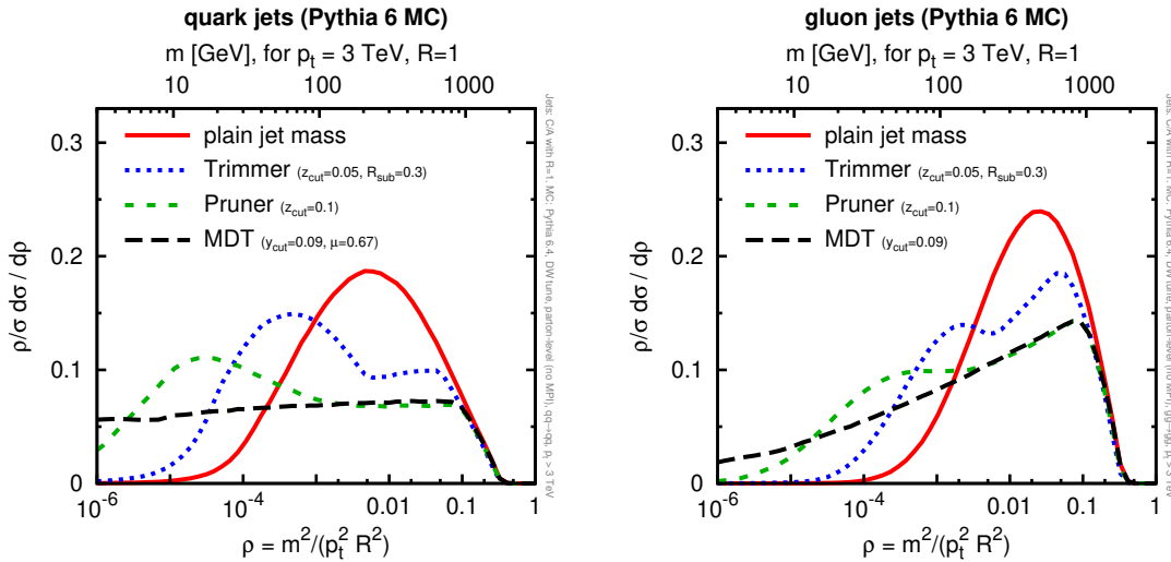
Figure 2.3: (taken from [83]) \rho distribution considering different groomer taggers (trimming, pruning, mass drop), and the plain jet mass estimated with MC for: (left) quark jets (right) gluon jets. The upper x -axis shows the values of the jet mass, specifically considering jets of radius R = 1 , and p_T = 3 TeV.
