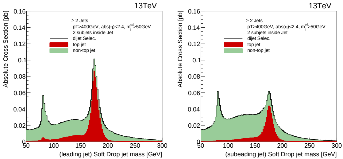
Figure C.2: Soft Drop jet mass distribution for (left) leading jet, (right) subleading jet, in t\bar{t} simulated events. Events were selected with the boosted dijet criteria. Two jet categories are shown: top jets, and non-top jets, using the parton level information.
