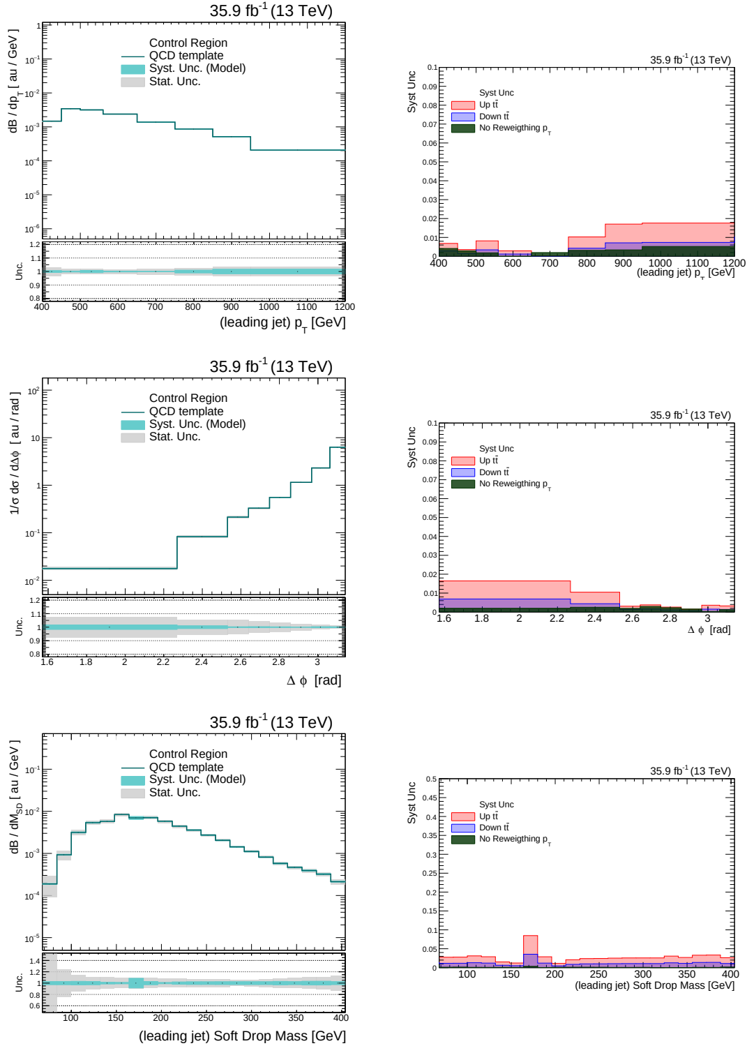
Figure 8.9: (left) Background template distributions in the control region and (right) systematic model-dependence uncertainties, for three observables: (upper) p_T of the leading jet, (middle) \Delta\phi , (lower) the Soft Drop mass of the leading jet.
