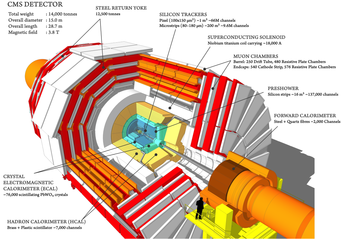
Figure 4.3: (taken from [113]) Sketch representing the CMS detector with the corresponding subdetector. Some features of the detector are additional provided.
