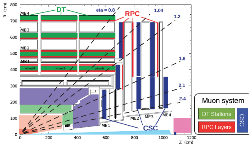
Figure 4.8: (taken from [119]) Sketch showing the Muon system of the CMS detector located in the outer part of the CMS machinery.
