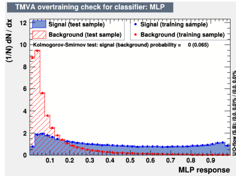
Figure 7.6: Test and training samples for background and signal events of the output of the MLP algorithm. The output discriminant for signal events is represented in blue while for background events in red.
