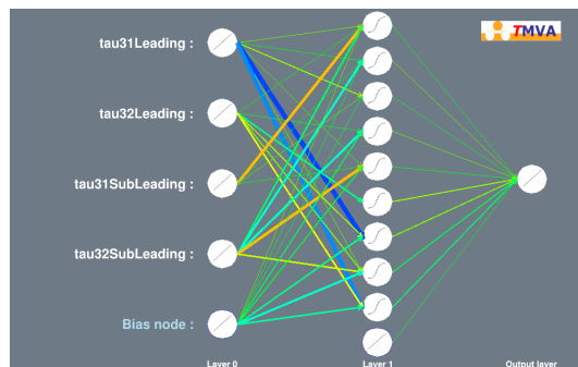
Figure 7.2: Neural network architecture for the Multilayer perceptron (MLP) algorithm. This Neural network is the one used to perform the training and testing procedure and provide the output discriminant for the event selection. \tau_3/\tau_2 , \tau_3/\tau_1 for the leading and subleading jets are the input variables considered for the MLP architecture.
