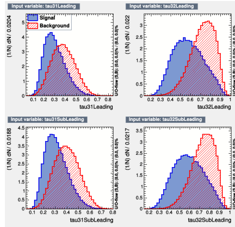
Figure 7.4: Input variables to the MLP algorithm, comparison between the shapes of the observables. The symbols \tau_{31} and \tau_{32} mean the ratio \tau_3/\tau_1 and \tau_3/\tau_2 respectively.
