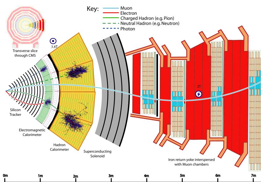
Figure 5.2: (taken from [123]) Schematic picture representing the interaction of particles with different parts of the CMS detector: five types of stable particles are illustrated: muons, electrons, charged hadrons, neutral hadrons, and photons. The Tracker System, Electromagnetic Calorimeter, Hadron Calorimeter, and Muon System are represented.
