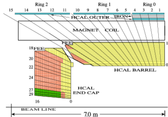
Figure 4.7: (taken from [118]) Schematic view of part of the HCAL in the CMS detector. The Forward HCAL is not shown which is located in the most forward region.
