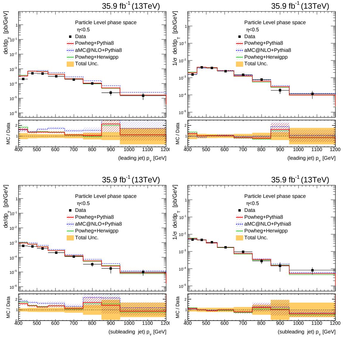
Figure 11.3: Cross section (left plots) and normalized distributions (right plots) differential as function of the p_T of the leading jet (upper plots), subleading jet (lower plots), compared to theory predictions. The total uncertainty are shown for each measurements in the lower panels, while in the upper panels only the statistical uncertainties are shown. The shown uncertainty in the theory predictions are the statistical uncertainties. The t\bar{t} measurements are performed in |\eta| < 0.5 .
