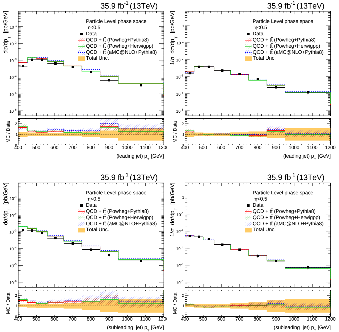
Figure I.2: Cross section (left plots) and normalized distributions (right plots) differentially in (upper plots) the p_T of the leading jet, (lower plots) the p_T of the subleading jet, compared to theory predictions. The total uncertainty are shown for each measurements in the lower panels, while in the upper panels only the statistical uncertainties are shown. The shown uncertainty in the theory predictions are the statistical uncertainties. The distributions correspond to the inclusive top-jet cross section, when the exclusive region of the phase space: |\eta| < 0.5 is considered.
