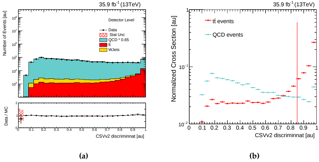
Figure 6.8: (left) Output discriminant of the CSVv2 in data, before the b-tagging selection criteria is applied, with the respective contributions of different sources of events, estimated by Monte Carlo simulations. (right) Normalized distribution as function of the CSVv2 tagger, in t\bar{t} and QCD multijet events.
