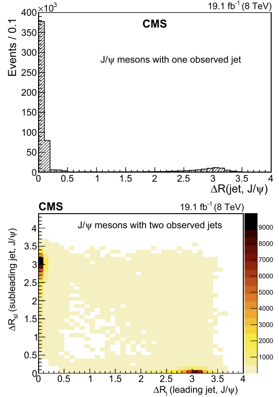
Fig. 1. The distributions of (upper) \Delta R (jet, J/\psi ) for one-jet events and (lower) \Delta R_l (leading jet, J/\psi ) vs. \Delta R_{sl} (subleading jet, J/\psi ) for two-jet events.
