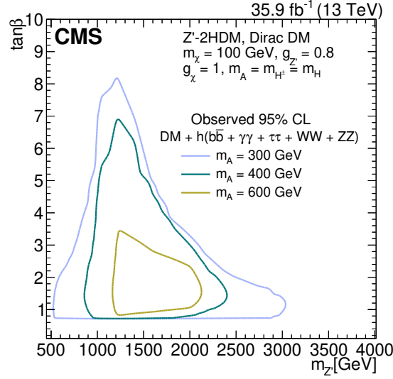
Figure 10. The upper limits at 95% CL on the observed \sigma/\sigma_{\text{th}} for the Z' -2HDM in the m_{Z'}\text{--}\tan\beta plane from the combination of the five Higgs boson decay channels. Each contour represents the excluded region for a given value of m_A = 300, 400, \text{ and } 600 GeV.
