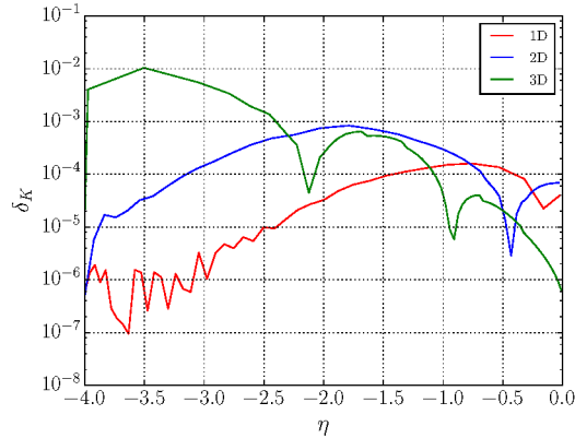
Figure 15. The plot shows \delta_K as a function of time for simulations in 1D, 2D and 3D. The Lyapunov-Irvine test is passed ( \delta_K \ll 1 ) in all cases. See text for the parameters of the simulations.
