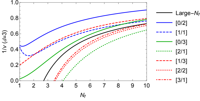
FIG. 3. Padé approximants for 1/\nu as a function of N_f at two (blue), three (green), and four-loop (red) orders. The large- N_f result (94) is shown in black.
