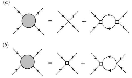
FIG. 1. One-loop renormalization of four-point vertices due to \mathbb{Z}_4 anisotropy (dashed lines: scalar field propagator, ordinary crossing: |\phi|^4 vertex, box: \phi^4 or \phi^{*4} vertex). Renormalization of (a) the four-scalar coupling \lambda^2 , (b) the anisotropy b .
