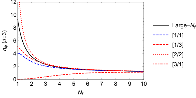
FIG. 2. Padé approximants for \eta_\phi as a function of N_f at two (blue) and four-loop (red) orders. The large- N_f result (93) is shown in black.
