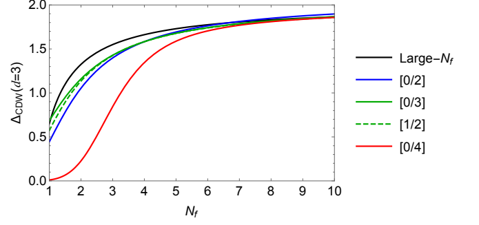
FIG. 4. Padé approximants for \Delta_{\text{CDW}} as a function of N_f for d = 3 at two (blue), three (green), and four-loop (red) orders. The large- N_f result (97) is shown in black.
