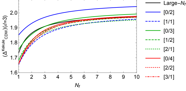
FIG. 5. Padé approximants for \Delta_{\text{CDW}} in the chiral O(2) GNY model as a function of N_f for d = 3 at two (blue), three (green), and four (red) orders. The large- N_f result (101) is shown in black.
