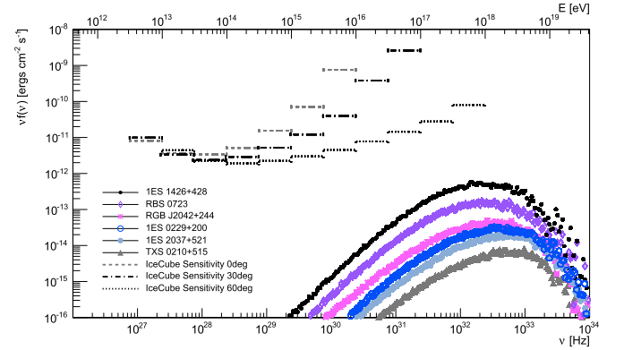
Figure 11. The maximum neutrino flux expected from the proton synchrotron model applied to six EHBs. The IceCube sensitivity (IceCube Collaboration et al. 2019) for three different declinations is also represented.
