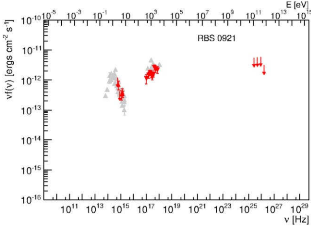
Figure 10. SED of RBS 0921. The unique source of the sample is still undetected at gamma-rays.
